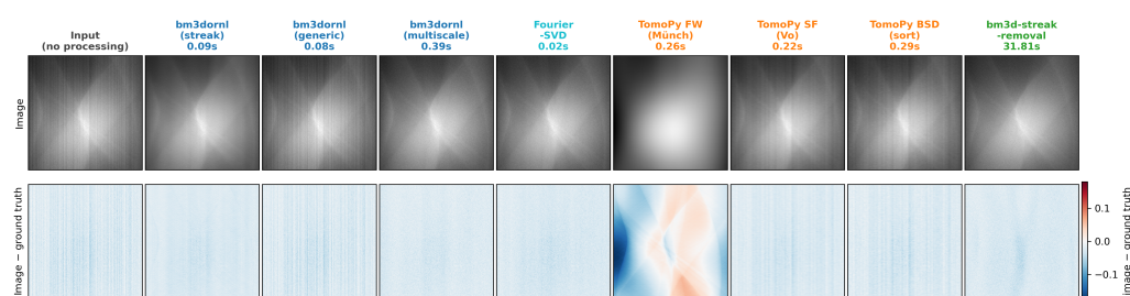
Figure 2: Method comparison on the crop marked in Figure 1 . Top row: the unprocessed input, then the result of each method with its processing time. Bottom row: difference from the ground truth (image minus ground truth) on one zero-centered red–blue scale shared by all columns; red marks pixels above the ground truth, blue marks pixels below it, and white marks agreement, so a perfect result would leave a uniformly white difference image. The faint blue tint common to every column, including the input, comes from the benchmark's rescaling of the input to [0, 1] and is not a sign of removal; the artifacts are the vertical stripes, complete in the input column and remaining in the others to the extent each method left them. Data from Linux x86_64.
