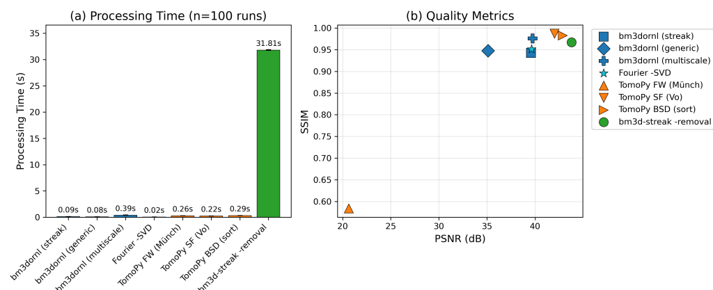
Figure 3: Performance metrics (Linux x86 64 , n=100 runs). (a) Processing time comparison on linear scale, showing Fourier-SVD's 1900× speedup and standard BM3DORN's 340× speedup over bm3d-streak-removal. (b) Quality metrics, peak signal-to-noise ratio (PSNR) against structural similarity index measure (SSIM), showing trade-offs between methods. BM3DORN variants (blue/cyan), TomoPy (orange), bm3d-streak-removal (green).
