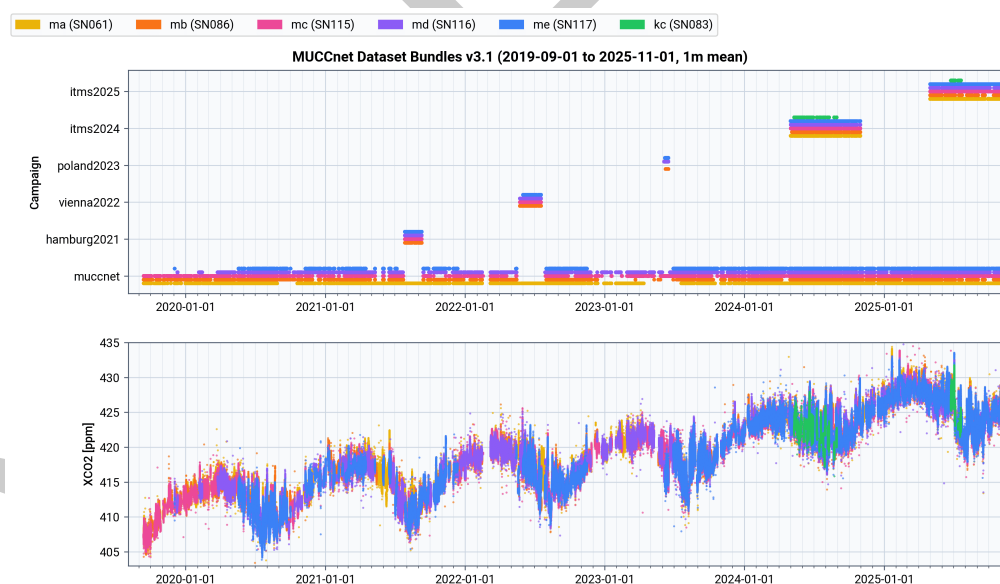
Figure 2: XCO 2 retrievals from 2019-09-01 to 2025-11-01 for the five MUCCnet instruments (ma to me) and the KIT traveling reference (kc). The upper panel shows when each EM27/SUN instrument has been recording as part of which measurement campaign. The lower panel shows the corresponding one-minute mean XCO 2 retrieval results.
