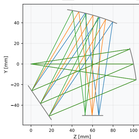
Figure 2: A model of a folded Czerny-Turner spectrometer. Different colored rays represent different wavelengths.
