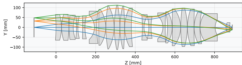
Figure 1: An example of a complex, multi-element UV photolithography lens modeled and rendered in Optiland. Based on U.S. Patent #5,831,776. Different colored rays represent different fields.
