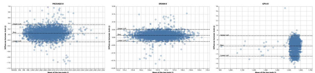
Figure 3: Bland-Altman analysis of energy measurements (J) across RAPL domains (DRAM, PACKAGE) comparing ' perf ' and Joule Profiler, and GPU comparing Alumet and Joule Profiler.
