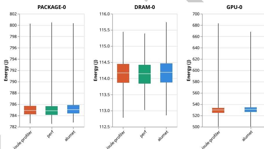
Figure 4: Energy distribution (J) across RAPL domains (DRAM, PACKAGE) and GPU comparing perf, Alumet, and Joule Profiler.
