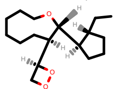
PhEthOH_1625.pdb
