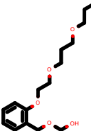
PhEthOH_2748.pdb
