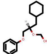
PhEthOH_4248.pdb
