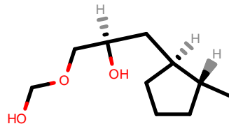
PhEthOH_318.pdb
