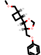
PhEthOH_1982.pdb
