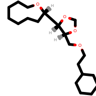
PhEthOH_4455.pdb
