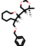
PhEthOH_393.pdb
