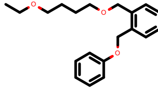
PhEthOH_2230.pdb
