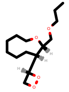
PhEthOH_1419.pdb
