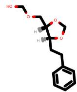
PhEthOH_950.pdb
