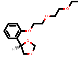
PhEthOH_2302.pdb
