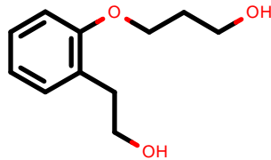
PhEthOH_478.pdb
