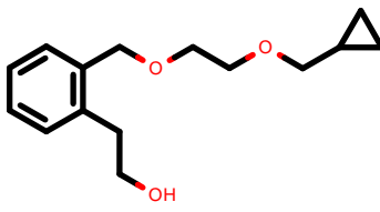
PhEthOH_3125.pdb
