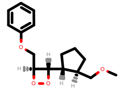
PhEthOH_2019.pdb
