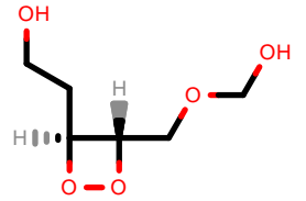
PhEthOH_519.pdb
