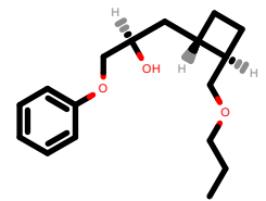
PhEthOH_2815.pdb
