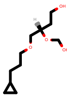
PhEthOH_3210.pdb
