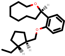
PhEthOH_1632.pdb
