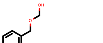
PhEthOH_2581.pdb
