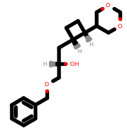
PhEthOH_4967.pdb
