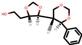
PhEthOH_1276.pdb
