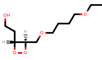
PhEthOH_2329.pdb
