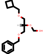
PhEthOH_3540.pdb
