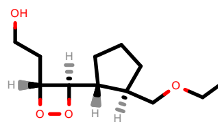
PhEthOH_2451.pdb
