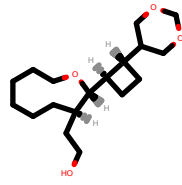
PhEthOH_4977.pdb
