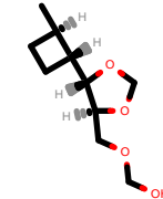
PhEthOH_274.pdb
