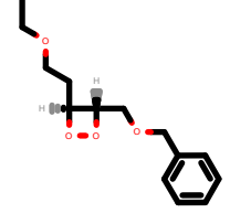
PhEthOH_2155.pdb
