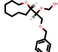
PhEthOH_1005.pdb
