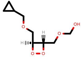
PhEthOH_3133.pdb
