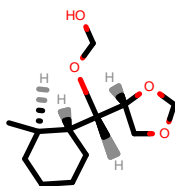
PhEthOH_373.pdb
