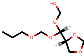
PhEthOH_2641.pdb
