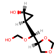
PhEthOH_667.pdb
