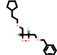
PhEthOH_3999.pdb
