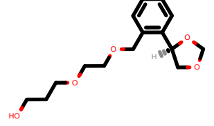
PhEthOH_623.pdb
