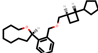
PhEthOH_4157.pdb
