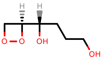
PhEthOH_488.pdb
