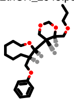
PhEthOH_2949.pdb
