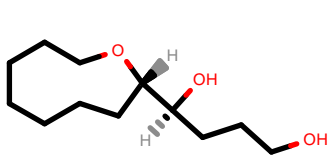
PhEthOH_500.pdb
