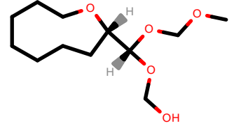
PhEthOH_1807.pdb
