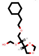
PhEthOH_4447.pdb
