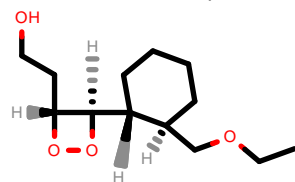
PhEthOH_2493.pdb
