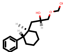
PhEthOH_1238.pdb
