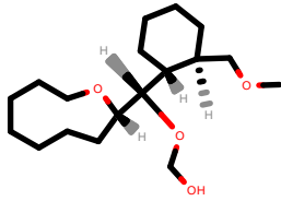
PhEthOH_2101.pdb
