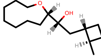
PhEthOH_294.pdb
