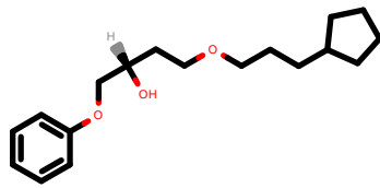
PhEthOH_4033.pdb
