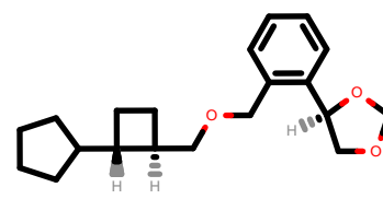
PhEthOH_4151.pdb
