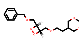
PhEthOH_4839.pdb
