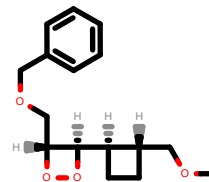
PhEthOH_1983.pdb
