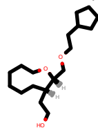
PhEthOH_4007.pdb
