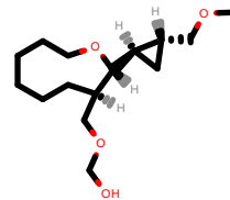
PhEthOH_1959.pdb
