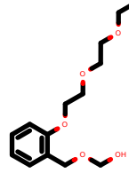
PhEthOH_2290.pdb
