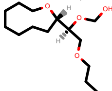
PhEthOH_165.pdb
