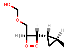
PhEthOH_235.pdb
