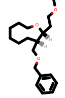
PhEthOH_1737.pdb
