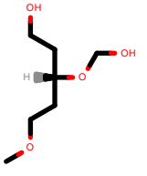
PhEthOH_1740.pdb
