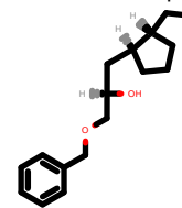
PhEthOH_1607.pdb
