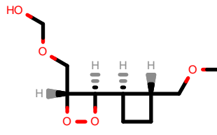
PhEthOH_1999.pdb
