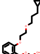
PhEthOH_3210.pdb
