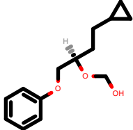
PhEthOH_3068.pdb
