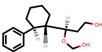
PhEthOH_1232.pdb
