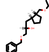
PhEthOH_2447.pdb
