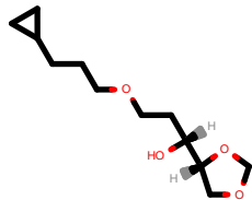
PhEthOH_3228.pdb
