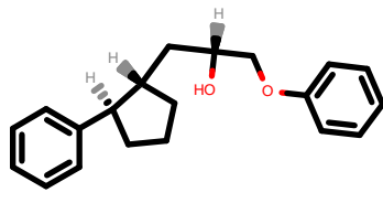
PhEthOH_1181.pdb
