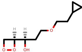
PhEthOH_3180.pdb
