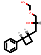
PhEthOH_1158.pdb
