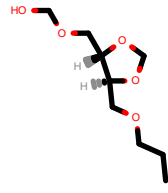
PhEthOH_152.pdb
