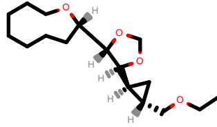
PhEthOH_2397.pdb
