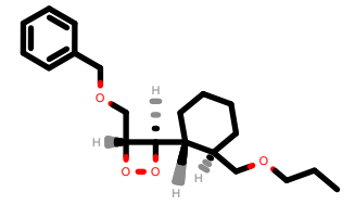
PhEthOH_2911.pdb
