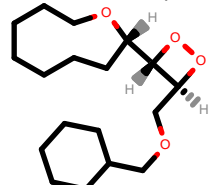
PhEthOH_4408.pdb
