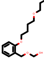
PhEthOH_2668.pdb
