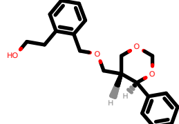
PhEthOH_1277.pdb
