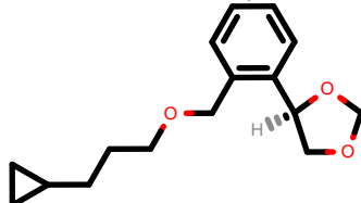
PhEthOH_3101.pdb
