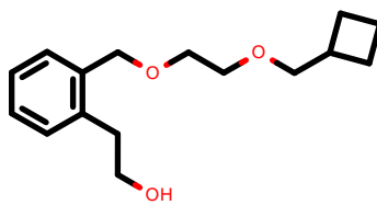
PhEthOH_3545.pdb
