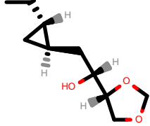
PhEthOH_1544.pdb
