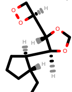
PhEthOH_1624.pdb
