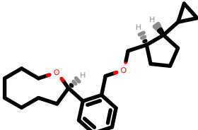
PhEthOH_3317.pdb
