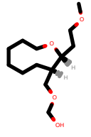
PhEthOH_1749.pdb
