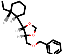
PhEthOH_1648.pdb
