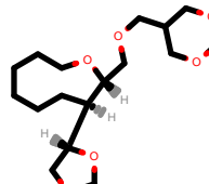
PhEthOH_4823.pdb
