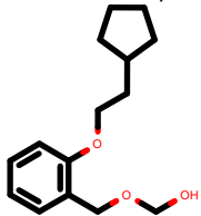
PhEthOH_3844.pdb
