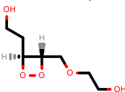
PhEthOH_561.pdb
