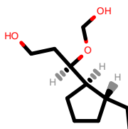
PhEthOH_1610.pdb
