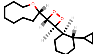
PhEthOH_3358.pdb
