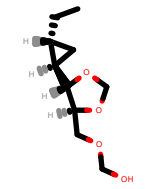
PhEthOH_1534.pdb
