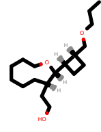
PhEthOH_2835.pdb
