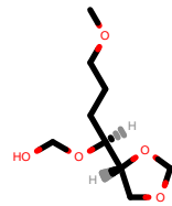
PhEthOH_1843.pdb
