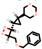
PhEthOH_4927.pdb
