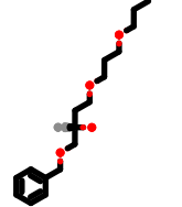
PhEthOH_2741.pdb
