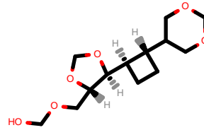
PhEthOH_4982.pdb
