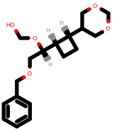
PhEthOH_4968.pdb
