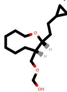
PhEthOH_3093.pdb
