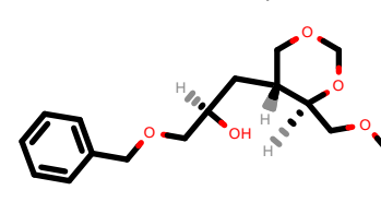
PhEthOH_2111.pdb
