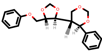
PhEthOH_1268.pdb
