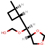
PhEthOH_285.pdb
