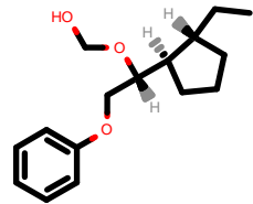
PhEthOH_1598.pdb
