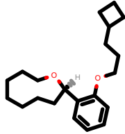
PhEthOH_3526.pdb
