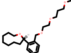
PhEthOH_1885.pdb
