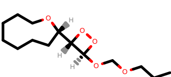
PhEthOH_2644.pdb
