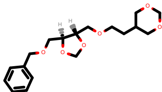
PhEthOH_4844.pdb
