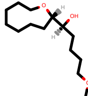
PhEthOH_1848.pdb
