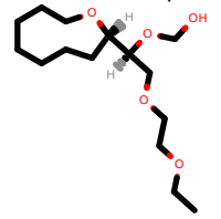
PhEthOH_2311.pdb
