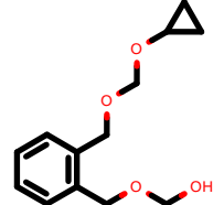
PhEthOH_3047.pdb
