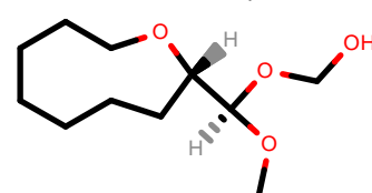
PhEthOH_39.pdb
