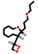
PhEthOH_2679.pdb
