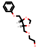
PhEthOH_554.pdb
