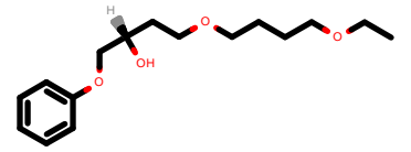
PhEthOH_2311.pdb
