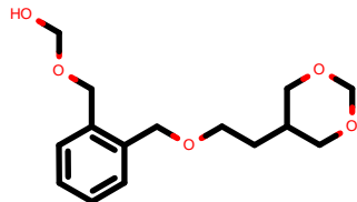
PhEthOH_4685.pdb
