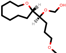
PhEthOH_1849.pdb
