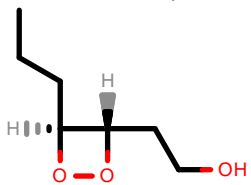
PhEthOH_57.pdb
