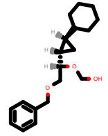
PhEthOH_4506.pdb
