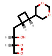
PhEthOH_4986.pdb
