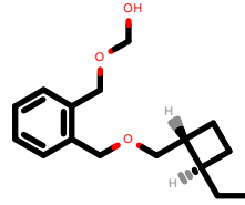
PhEthOH_1577.pdb
