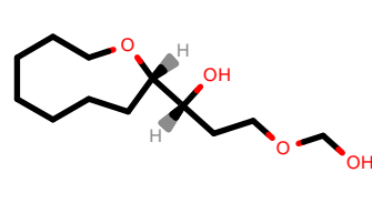
PhEthOH_542.pdb
