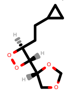
PhEthOH_3100.pdb
