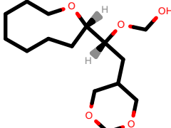
PhEthOH_4701.pdb
