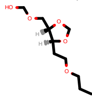
PhEthOH_2588.pdb
