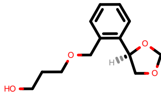
PhEthOH_493.pdb
