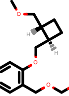
PhEthOH_1996.pdb
