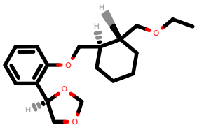
PhEthOH_2512.pdb
