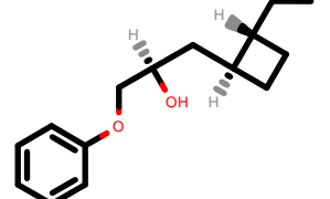
PhEthOH_1555.pdb
