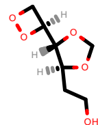
PhEthOH_490.pdb
