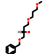
PhEthOH_1855.pdb
