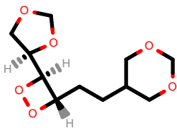
PhEthOH_4780.pdb
