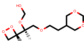
PhEthOH_4857.pdb
