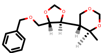
PhEthOH_388.pdb
