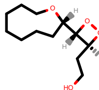
PhEthOH_502.pdb
