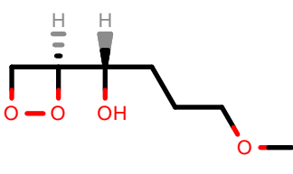
PhEthOH_1752.pdb
