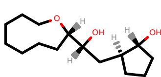
PhEthOH_752.pdb
