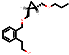
PhEthOH_2785.pdb
