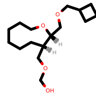
PhEthOH_3551.pdb
