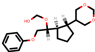
PhEthOH_5004.pdb
