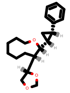
PhEthOH_1131.pdb
