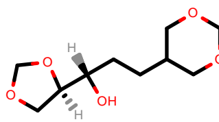
PhEthOH_4694.pdb
