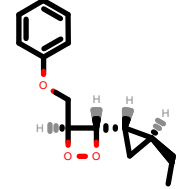
PhEthOH_1519.pdb
