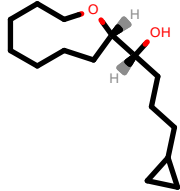
PhEthOH_3108.pdb
