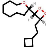
PhEthOH_3530.pdb
