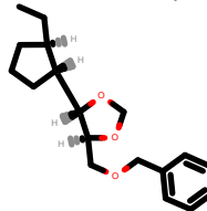
PhEthOH_1610.pdb
