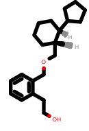
PhEthOH_4175.pdb
