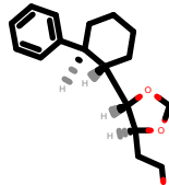
PhEthOH_1234.pdb
