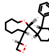
PhEthOH_1247.pdb
