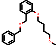
PhEthOH_1816.pdb
