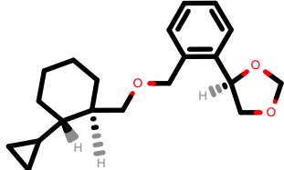
PhEthOH_3349.pdb
