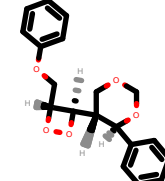
PhEthOH_1267.pdb
