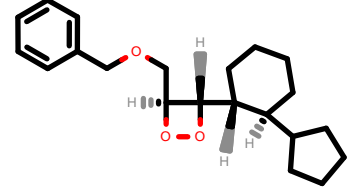
PhEthOH_4171.pdb
