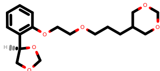
PhEthOH_4906.pdb
