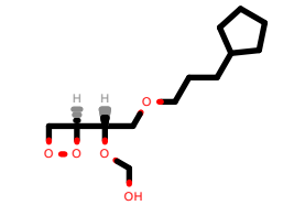
PhEthOH_4063.pdb
