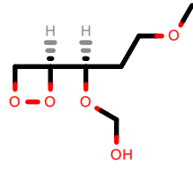
PhEthOH_1753.pdb
