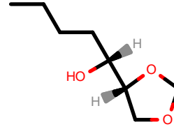
PhEthOH_1338.pdb
