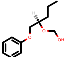
PhEthOH_44.pdb
