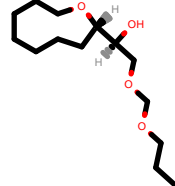
PhEthOH_2646.pdb
