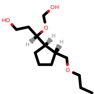
PhEthOH_2870.pdb
