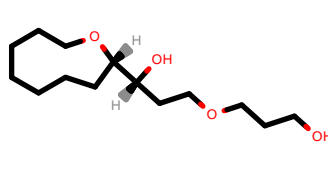
PhEthOH_630.pdb
