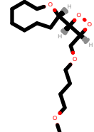
PhEthOH_1934.pdb
