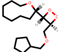
PhEthOH_3988.pdb
