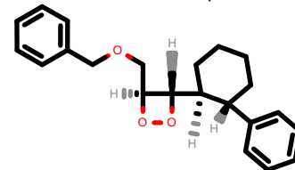
PhEthOH_1231.pdb
