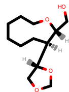
PhEthOH_455.pdb
