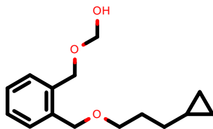
PhEthOH_3089.pdb
