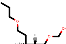
PhEthOH_2583.pdb
