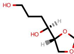
PhEthOH_494.pdb
