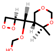
PhEthOH_405.pdb
