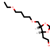
PhEthOH_2330.pdb
