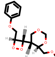
PhEthOH_2103.pdb
