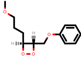
PhEthOH_1813.pdb
