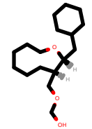
PhEthOH_4269.pdb
