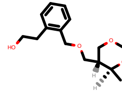
PhEthOH_395.pdb
