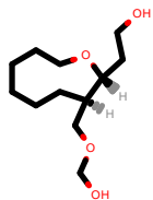
PhEthOH_485.pdb
