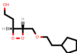
PhEthOH_4005.pdb
