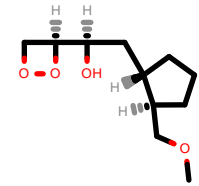
PhEthOH_2046.pdb
