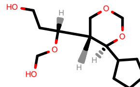
PhEthOH_4214.pdb
