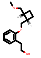
PhEthOH_1990.pdb
