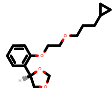
PhEthOH_3226.pdb
