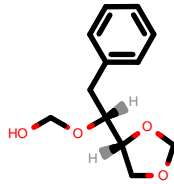
PhEthOH_877.pdb
