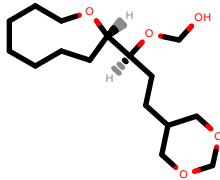
PhEthOH_4785.pdb
