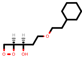
PhEthOH_4440.pdb
