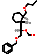
PhEthOH_2910.pdb
