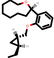
PhEthOH_1552.pdb
