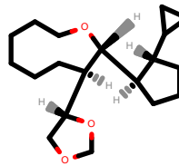
PhEthOH_3315.pdb
