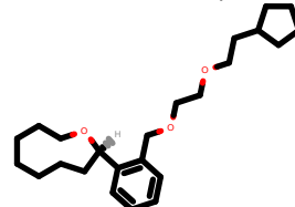
PhEthOH_4031.pdb
