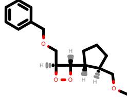
PhEthOH_2029.pdb
