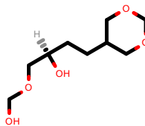
PhEthOH_4686.pdb
