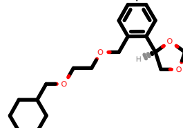
PhEthOH_4399.pdb
