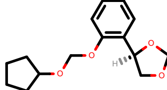
PhEthOH_3898.pdb
