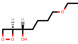
PhEthOH_2256.pdb
