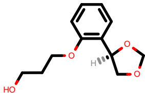
PhEthOH_492.pdb
