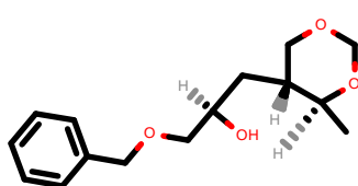
PhEthOH_385.pdb
