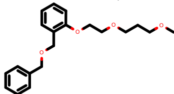
PhEthOH_1854.pdb
