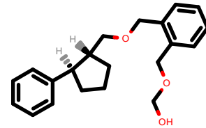
PhEthOH_1195.pdb
