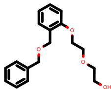
PhEthOH_552.pdb
