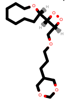
PhEthOH_4916.pdb
