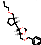
PhEthOH_2866.pdb
