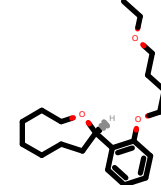
PhEthOH_2266.pdb
