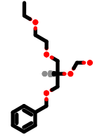
PhEthOH_2280.pdb
