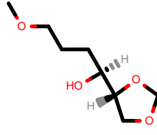
PhEthOH_1758.pdb
