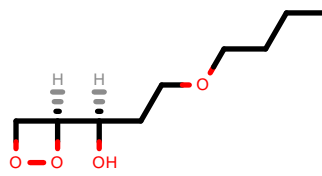
PhEthOH_194.pdb
