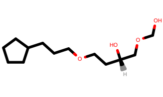
PhEthOH_4056.pdb
