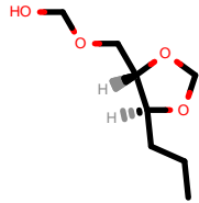
PhEthOH_1328.pdb
