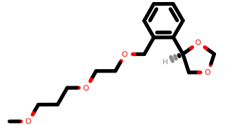
PhEthOH_1879.pdb
