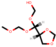
PhEthOH_1801.pdb
