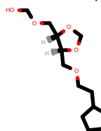
PhEthOH_4016.pdb
