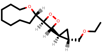
PhEthOH_2396.pdb
