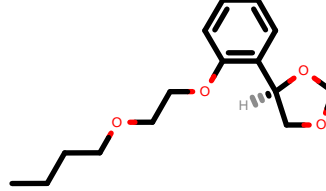
PhEthOH_202.pdb
