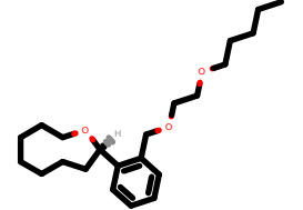
PhEthOH_1511.pdb
