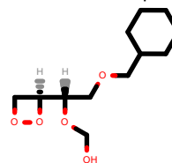
PhEthOH_4395.pdb
