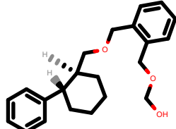
PhEthOH_1237.pdb
