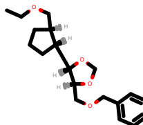
PhEthOH_2450.pdb
