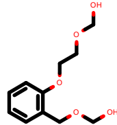
PhEthOH_522.pdb
