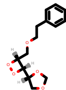
PhEthOH_1046.pdb
