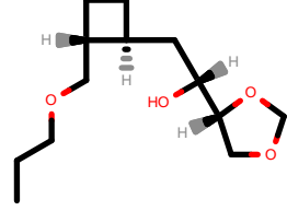
PhEthOH_2846.pdb
