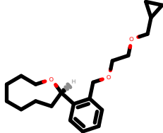
PhEthOH_3149.pdb
