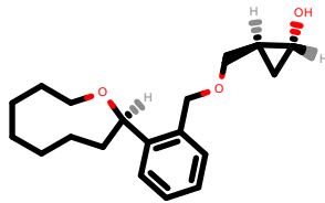
PhEthOH_671.pdb
