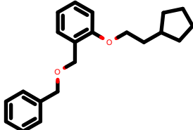
PhEthOH_3832.pdb
