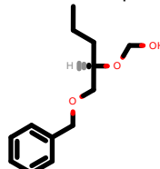
PhEthOH_50.pdb
