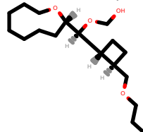
PhEthOH_2857.pdb
