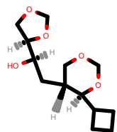
PhEthOH_3816.pdb
