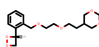
PhEthOH_4855.pdb
