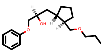
PhEthOH_2861.pdb
