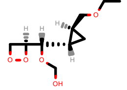
PhEthOH_2383.pdb
