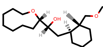
PhEthOH_2096.pdb
