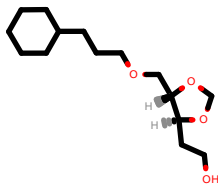
PhEthOH_4472.pdb
