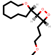
PhEthOH_1850.pdb
