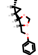
PhEthOH_218.pdb
