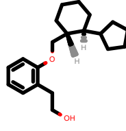
PhEthOH_4174.pdb
