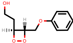
PhEthOH_469.pdb
