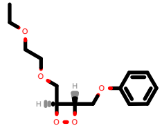
PhEthOH_2271.pdb
