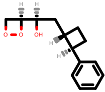
PhEthOH_1164.pdb
