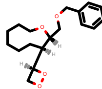
PhEthOH_999.pdb
