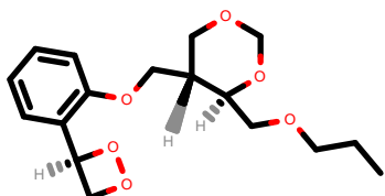
PhEthOH_2964.pdb
