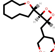
PhEthOH_4702.pdb
