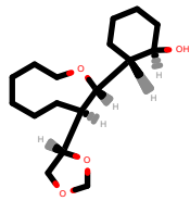
PhEthOH_791.pdb
