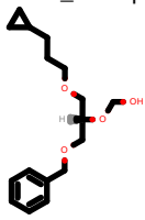
PhEthOH_3204.pdb
