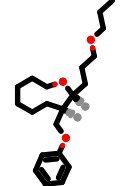
PhEthOH_2655.pdb
