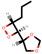
PhEthOH_1340.pdb
