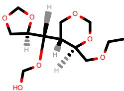
PhEthOH_2553.pdb
