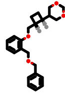
PhEthOH_4966.pdb
