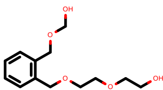
PhEthOH_565.pdb
