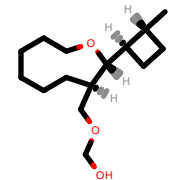
PhEthOH_275.pdb
