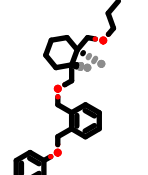
PhEthOH_2898.pdb
