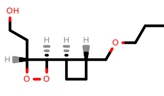
PhEthOH_2833.pdb
