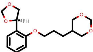
PhEthOH_4776.pdb
