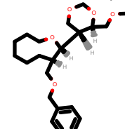
PhEthOH_2111.pdb
