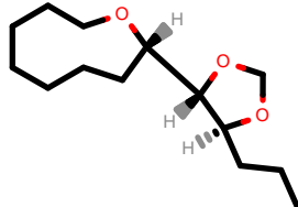
PhEthOH_83.pdb
