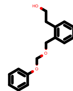
PhEthOH_895.pdb
