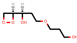
PhEthOH_618.pdb
