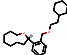
PhEthOH_4283.pdb
