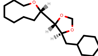
PhEthOH_4287.pdb
