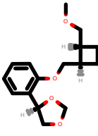
PhEthOH_2008.pdb
