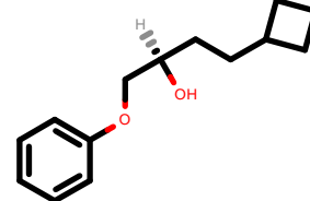
PhEthOH_3407.pdb
