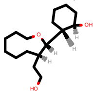
PhEthOH_773.pdb
