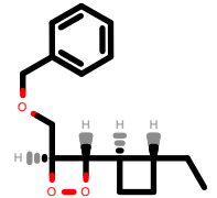
PhEthOH_1567.pdb
