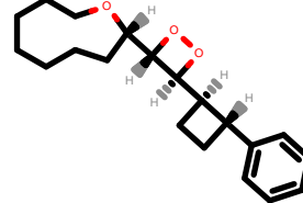
PhEthOH_1178.pdb
