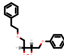
PhEthOH_1011.pdb
