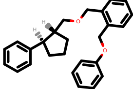
PhEthOH_1180.pdb
