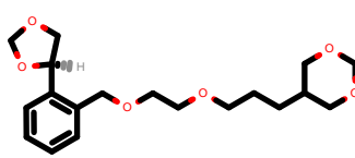
PhEthOH_4907.pdb
