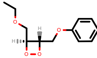
PhEthOH_87.pdb
