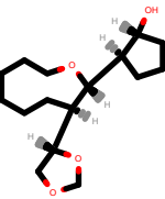
PhEthOH_753.pdb
