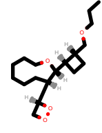
PhEthOH_2847.pdb
