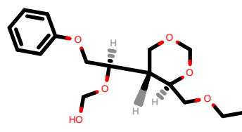
PhEthOH_2526.pdb
