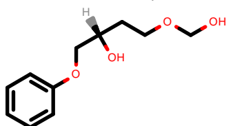
PhEthOH_505.pdb
