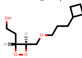
PhEthOH_3631.pdb
