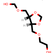
PhEthOH_572.pdb
