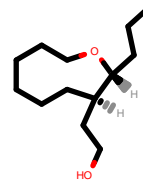
PhEthOH_1319.pdb
