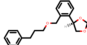
PhEthOH_959.pdb
