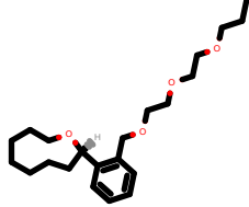
PhEthOH_2729.pdb
