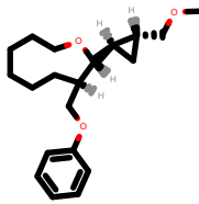
PhEthOH_1941.pdb
