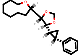
PhEthOH_1137.pdb
