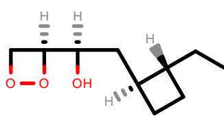
PhEthOH_1584.pdb
