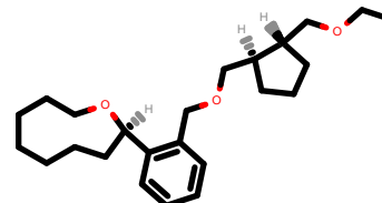
PhEthOH_2473.pdb
