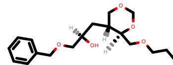
PhEthOH_2947.pdb
