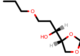
PhEthOH_1422.pdb
