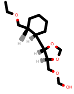
PhEthOH_2504.pdb
