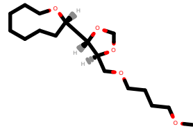
PhEthOH_1935.pdb
