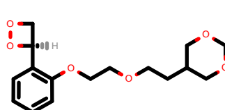
PhEthOH_4854.pdb
