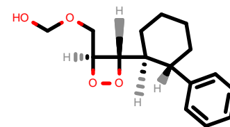
PhEthOH_1239.pdb
