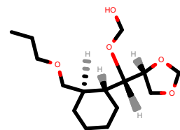
PhEthOH_2935.pdb
