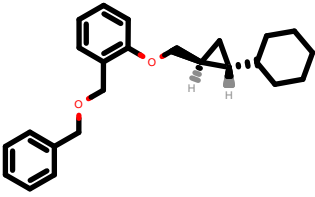
PhEthOH_4504.pdb
