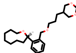
PhEthOH_4783.pdb
