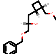
PhEthOH_1981.pdb
