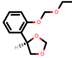
PhEthOH_1374.pdb
