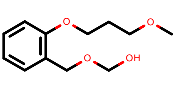
PhEthOH_1744.pdb
