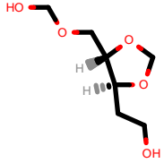
PhEthOH_520.pdb
