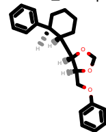
PhEthOH_1226.pdb
