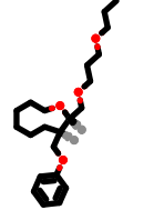
PhEthOH_2739.pdb
