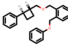
PhEthOH_1138.pdb
