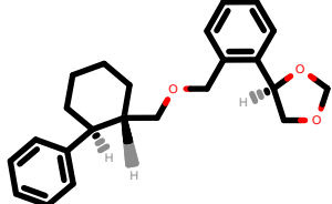
PhEthOH_1253.pdb
