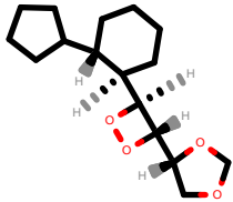
PhEthOH_4196.pdb
