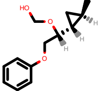
PhEthOH_216.pdb
