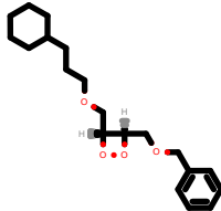
PhEthOH_4465.pdb
