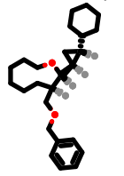
PhEthOH_4509.pdb
