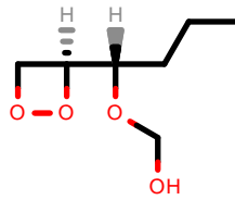
PhEthOH_1333.pdb
