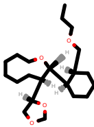
PhEthOH_2937.pdb
