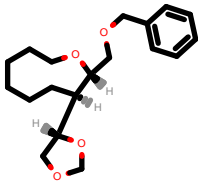
PhEthOH_1005.pdb
