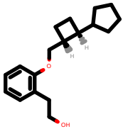
PhEthOH_4132.pdb
