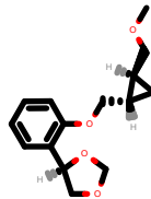
PhEthOH_1966.pdb
