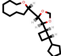
PhEthOH_4157.pdb
