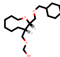
PhEthOH_4391.pdb
