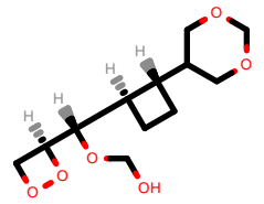
PhEthOH_4987.pdb
