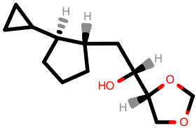
PhEthOH_3312.pdb
