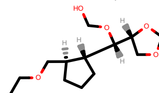
PhEthOH_2469.pdb
