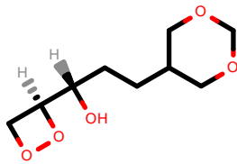
PhEthOH_4692.pdb
