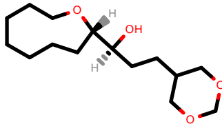
PhEthOH_4700.pdb
