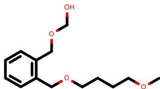
PhEthOH_1825.pdb
