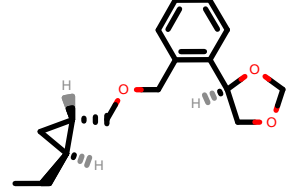
PhEthOH_1547.pdb
