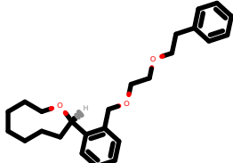
PhEthOH_1049.pdb
