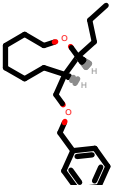
PhEthOH_53.pdb
