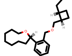
PhEthOH_1595.pdb
