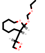
PhEthOH_2217.pdb
