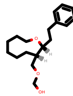
PhEthOH_951.pdb
