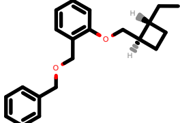
PhEthOH_1564.pdb
