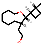
PhEthOH_269.pdb
