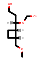
PhEthOH_1992.pdb
