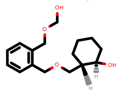
PhEthOH_775.pdb
