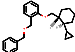
PhEthOH_3324.pdb
