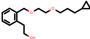
PhEthOH_3209.pdb
