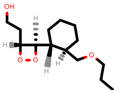
PhEthOH_2917.pdb
