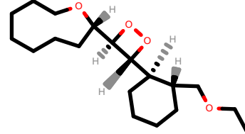
PhEthOH_2522.pdb
