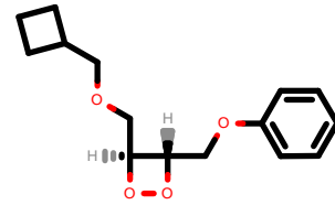
PhEthOH_3535.pdb
