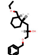
PhEthOH_2485.pdb
