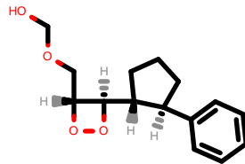
PhEthOH_1201.pdb
