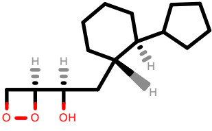
PhEthOH_4188.pdb
