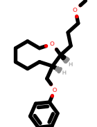
PhEthOH_1815.pdb
