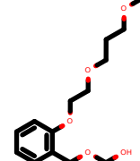
PhEthOH_1866.pdb
