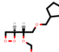
PhEthOH_3975.pdb
