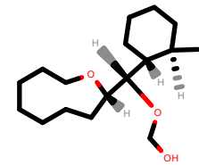
PhEthOH_379.pdb
