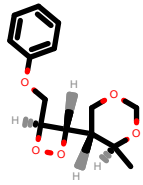
PhEthOH_381.pdb
