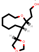
PhEthOH_497.pdb
