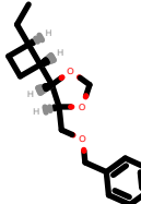
PhEthOH_1564.pdb
