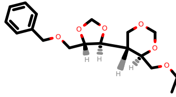
PhEthOH_2534.pdb
