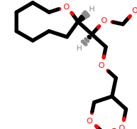
PhEthOH_4831.pdb
