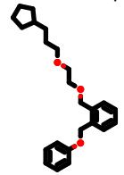
PhEthOH_4036.pdb
