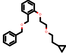
PhEthOH_3160.pdb
