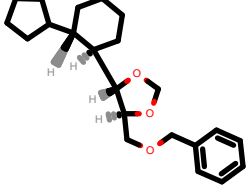
PhEthOH_4172.pdb
