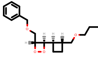
PhEthOH_2827.pdb
