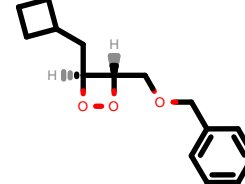
PhEthOH_3415.pdb
