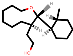
PhEthOH_357.pdb
