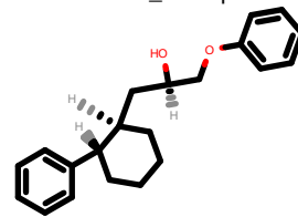
PhEthOH_1223.pdb
