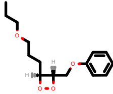
PhEthOH_2653.pdb
