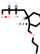
PhEthOH_2928.pdb
