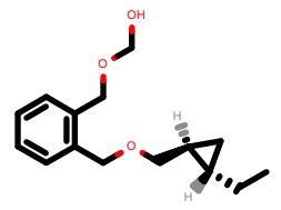
PhEthOH_1535.pdb
