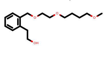
PhEthOH_1907.pdb
