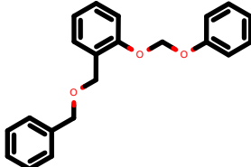
PhEthOH_892.pdb
