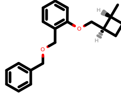
PhEthOH_262.pdb
