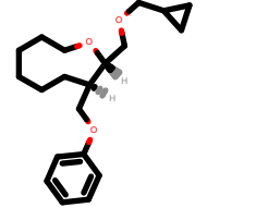
PhEthOH_3117.pdb
