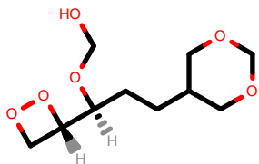
PhEthOH_4773.pdb
