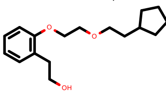
PhEthOH_4006.pdb
