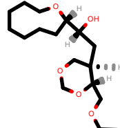
PhEthOH_2558.pdb
