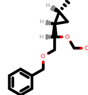
PhEthOH_222.pdb
