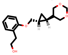
PhEthOH_4926.pdb
