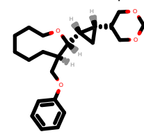
PhEthOH_4923.pdb
