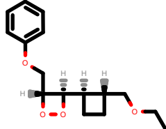
PhEthOH_2397.pdb
