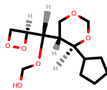
PhEthOH_4231.pdb
