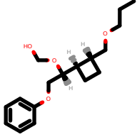
PhEthOH_2820.pdb
