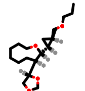
PhEthOH_2807.pdb
