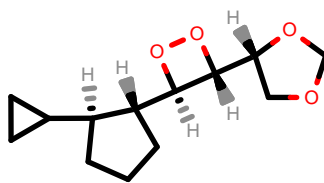
PhEthOH_3314.pdb
