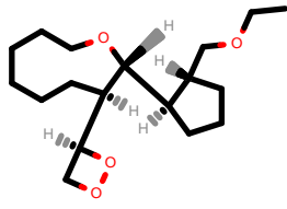
PhEthOH_2469.pdb
