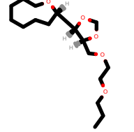
PhEthOH_2733.pdb
