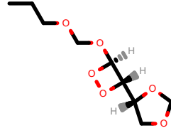
PhEthOH_2642.pdb
