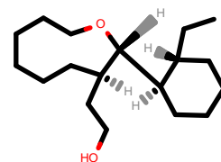
PhEthOH_1655.pdb
