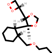
PhEthOH_2930.pdb
