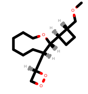
PhEthOH_2007.pdb
