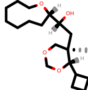
PhEthOH_3822.pdb
