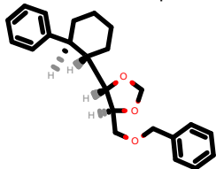
PhEthOH_1232.pdb
