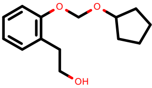
PhEthOH_3880.pdb
