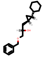
PhEthOH_4505.pdb
