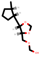
PhEthOH_316.pdb
