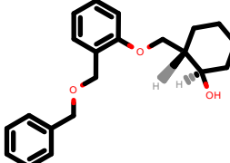
PhEthOH_766.pdb
