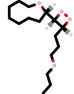
PhEthOH_2686.pdb
