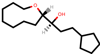
PhEthOH_3864.pdb
