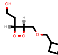
PhEthOH_3547.pdb
