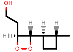
PhEthOH_267.pdb
