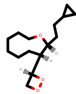
PhEthOH_3099.pdb
