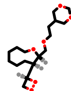
PhEthOH_4863.pdb
