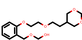
PhEthOH_4848.pdb
