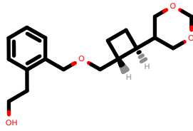
PhEthOH_4973.pdb
