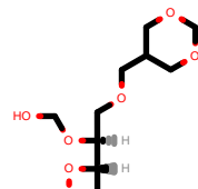
PhEthOH_4815.pdb
