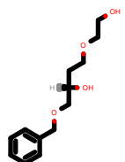
PhEthOH_553.pdb
