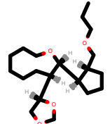
PhEthOH_2891.pdb
