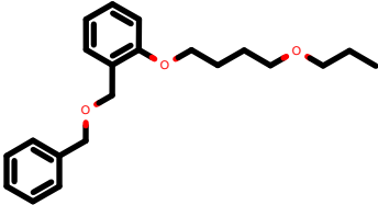
PhEthOH_2652.pdb
