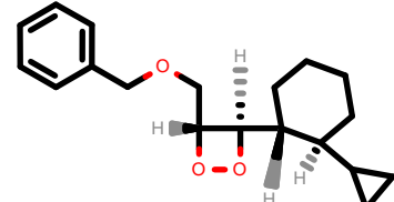
PhEthOH_3327.pdb
