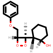
PhEthOH_759.pdb
