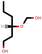
PhEthOH_1316.pdb
