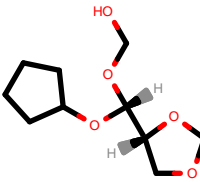
PhEthOH_3901.pdb
