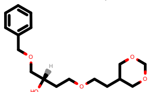
PhEthOH_4837.pdb
