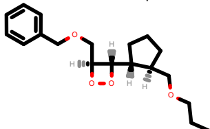
PhEthOH_2865.pdb
