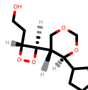
PhEthOH_4215.pdb
