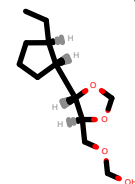
PhEthOH_1618.pdb
