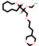
PhEthOH_4915.pdb
