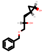
PhEthOH_637.pdb
