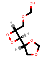
PhEthOH_542.pdb
