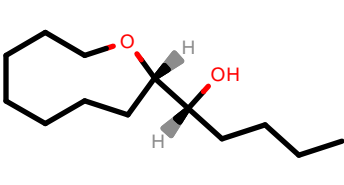
PhEthOH_1340.pdb
