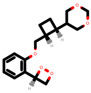
PhEthOH_4984.pdb
