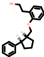
PhEthOH_1188.pdb
