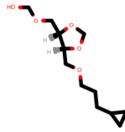
PhEthOH_3218.pdb
