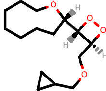
PhEthOH_3152.pdb
