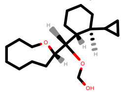
PhEthOH_3357.pdb
