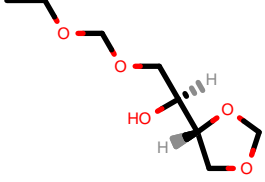
PhEthOH_2220.pdb
