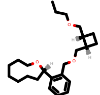
PhEthOH_2855.pdb
