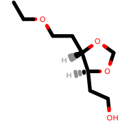
PhEthOH_2162.pdb
