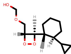
PhEthOH_3339.pdb
