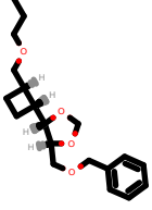
PhEthOH_2828.pdb
