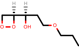
PhEthOH_156.pdb
