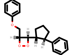
PhEthOH_1183.pdb
