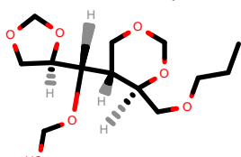
PhEthOH_2973.pdb
