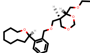
PhEthOH_2557.pdb
