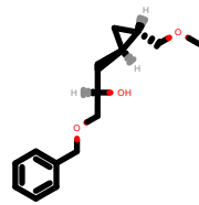
PhEthOH_1943.pdb
