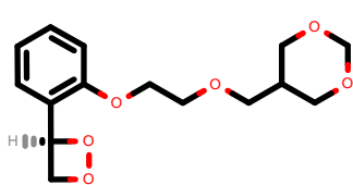
PhEthOH_4812.pdb
