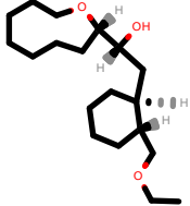
PhEthOH_2520.pdb
