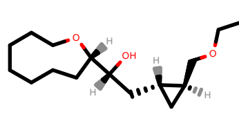
PhEthOH_2394.pdb
