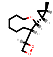
PhEthOH_243.pdb
