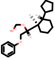
PhEthOH_4164.pdb
