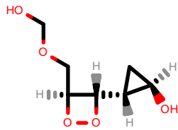
PhEthOH_655.pdb
