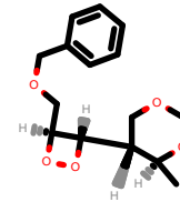
PhEthOH_391.pdb
