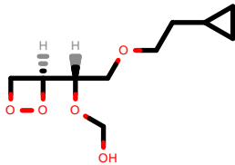
PhEthOH_3181.pdb
