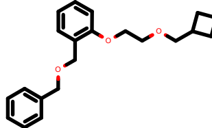
PhEthOH_3538.pdb
