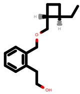
PhEthOH_1567.pdb
