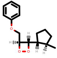
PhEthOH_301.pdb
