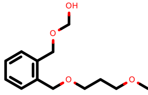
PhEthOH_1745.pdb
