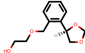
PhEthOH_451.pdb
