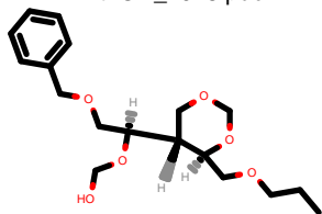
PhEthOH_2952.pdb
