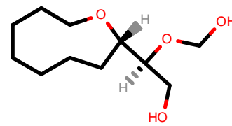
PhEthOH_463.pdb
