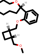
PhEthOH_2014.pdb
