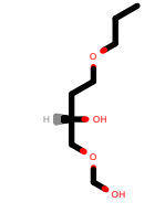
PhEthOH_150.pdb
