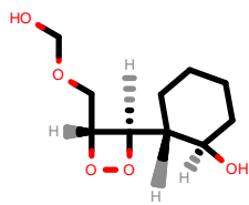
PhEthOH_777.pdb
