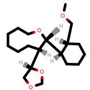
PhEthOH_2097.pdb
