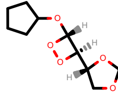
PhEthOH_3902.pdb
