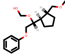
PhEthOH_2022.pdb
