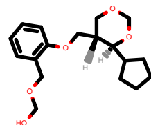
PhEthOH_4222.pdb
