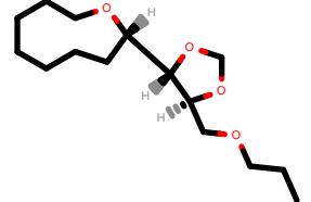
PhEthOH_1431.pdb
