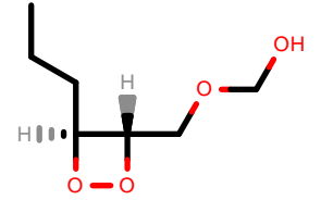
PhEthOH_1327.pdb
