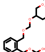
PhEthOH_4723.pdb
