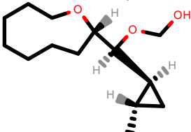
PhEthOH_253.pdb
