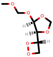
PhEthOH_1792.pdb
