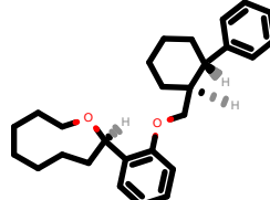
PhEthOH_1254.pdb
