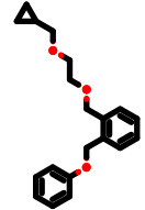
PhEthOH_3112.pdb
