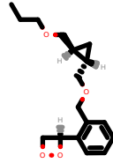
PhEthOH_2801.pdb
