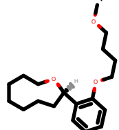
PhEthOH_1846.pdb
