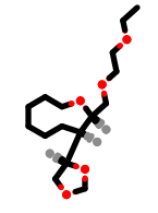
PhEthOH_2303.pdb
