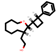
PhEthOH_1151.pdb
