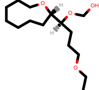
PhEthOH_2269.pdb
