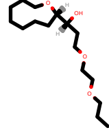
PhEthOH_2730.pdb
