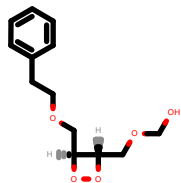
PhEthOH_1033.pdb
