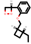
PhEthOH_1582.pdb
