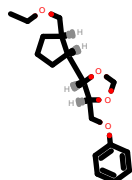
PhEthOH_2444.pdb
