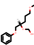
PhEthOH_2232.pdb
