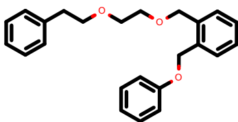
PhEthOH_1008.pdb
