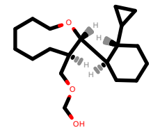
PhEthOH_3341.pdb
