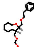
PhEthOH_1035.pdb
