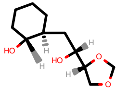
PhEthOH_788.pdb
