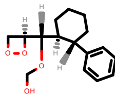
PhEthOH_1245.pdb
