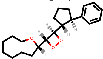
PhEthOH_1220.pdb
