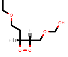
PhEthOH_2167.pdb
