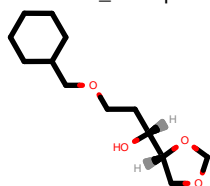
PhEthOH_4400.pdb
