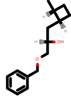
PhEthOH_263.pdb
