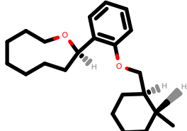
PhEthOH_376.pdb
