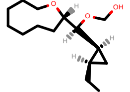
PhEthOH_1555.pdb
