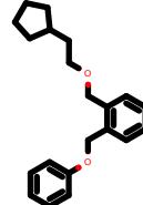
PhEthOH_3826.pdb
