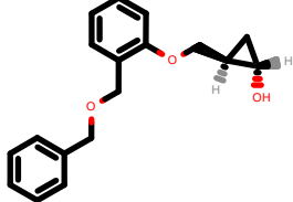
PhEthOH_636.pdb
