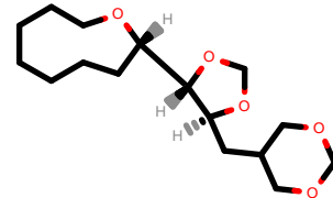
PhEthOH_4703.pdb
