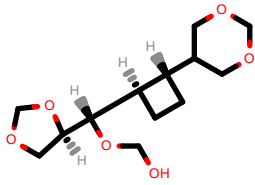
PhEthOH_4989.pdb
