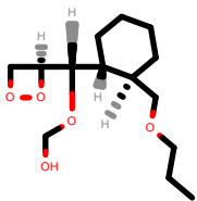
PhEthOH_2929.pdb
