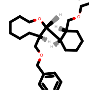
PhEthOH_2489.pdb
