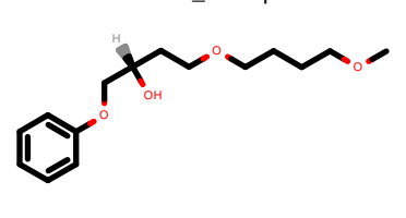
PhEthOH_1895.pdb
