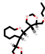
PhEthOH_2975.pdb
