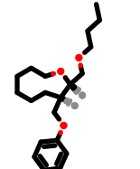
PhEthOH_177.pdb
