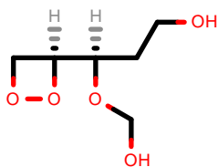
PhEthOH_489.pdb
