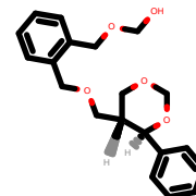
PhEthOH_1279.pdb
