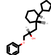
PhEthOH_4159.pdb
