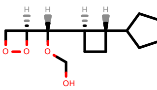
PhEthOH_4147.pdb
