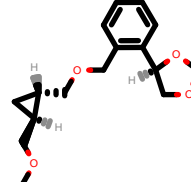
PhEthOH_1967.pdb
