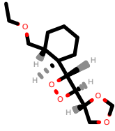
PhEthOH_2516.pdb
