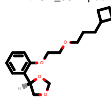
PhEthOH_3646.pdb
