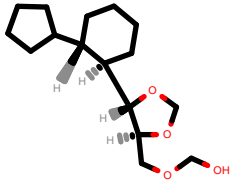
PhEthOH_4184.pdb
