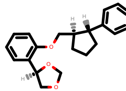
PhEthOH_1206.pdb
