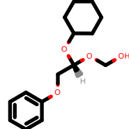
PhEthOH_4286.pdb
