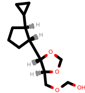
PhEthOH_3302.pdb
