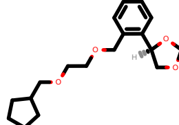
PhEthOH_3983.pdb
