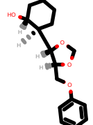
PhEthOH_764.pdb
