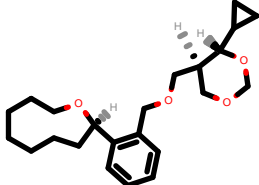
PhEthOH_3401.pdb
