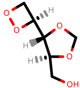
PhEthOH_448.pdb
