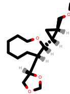
PhEthOH_1971.pdb
