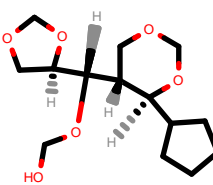
PhEthOH_4233.pdb
