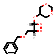
PhEthOH_4713.pdb
