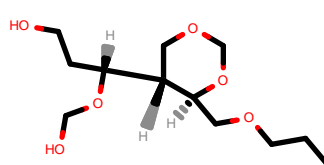
PhEthOH_2954.pdb
