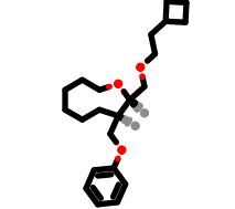
PhEthOH_3579.pdb
