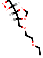
PhEthOH_2300.pdb
