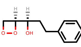
PhEthOH_866.pdb
