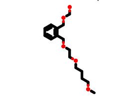
PhEthOH_1913.pdb
