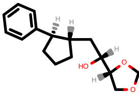
PhEthOH_1212.pdb
