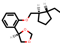
PhEthOH_1626.pdb
