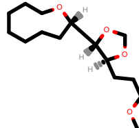
PhEthOH_1851.pdb
