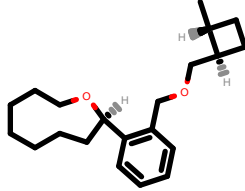
PhEthOH_293.pdb
