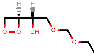
PhEthOH_2214.pdb
