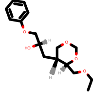
PhEthOH_2525.pdb
