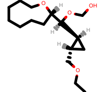
PhEthOH_2395.pdb
