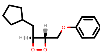
PhEthOH_3829.pdb
