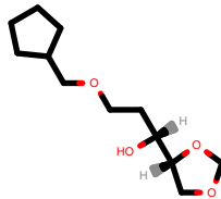
PhEthOH_3984.pdb
