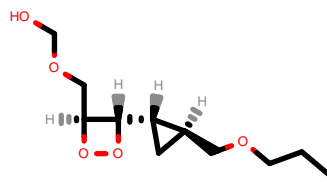
PhEthOH_2793.pdb
