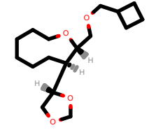
PhEthOH_3567.pdb
