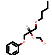
PhEthOH_170.pdb
