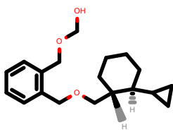
PhEthOH_3337.pdb
