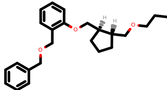
PhEthOH_2866.pdb
