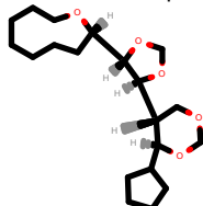
PhEthOH_4245.pdb
