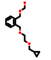
PhEthOH_3131.pdb
