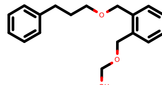
PhEthOH_943.pdb
