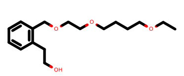
PhEthOH_2323.pdb
