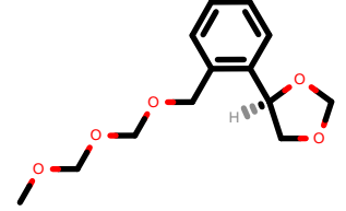
PhEthOH_1799.pdb
