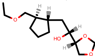
PhEthOH_2468.pdb
