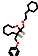
PhEthOH_4415.pdb
