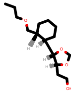
PhEthOH_2918.pdb
