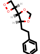
PhEthOH_956.pdb
