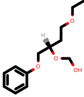
PhEthOH_2148.pdb
