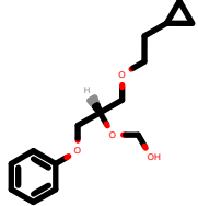
PhEthOH_3156.pdb
