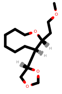
PhEthOH_1757.pdb
