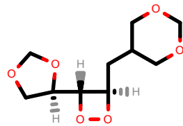
PhEthOH_4700.pdb
