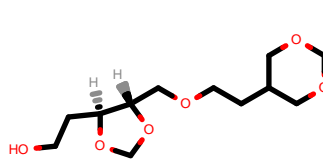
PhEthOH_4846.pdb
