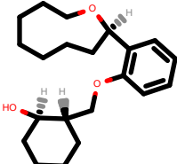
PhEthOH_792.pdb
