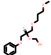
PhEthOH_1854.pdb
