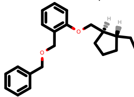
PhEthOH_1606.pdb
