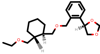
PhEthOH_2513.pdb
