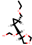
PhEthOH_2389.pdb
