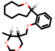
PhEthOH_414.pdb
