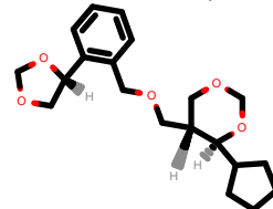
PhEthOH_4235.pdb
