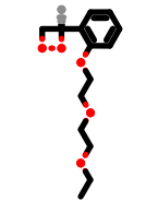
PhEthOH_2296.pdb
