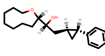
PhEthOH_1134.pdb
