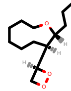
PhEthOH_1335.pdb
