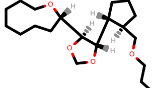
PhEthOH_2897.pdb
