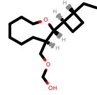
PhEthOH_1581.pdb
