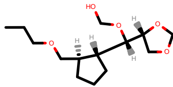
PhEthOH_2889.pdb
