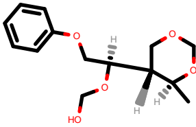
PhEthOH_380.pdb
