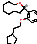
PhEthOH_3862.pdb
