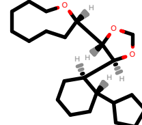
PhEthOH_4203.pdb
