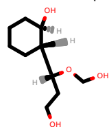
PhEthOH_770.pdb
