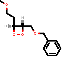
PhEthOH_1735.pdb
