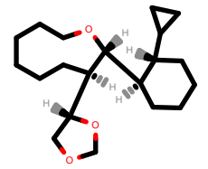
PhEthOH_3357.pdb
