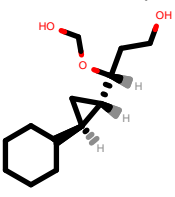
PhEthOH_4508.pdb
