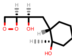
PhEthOH_782.pdb
