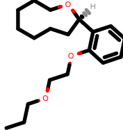
PhEthOH_1426.pdb
