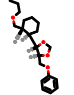
PhEthOH_2906.pdb
