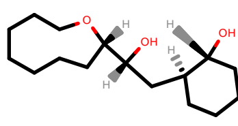
PhEthOH_794.pdb
