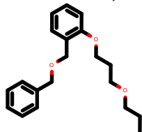
PhEthOH_2572.pdb
