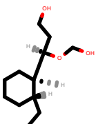
PhEthOH_1652.pdb
