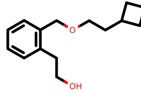
PhEthOH_3419.pdb
