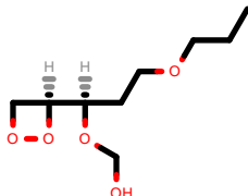
PhEthOH_2589.pdb
