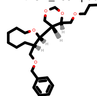
PhEthOH_2955.pdb
