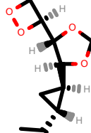
PhEthOH_1544.pdb
