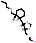
PhEthOH_2924.pdb
