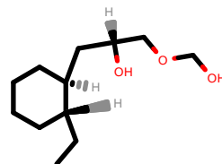
PhEthOH_1658.pdb
