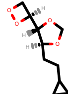
PhEthOH_3098.pdb
