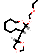
PhEthOH_2223.pdb
