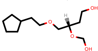
PhEthOH_4004.pdb
