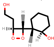
PhEthOH_771.pdb
