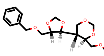
PhEthOH_2110.pdb
