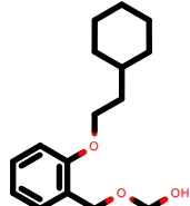
PhEthOH_4264.pdb
