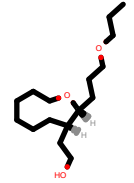
PhEthOH_2663.pdb
