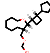
PhEthOH_4143.pdb
