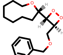
PhEthOH_1006.pdb
