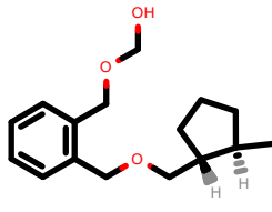
PhEthOH_317.pdb
