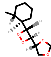
PhEthOH_374.pdb
