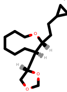
PhEthOH_3101.pdb
