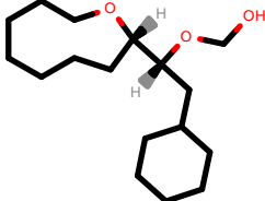
PhEthOH_4285.pdb
