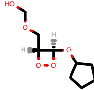
PhEthOH_3889.pdb
