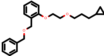
PhEthOH_3198.pdb
