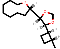
PhEthOH_297.pdb
