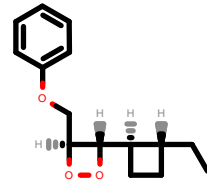
PhEthOH_1557.pdb
