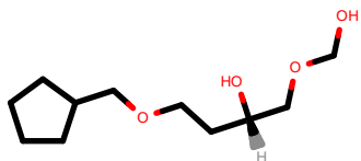
PhEthOH_3968.pdb
