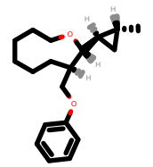
PhEthOH_219.pdb
