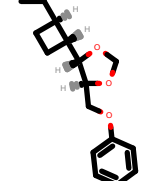
PhEthOH_1558.pdb
