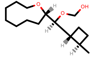
PhEthOH_295.pdb
