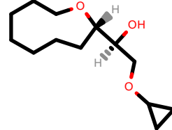
PhEthOH_3066.pdb
