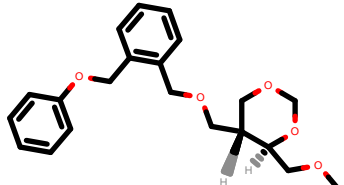
PhEthOH_2100.pdb
