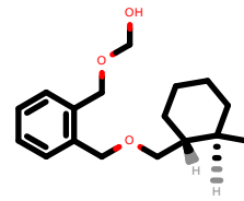
PhEthOH_359.pdb
