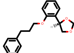
PhEthOH_958.pdb
