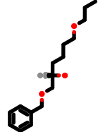
PhEthOH_2653.pdb
