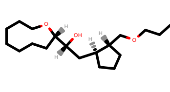
PhEthOH_2898.pdb
