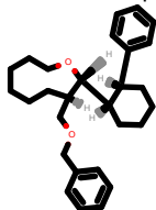
PhEthOH_1233.pdb
