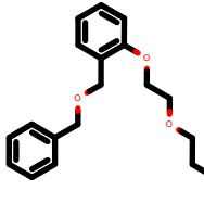
PhEthOH_178.pdb
