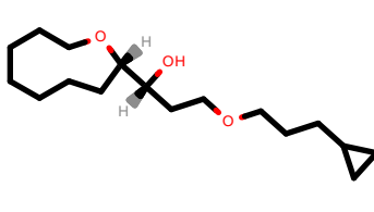
PhEthOH_3230.pdb
