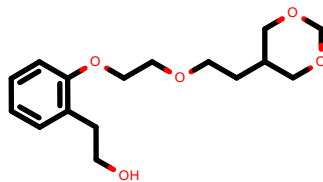
PhEthOH_4846.pdb
