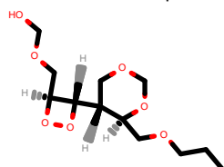
PhEthOH_2961.pdb
