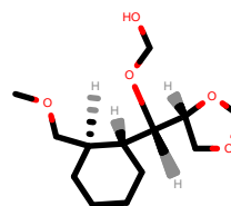
PhEthOH_2091.pdb
