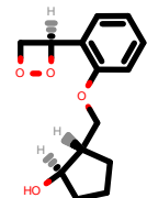
PhEthOH_738.pdb
