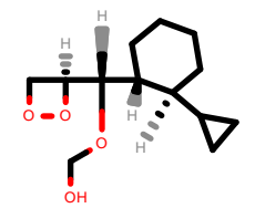
PhEthOH_3345.pdb
