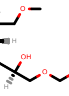
PhEthOH_1998.pdb
