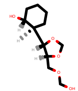
PhEthOH_778.pdb
