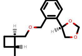
PhEthOH_283.pdb
