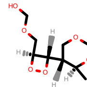
PhEthOH_403.pdb
