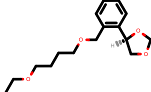
PhEthOH_2261.pdb
