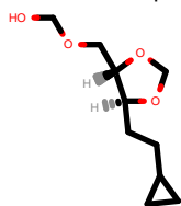
PhEthOH_3092.pdb
