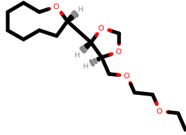
PhEthOH_2313.pdb
