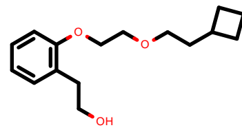
PhEthOH_3582.pdb
