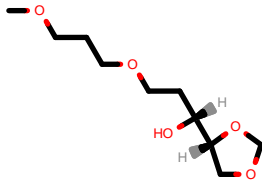
PhEthOH_1880.pdb
