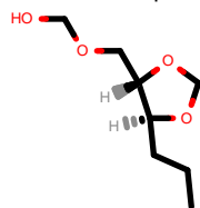
PhEthOH_64.pdb
