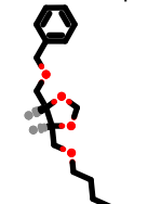
PhEthOH_178.pdb
