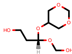
PhEthOH_4722.pdb
