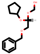
PhEthOH_3876.pdb
