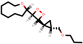
PhEthOH_2812.pdb
