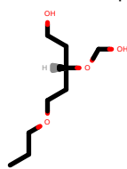
PhEthOH_2580.pdb
