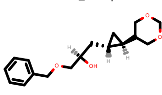
PhEthOH_4925.pdb
