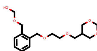
PhEthOH_4807.pdb
