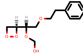
PhEthOH_1039.pdb
