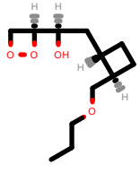
PhEthOH_2844.pdb
