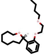
PhEthOH_208.pdb
