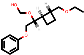
PhEthOH_2396.pdb
