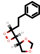
PhEthOH_958.pdb
