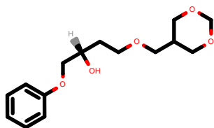
PhEthOH_4789.pdb
