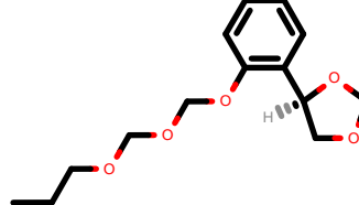
PhEthOH_2638.pdb
