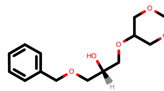
PhEthOH_4715.pdb
