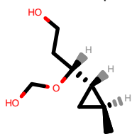
PhEthOH_228.pdb
