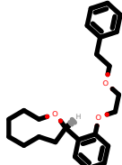
PhEthOH_1048.pdb
