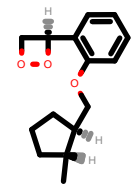
PhEthOH_318.pdb
