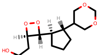
PhEthOH_5013.pdb
