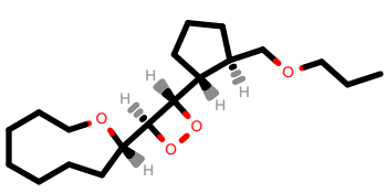
PhEthOH_2896.pdb
