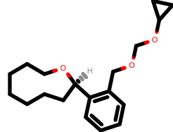
PhEthOH_3065.pdb
