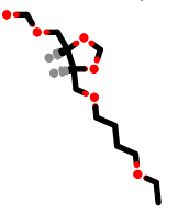
PhEthOH_2332.pdb
