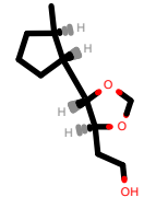
PhEthOH_314.pdb
