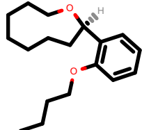
PhEthOH_78.pdb
