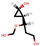
PhEthOH_648.pdb
