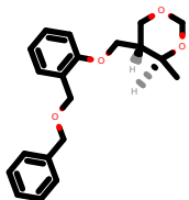
PhEthOH_388.pdb
