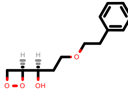
PhEthOH_1038.pdb
