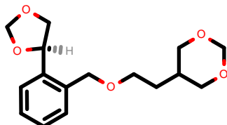
PhEthOH_4693.pdb
