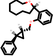
PhEthOH_1132.pdb
