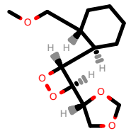
PhEthOH_2096.pdb
