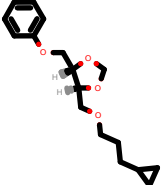
PhEthOH_3196.pdb
