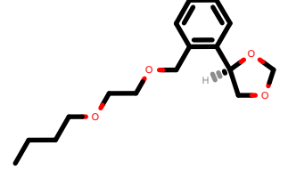
PhEthOH_203.pdb
