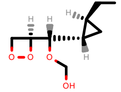
PhEthOH_1543.pdb
