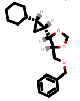
PhEthOH_4508.pdb
