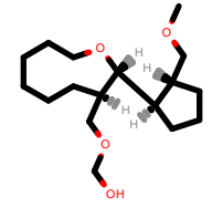
PhEthOH_2043.pdb
