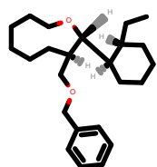
PhEthOH_1649.pdb
