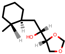
PhEthOH_372.pdb
