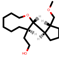
PhEthOH_2037.pdb
