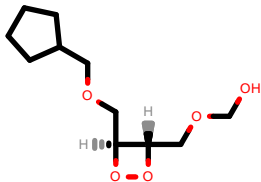
PhEthOH_3969.pdb
