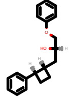
PhEthOH_1139.pdb
