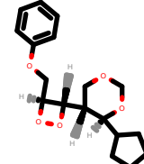
PhEthOH_4207.pdb
