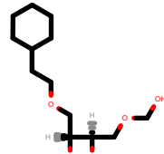
PhEthOH_4431.pdb
