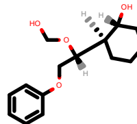
PhEthOH_758.pdb
