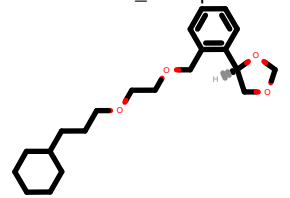
PhEthOH_4487.pdb
