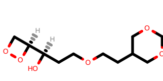
PhEthOH_4856.pdb
