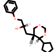
PhEthOH_4205.pdb
