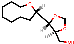
PhEthOH_465.pdb
