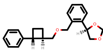
PhEthOH_1169.pdb
