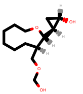
PhEthOH_657.pdb
