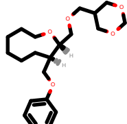
PhEthOH_4793.pdb
