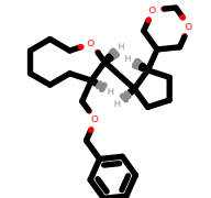
PhEthOH_5013.pdb
