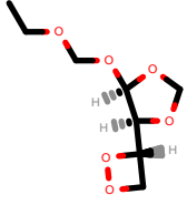
PhEthOH_2216.pdb
