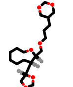
PhEthOH_4911.pdb
