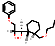
PhEthOH_2905.pdb
