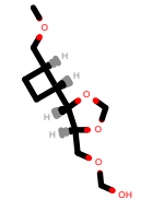
PhEthOH_2000.pdb
