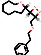
PhEthOH_1052.pdb
