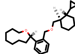
PhEthOH_3359.pdb
