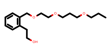
PhEthOH_2747.pdb
