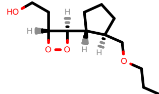
PhEthOH_2871.pdb
