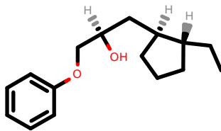
PhEthOH_1597.pdb
