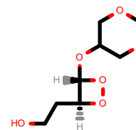
PhEthOH_4723.pdb
