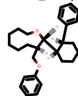
PhEthOH_1227.pdb
