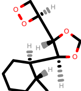
PhEthOH_368.pdb
