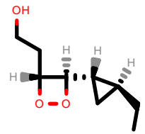
PhEthOH_1531.pdb
