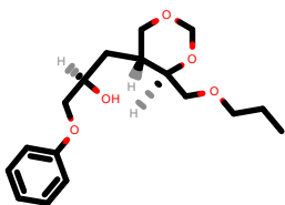
PhEthOH_2941.pdb
