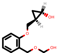
PhEthOH_652.pdb
