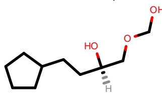
PhEthOH_3846.pdb
