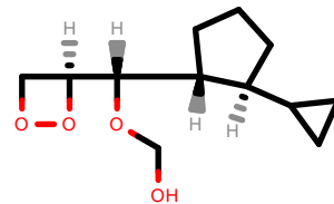
PhEthOH_3307.pdb
