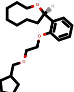
PhEthOH_3984.pdb
