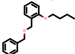
PhEthOH_48.pdb
