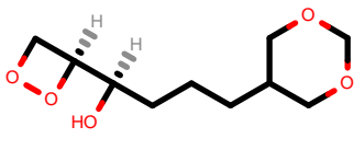
PhEthOH_4776.pdb
