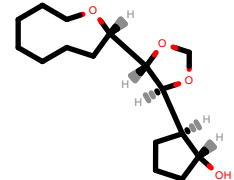
PhEthOH_759.pdb
