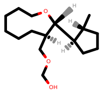
PhEthOH_317.pdb
