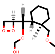
PhEthOH_2085.pdb
