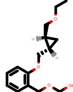
PhEthOH_2374.pdb
