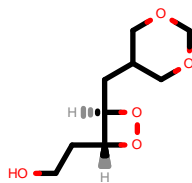
PhEthOH_4677.pdb
