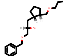
PhEthOH_2867.pdb
