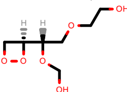
PhEthOH_573.pdb
