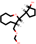
PhEthOH_737.pdb
