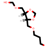
PhEthOH_1870.pdb
