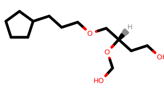
PhEthOH_4050.pdb
