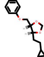
PhEthOH_3070.pdb
