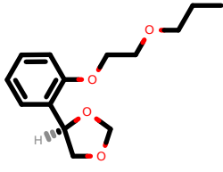
PhEthOH_156.pdb
