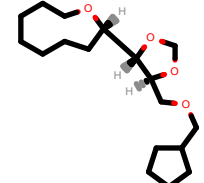
PhEthOH_3989.pdb
