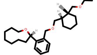
PhEthOH_2519.pdb
