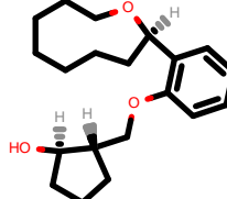
PhEthOH_754.pdb
