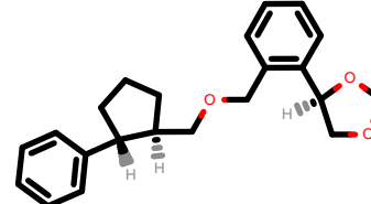
PhEthOH_1207.pdb
