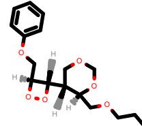
PhEthOH_2943.pdb
