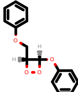
PhEthOH_889.pdb
