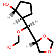
PhEthOH_747.pdb
