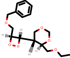
PhEthOH_2533.pdb
