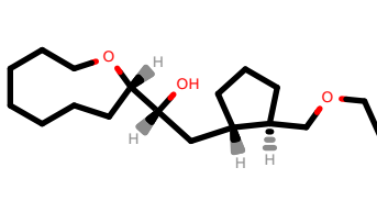
PhEthOH_2474.pdb
