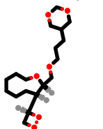
PhEthOH_4901.pdb
