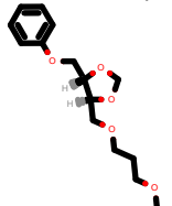
PhEthOH_1852.pdb
