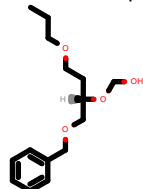
PhEthOH_2574.pdb
