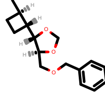
PhEthOH_266.pdb
