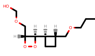
PhEthOH_2839.pdb
