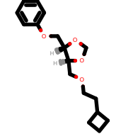
PhEthOH_3578.pdb
