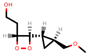
PhEthOH_1951.pdb
