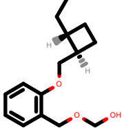
PhEthOH_1576.pdb
