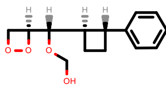
PhEthOH_1165.pdb
