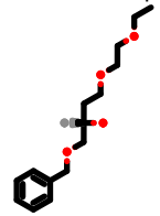
PhEthOH_2279.pdb
