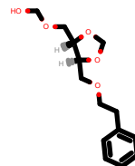
PhEthOH_1034.pdb
