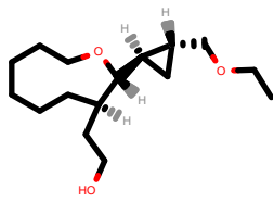
PhEthOH_2373.pdb
