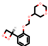
PhEthOH_4732.pdb
