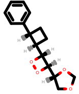
PhEthOH_1172.pdb
