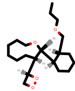
PhEthOH_2931.pdb
