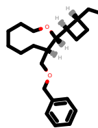
PhEthOH_1565.pdb
