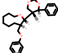
PhEthOH_1269.pdb
