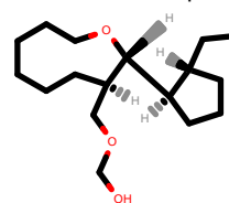
PhEthOH_1619.pdb
