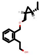
PhEthOH_1529.pdb
