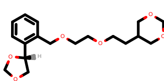
PhEthOH_4861.pdb
