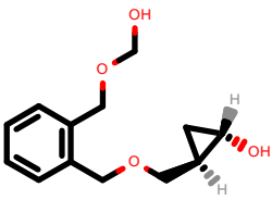
PhEthOH_653.pdb
