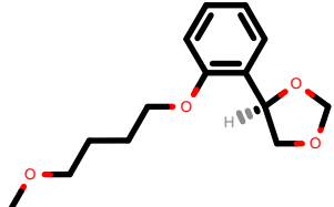
PhEthOH_1840.pdb
