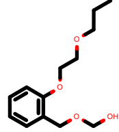
PhEthOH_148.pdb
