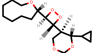
PhEthOH_3404.pdb
