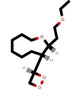
PhEthOH_2175.pdb
