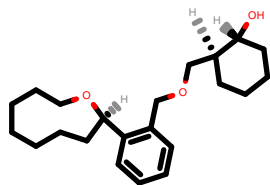
PhEthOH_793.pdb
