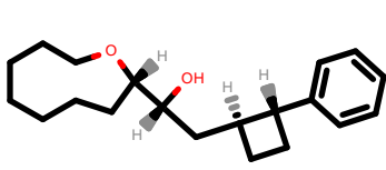
PhEthOH_1172.pdb
