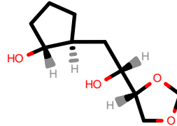
PhEthOH_746.pdb
