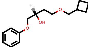
PhEthOH_3533.pdb
