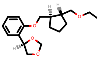
PhEthOH_2470.pdb
