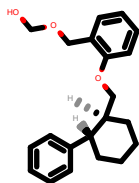
PhEthOH_1236.pdb
