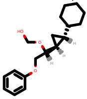
PhEthOH_4500.pdb
