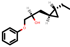
PhEthOH_1517.pdb
