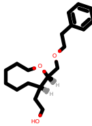
PhEthOH_1029.pdb
