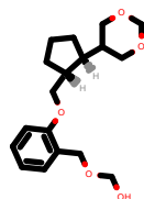
PhEthOH_5020.pdb
