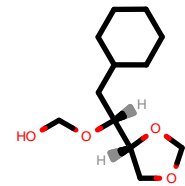
PhEthOH_4279.pdb
