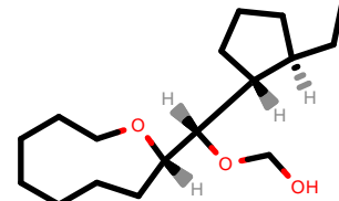
PhEthOH_1635.pdb
