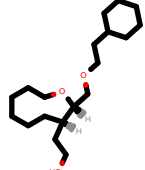
PhEthOH_4431.pdb
