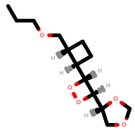
PhEthOH_2852.pdb
