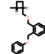
PhEthOH_252.pdb
