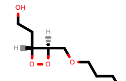
PhEthOH_183.pdb
