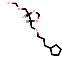
PhEthOH_4058.pdb
