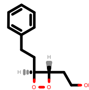
PhEthOH_939.pdb
