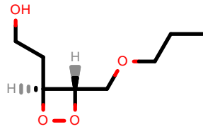
PhEthOH_145.pdb
