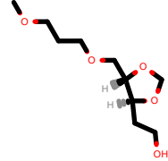
PhEthOH_1864.pdb
