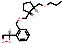
PhEthOH_2881.pdb
