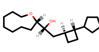
PhEthOH_4158.pdb
