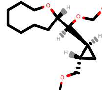
PhEthOH_1975.pdb
