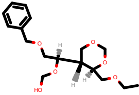
PhEthOH_2528.pdb
