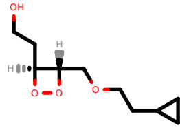
PhEthOH_3165.pdb
