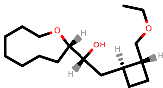
PhEthOH_2432.pdb
