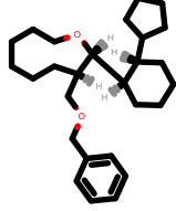
PhEthOH_4173.pdb
