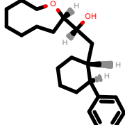
PhEthOH_1256.pdb
