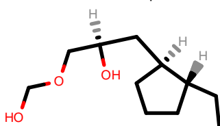
PhEthOH_1616.pdb
