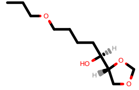
PhEthOH_2682.pdb
