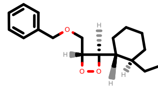
PhEthOH_1651.pdb
