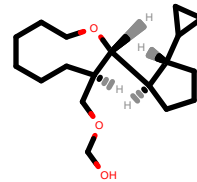
PhEthOH_3303.pdb
