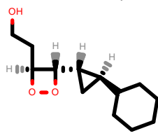
PhEthOH_4509.pdb
