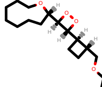
PhEthOH_2434.pdb
