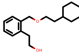
PhEthOH_4255.pdb
