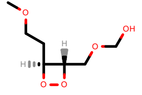
PhEthOH_1747.pdb
