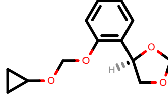
PhEthOH_3058.pdb
