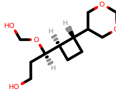
PhEthOH_4974.pdb
