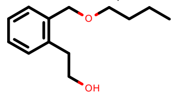
PhEthOH_1319.pdb
