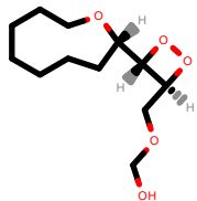
PhEthOH_548.pdb
