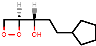
PhEthOH_3852.pdb
