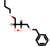
PhEthOH_139.pdb
