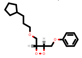
PhEthOH_4039.pdb
