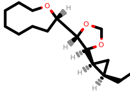
PhEthOH_1553.pdb
