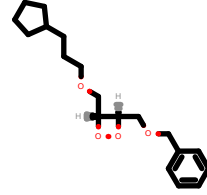
PhEthOH_4045.pdb
