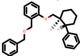
PhEthOH_1228.pdb
