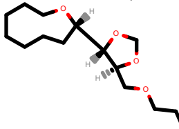
PhEthOH_167.pdb
