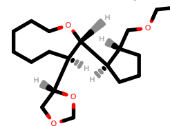
PhEthOH_2471.pdb
