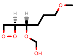
PhEthOH_1833.pdb
