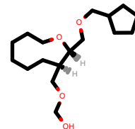
PhEthOH_3971.pdb
