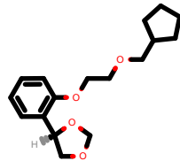
PhEthOH_3982.pdb
