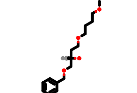
PhEthOH_1897.pdb
