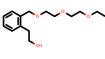
PhEthOH_2285.pdb
