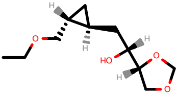
PhEthOH_2388.pdb
