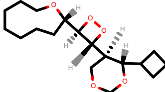
PhEthOH_3824.pdb
