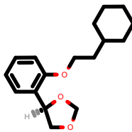
PhEthOH_4276.pdb
