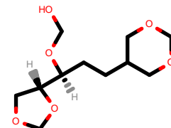
PhEthOH_4779.pdb
