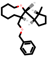
PhEthOH_309.pdb
