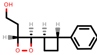
PhEthOH_1149.pdb
