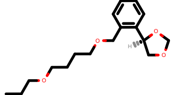
PhEthOH_2681.pdb
