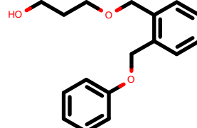
PhEthOH_466.pdb
