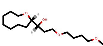
PhEthOH_1928.pdb
