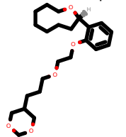
PhEthOH_4912.pdb
