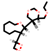
PhEthOH_2549.pdb
