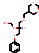
PhEthOH_4790.pdb
