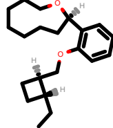
PhEthOH_1594.pdb
