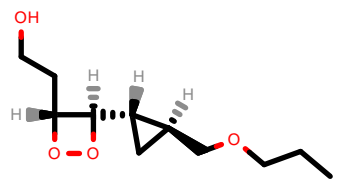
PhEthOH_2787.pdb
