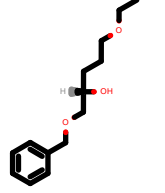
PhEthOH_2153.pdb
