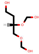
PhEthOH_518.pdb
