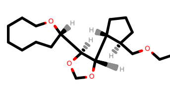
PhEthOH_2477.pdb
