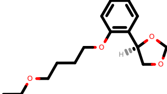
PhEthOH_2260.pdb
