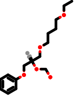
PhEthOH_2316.pdb
