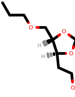
PhEthOH_146.pdb
