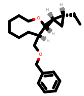
PhEthOH_1527.pdb
