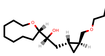
PhEthOH_2814.pdb
