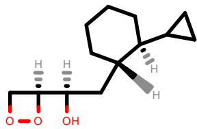
PhEthOH_3344.pdb
