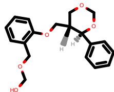
PhEthOH_1278.pdb
