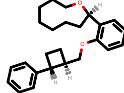
PhEthOH_1174.pdb
