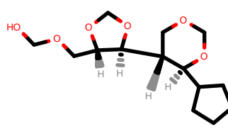
PhEthOH_4222.pdb
