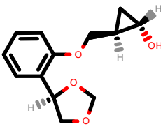
PhEthOH_664.pdb
