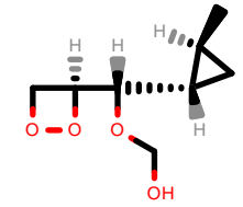
PhEthOH_241.pdb
