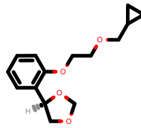
PhEthOH_3142.pdb
