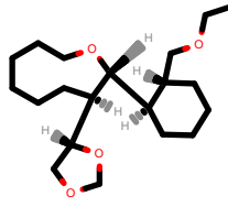
PhEthOH_2517.pdb
