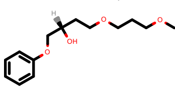
PhEthOH_1853.pdb
