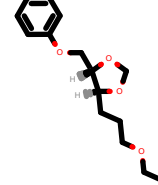
PhEthOH_2234.pdb
