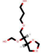
PhEthOH_625.pdb
