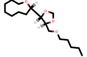
PhEthOH_1515.pdb
