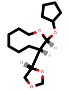
PhEthOH_3903.pdb
