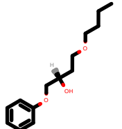
PhEthOH_169.pdb
