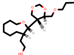
PhEthOH_2957.pdb
