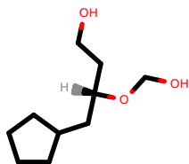
PhEthOH_3836.pdb
