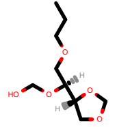
PhEthOH_1423.pdb
