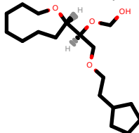
PhEthOH_4029.pdb
