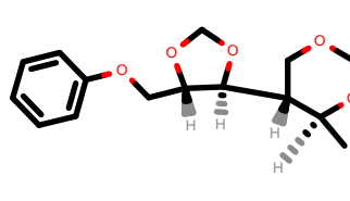
PhEthOH_382.pdb
