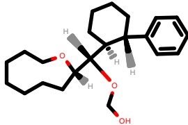
PhEthOH_1257.pdb
