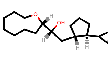
PhEthOH_3318.pdb
