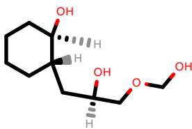
PhEthOH_776.pdb
