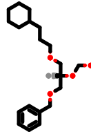
PhEthOH_4464.pdb
