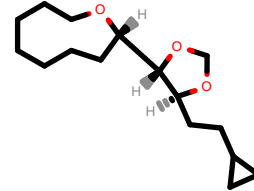
PhEthOH_3111.pdb
