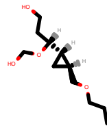
PhEthOH_2786.pdb
