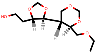
PhEthOH_2536.pdb
