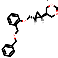
PhEthOH_4924.pdb
