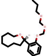
PhEthOH_2644.pdb
