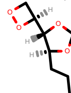
PhEthOH_70.pdb
