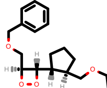
PhEthOH_2449.pdb
