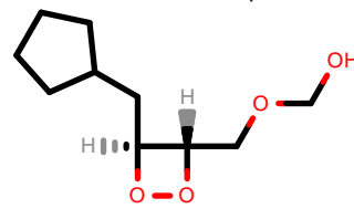
PhEthOH_3847.pdb
