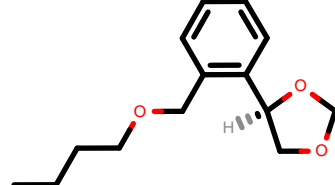
PhEthOH_1337.pdb
