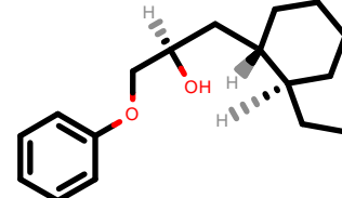
PhEthOH_1643.pdb
