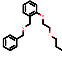
PhEthOH_1438.pdb
