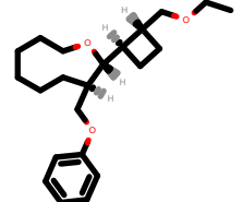
PhEthOH_2399.pdb
