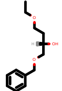
PhEthOH_91.pdb
