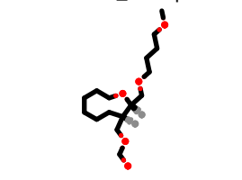
PhEthOH_1917.pdb
