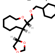
PhEthOH_4403.pdb
