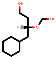
PhEthOH_4260.pdb
