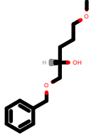
PhEthOH_1733.pdb
