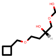
PhEthOH_3548.pdb
