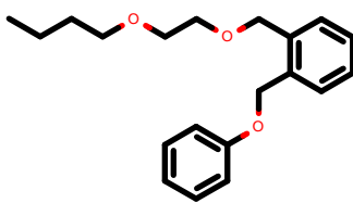
PhEthOH_168.pdb
