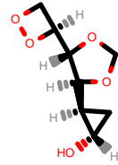
PhEthOH_662.pdb
