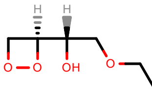
PhEthOH_1374.pdb
