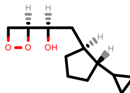
PhEthOH_3306.pdb
