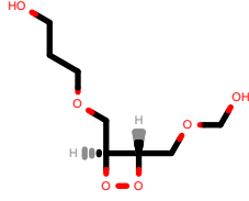
PhEthOH_613.pdb
