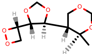
PhEthOH_406.pdb
