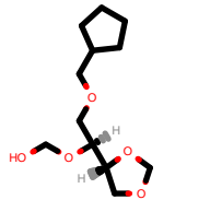
PhEthOH_3985.pdb
