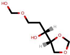
PhEthOH_540.pdb
