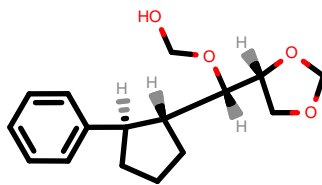
PhEthOH_1213.pdb
