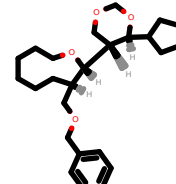
PhEthOH_4215.pdb
