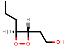
PhEthOH_1317.pdb
