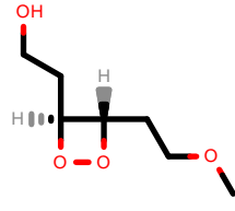
PhEthOH_1741.pdb
