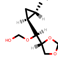
PhEthOH_247.pdb
