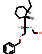
PhEthOH_1650.pdb
