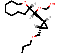
PhEthOH_2815.pdb
