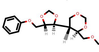
PhEthOH_2108.pdb
