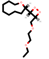
PhEthOH_2312.pdb
