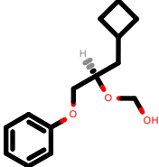
PhEthOH_3408.pdb
