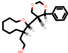
PhEthOH_1277.pdb
