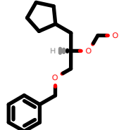
PhEthOH_3834.pdb
