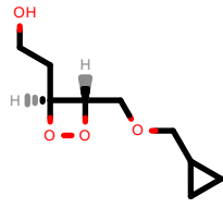
PhEthOH_3127.pdb
