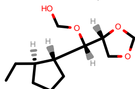
PhEthOH_1629.pdb
