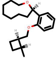
PhEthOH_292.pdb
