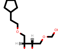
PhEthOH_4015.pdb
