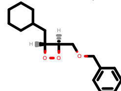
PhEthOH_4255.pdb
