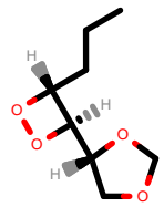
PhEthOH_76.pdb
