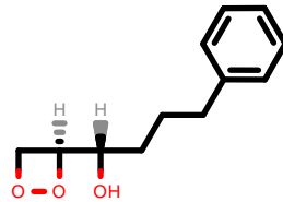
PhEthOH_954.pdb
