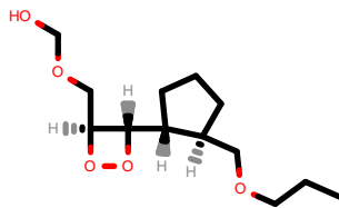
PhEthOH_2877.pdb
