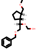
PhEthOH_2028.pdb
