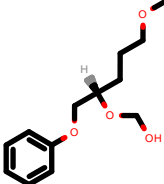
PhEthOH_1812.pdb
