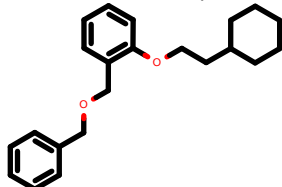
PhEthOH_4252.pdb
