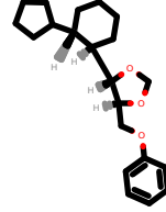
PhEthOH_4166.pdb
