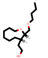
PhEthOH_185.pdb
