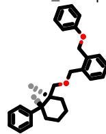
PhEthOH_1222.pdb
