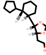
PhEthOH_4178.pdb
