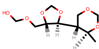
PhEthOH_400.pdb
