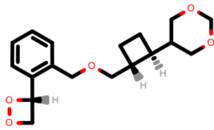
PhEthOH_4985.pdb
