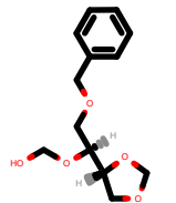
PhEthOH_1003.pdb
