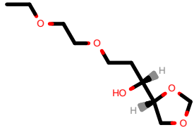
PhEthOH_2300.pdb
