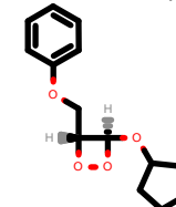
PhEthOH_3871.pdb
