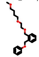
PhEthOH_1894.pdb
