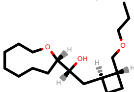
PhEthOH_2856.pdb
