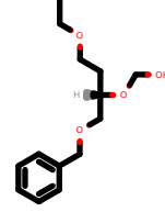
PhEthOH_2154.pdb
