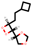
PhEthOH_3520.pdb
