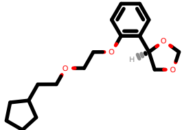
PhEthOH_4024.pdb
