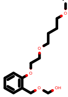
PhEthOH_1912.pdb
