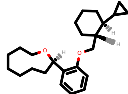
PhEthOH_3358.pdb
