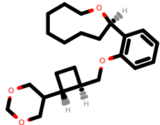
PhEthOH_4992.pdb
