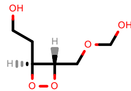
PhEthOH_483.pdb
