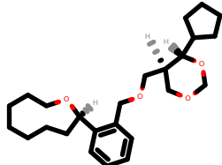
PhEthOH_4241.pdb
