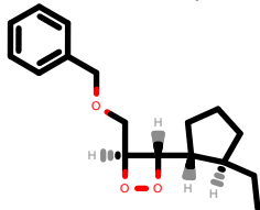
PhEthOH_1609.pdb
