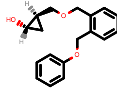
PhEthOH_634.pdb
