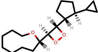
PhEthOH_3320.pdb
