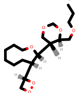
PhEthOH_2969.pdb
