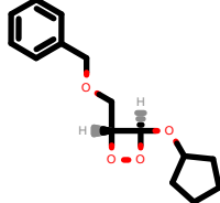
PhEthOH_3877.pdb
