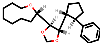
PhEthOH_1217.pdb
