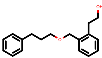
PhEthOH_937.pdb
