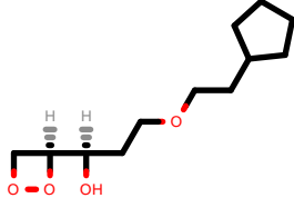
PhEthOH_4020.pdb
