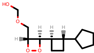
PhEthOH_4141.pdb
