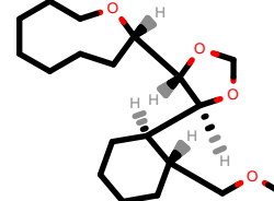
PhEthOH_2103.pdb
