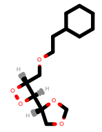
PhEthOH_4444.pdb
