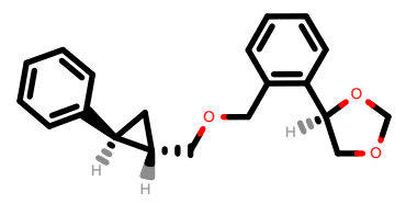
PhEthOH_1127.pdb
