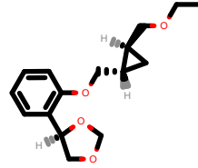
PhEthOH_2386.pdb
