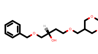
PhEthOH_4795.pdb
