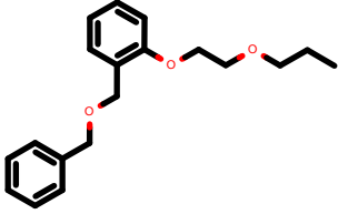
PhEthOH_136.pdb
