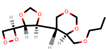
PhEthOH_2968.pdb
