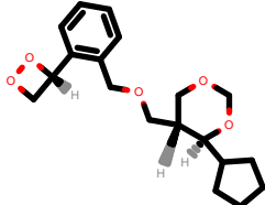
PhEthOH_4229.pdb
