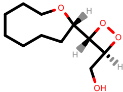
PhEthOH_464.pdb
