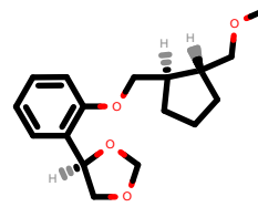
PhEthOH_2046.pdb
