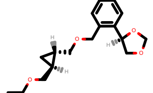
PhEthOH_2387.pdb
