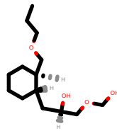
PhEthOH_2922.pdb
