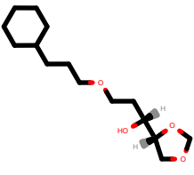
PhEthOH_4488.pdb
