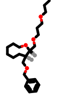
PhEthOH_2745.pdb
