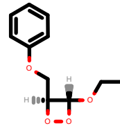
PhEthOH_1351.pdb
