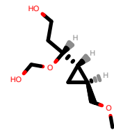
PhEthOH_1950.pdb
