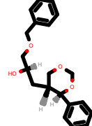
PhEthOH_1271.pdb
