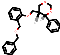
PhEthOH_1270.pdb
