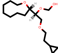
PhEthOH_3193.pdb
