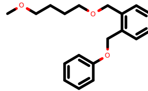
PhEthOH_1810.pdb
