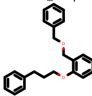
PhEthOH_934.pdb
