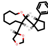
PhEthOH_1215.pdb
