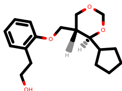
PhEthOH_4212.pdb
