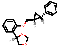
PhEthOH_1126.pdb
