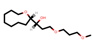
PhEthOH_1886.pdb
