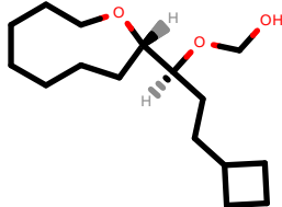
PhEthOH_3529.pdb
