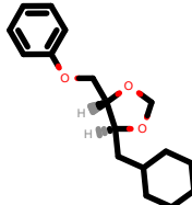
PhEthOH_4250.pdb
