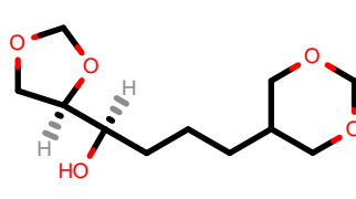
PhEthOH_4778.pdb
