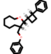
PhEthOH_1143.pdb
