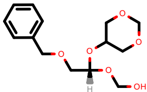
PhEthOH_4712.pdb
