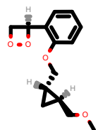
PhEthOH_1960.pdb
