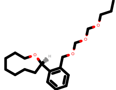
PhEthOH_2645.pdb
