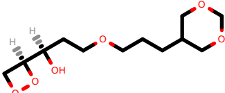
PhEthOH_4902.pdb
