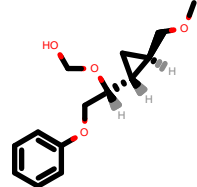
PhEthOH_1938.pdb
