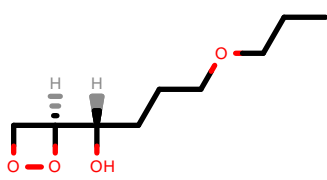
PhEthOH_2588.pdb
