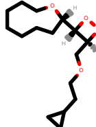
PhEthOH_3194.pdb
