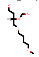
PhEthOH_1908.pdb
