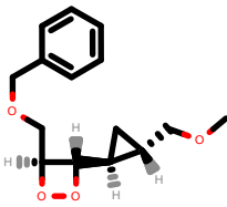
PhEthOH_1945.pdb
