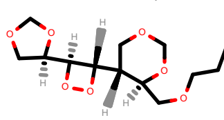
PhEthOH_2974.pdb
