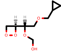
PhEthOH_3135.pdb
