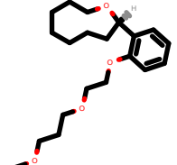
PhEthOH_1884.pdb
