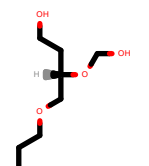
PhEthOH_182.pdb
