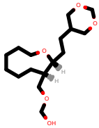
PhEthOH_4773.pdb
