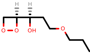
PhEthOH_1416.pdb
