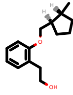
PhEthOH_310.pdb
