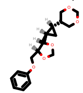
PhEthOH_4922.pdb
