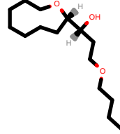
PhEthOH_210.pdb
