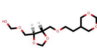
PhEthOH_4852.pdb
