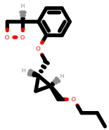
PhEthOH_2800.pdb
