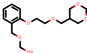
PhEthOH_4806.pdb
