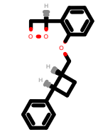
PhEthOH_1162.pdb
