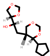
PhEthOH_4232.pdb
