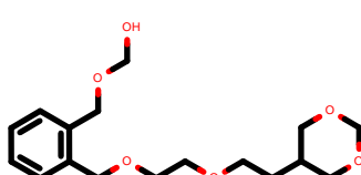
PhEthOH_4849.pdb
