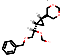
PhEthOH_4926.pdb
