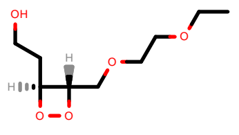
PhEthOH_2287.pdb
