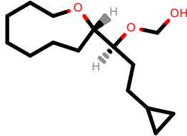
PhEthOH_3109.pdb
