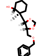
PhEthOH_766.pdb
