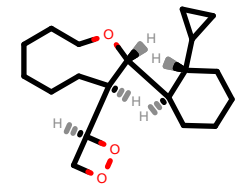
PhEthOH_3347.pdb
