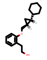
PhEthOH_4510.pdb
