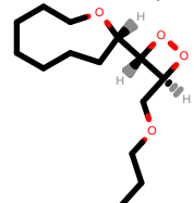
PhEthOH_166.pdb
