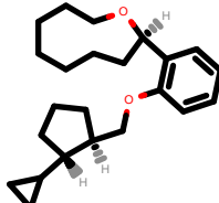
PhEthOH_3316.pdb
