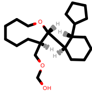
PhEthOH_4185.pdb
