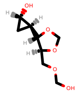
PhEthOH_656.pdb
