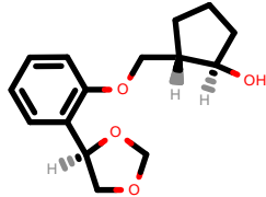
PhEthOH_744.pdb
