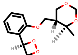
PhEthOH_406.pdb
