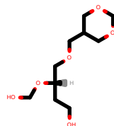
PhEthOH_4806.pdb
