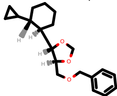
PhEthOH_3332.pdb
