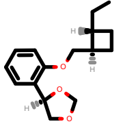
PhEthOH_1588.pdb
