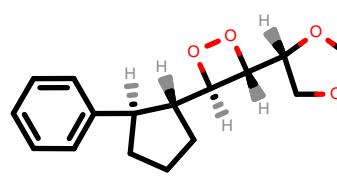
PhEthOH_1214.pdb
