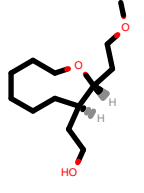
PhEthOH_1743.pdb
