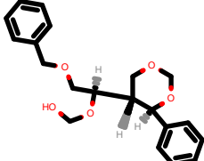
PhEthOH_1268.pdb
