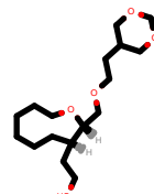
PhEthOH_4847.pdb
