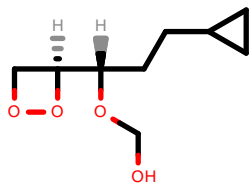
PhEthOH_3097.pdb
