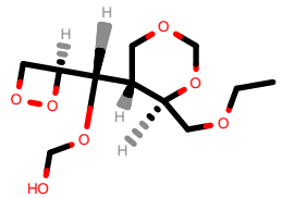
PhEthOH_2547.pdb
