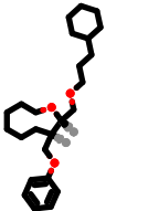
PhEthOH_4461.pdb
