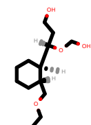
PhEthOH_2492.pdb
