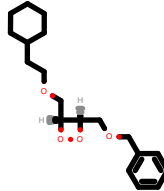
PhEthOH_4423.pdb
