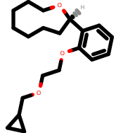
PhEthOH_3148.pdb
