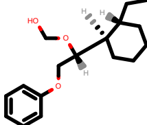
PhEthOH_1644.pdb
