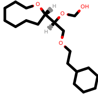
PhEthOH_4453.pdb
