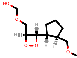
PhEthOH_2041.pdb
