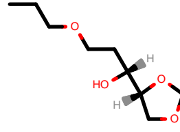
PhEthOH_158.pdb
