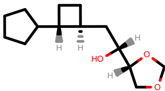
PhEthOH_4148.pdb
