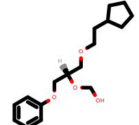
PhEthOH_3996.pdb
