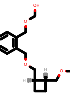
PhEthOH_1997.pdb
