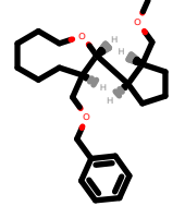
PhEthOH_2031.pdb
