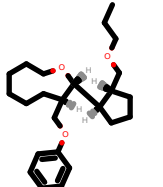
PhEthOH_2865.pdb
