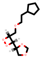
PhEthOH_4028.pdb
