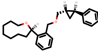
PhEthOH_1133.pdb
