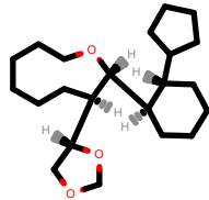
PhEthOH_4197.pdb
