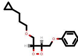
PhEthOH_3199.pdb
