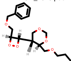
PhEthOH_2953.pdb
