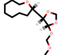
PhEthOH_1809.pdb
