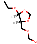
PhEthOH_1370.pdb
