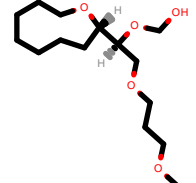
PhEthOH_1887.pdb
