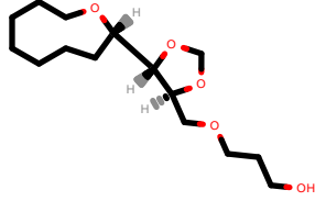
PhEthOH_633.pdb
