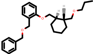
PhEthOH_2908.pdb
