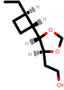
PhEthOH_1574.pdb
