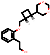
PhEthOH_4972.pdb
