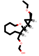
PhEthOH_2379.pdb
