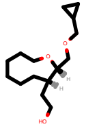
PhEthOH_3129.pdb
