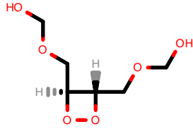
PhEthOH_529.pdb
