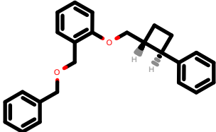
PhEthOH_1144.pdb
