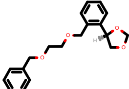
PhEthOH_1001.pdb
