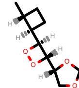
PhEthOH_286.pdb
