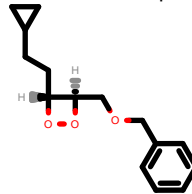
PhEthOH_3079.pdb
