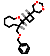
PhEthOH_4971.pdb
