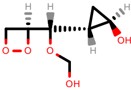
PhEthOH_661.pdb
