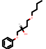
PhEthOH_1433.pdb
