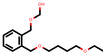
PhEthOH_2245.pdb
