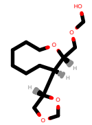
PhEthOH_543.pdb
