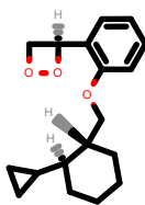
PhEthOH_3342.pdb
