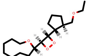
PhEthOH_2476.pdb
