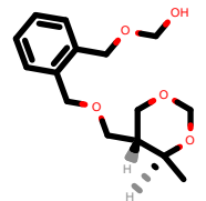
PhEthOH_401.pdb
