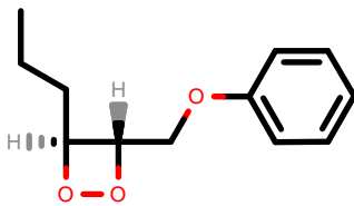
PhEthOH_45.pdb
