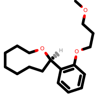
PhEthOH_1758.pdb
