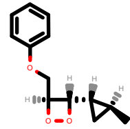
PhEthOH_217.pdb
