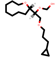
PhEthOH_3231.pdb
