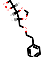
PhEthOH_1040.pdb
