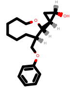
PhEthOH_639.pdb
