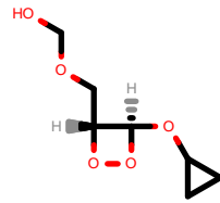
PhEthOH_3049.pdb
