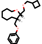
PhEthOH_3537.pdb
