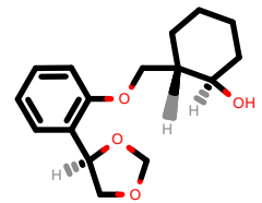
PhEthOH_786.pdb
