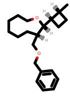
PhEthOH_267.pdb
