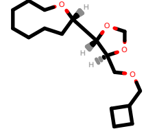
PhEthOH_3573.pdb
