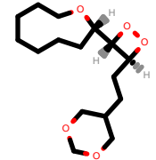
PhEthOH_4786.pdb
