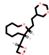
PhEthOH_4775.pdb
