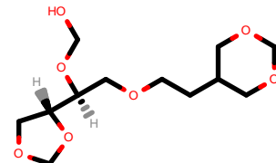
PhEthOH_4863.pdb
