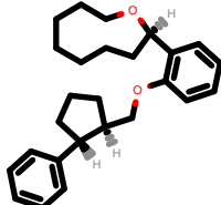
PhEthOH_1212.pdb
