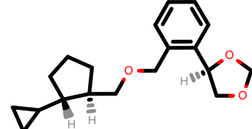
PhEthOH_3311.pdb
