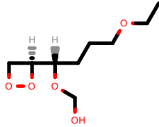
PhEthOH_2257.pdb
