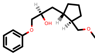
PhEthOH_2017.pdb
