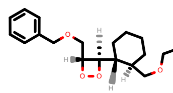
PhEthOH_2487.pdb
