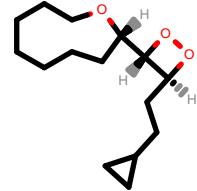
PhEthOH_3110.pdb
