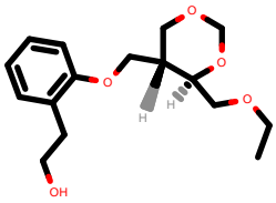
PhEthOH_2532.pdb
