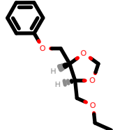
PhEthOH_88.pdb
