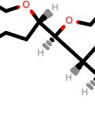
PhEthOH_2013.pdb
