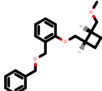
PhEthOH_1980.pdb
