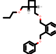
PhEthOH_2814.pdb
