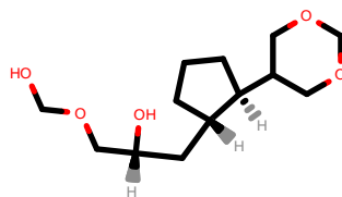
PhEthOH_5022.pdb
