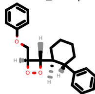
PhEthOH_1225.pdb
