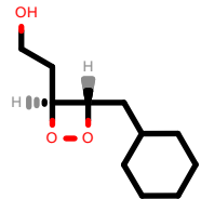
PhEthOH_4261.pdb
