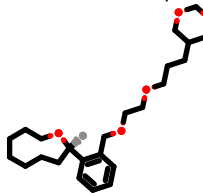
PhEthOH_4913.pdb
