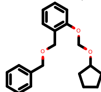
PhEthOH_3870.pdb
