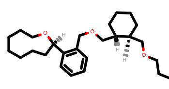
PhEthOH_2939.pdb
