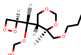
PhEthOH_2967.pdb
