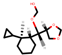
PhEthOH_3351.pdb
