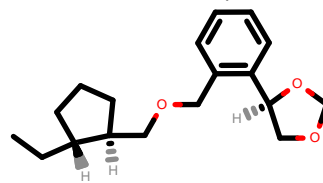
PhEthOH_1627.pdb
