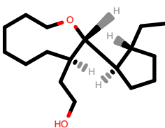
PhEthOH_1613.pdb
