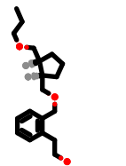
PhEthOH_2869.pdb
