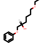
PhEthOH_2231.pdb
