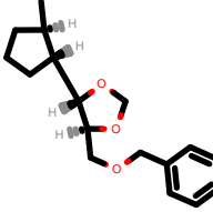
PhEthOH_308.pdb
