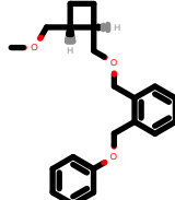
PhEthOH_1978.pdb
