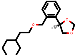
PhEthOH_4277.pdb
