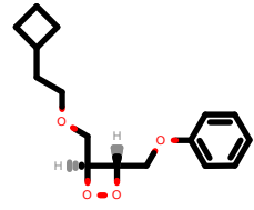
PhEthOH_3577.pdb
