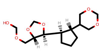
PhEthOH_5020.pdb
