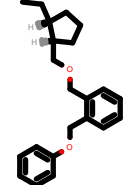
PhEthOH_1596.pdb
