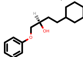
PhEthOH_4247.pdb
