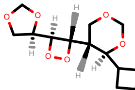
PhEthOH_3818.pdb
