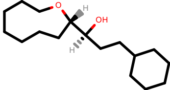
PhEthOH_4284.pdb
