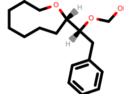
PhEthOH_883.pdb
