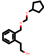
PhEthOH_3881.pdb
