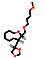
PhEthOH_1929.pdb
