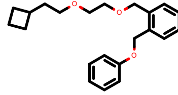
PhEthOH_3574.pdb
