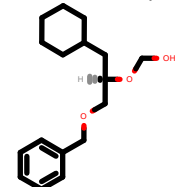
PhEthOH_4254.pdb
