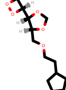
PhEthOH_4022.pdb
