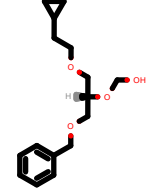
PhEthOH_3162.pdb
