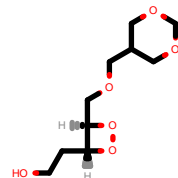
PhEthOH_4807.pdb
