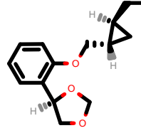
PhEthOH_1546.pdb
