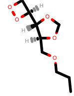
PhEthOH_158.pdb
