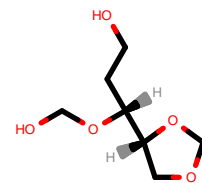
PhEthOH_495.pdb
