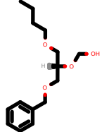
PhEthOH_1436.pdb
