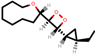
PhEthOH_1552.pdb
