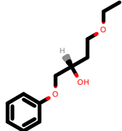
PhEthOH_85.pdb
