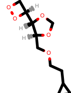
PhEthOH_3182.pdb
