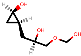
PhEthOH_654.pdb
