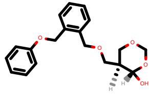
PhEthOH_798.pdb
