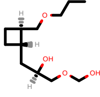
PhEthOH_2838.pdb
