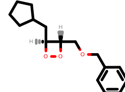
PhEthOH_3835.pdb
