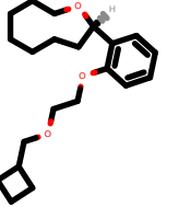
PhEthOH_3568.pdb
