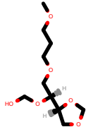
PhEthOH_1881.pdb
