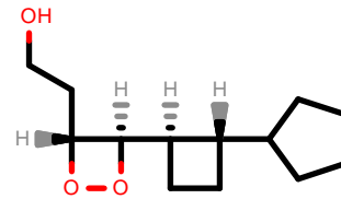
PhEthOH_4135.pdb
