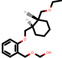
PhEthOH_2500.pdb
