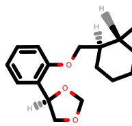
PhEthOH_370.pdb
