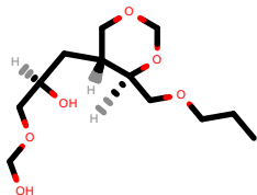
PhEthOH_2964.pdb
