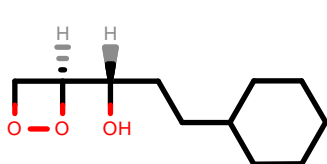
PhEthOH_4268.pdb
