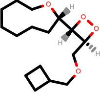
PhEthOH_3572.pdb
