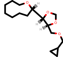
PhEthOH_3153.pdb
