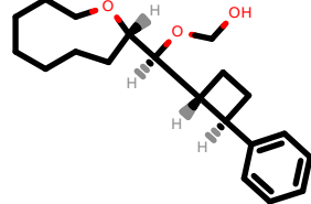
PhEthOH_1177.pdb
