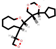
PhEthOH_4233.pdb
