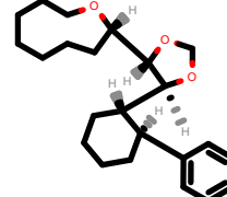
PhEthOH_1259.pdb
