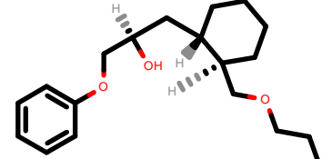
PhEthOH_2899.pdb
