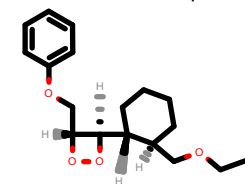
PhEthOH_2481.pdb
