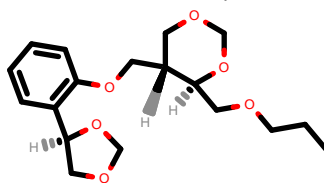
PhEthOH_2970.pdb
