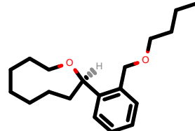
PhEthOH_79.pdb
