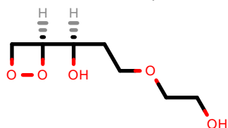
PhEthOH_572.pdb
