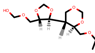
PhEthOH_2542.pdb
