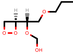
PhEthOH_1417.pdb
