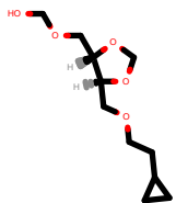
PhEthOH_3176.pdb
