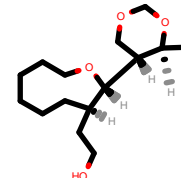
PhEthOH_395.pdb
