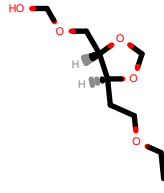
PhEthOH_2168.pdb
