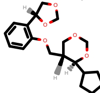
PhEthOH_4234.pdb
