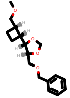
PhEthOH_1988.pdb
