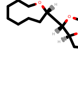
PhEthOH_2271.pdb
