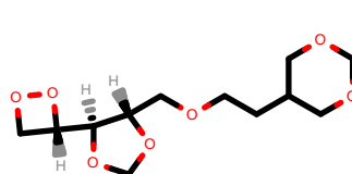
PhEthOH_4858.pdb
