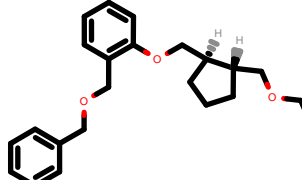
PhEthOH_2446.pdb
