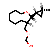
PhEthOH_237.pdb
