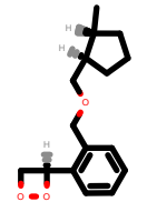
PhEthOH_319.pdb
