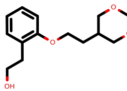
PhEthOH_4678.pdb
