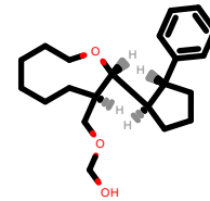
PhEthOH_1203.pdb
