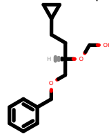
PhEthOH_3078.pdb
