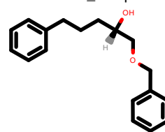
PhEthOH_935.pdb
