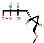
PhEthOH_1962.pdb
