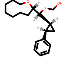
PhEthOH_1135.pdb
