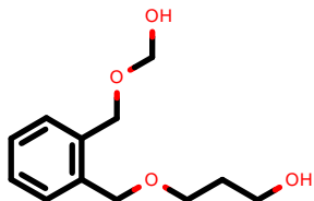
PhEthOH_481.pdb
