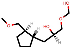
PhEthOH_2040.pdb
