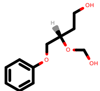
PhEthOH_468.pdb
