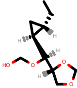
PhEthOH_1545.pdb
