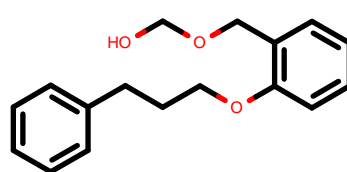
PhEthOH_942.pdb
