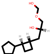
PhEthOH_4140.pdb
