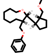
PhEthOH_2025.pdb
