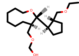
PhEthOH_2463.pdb
