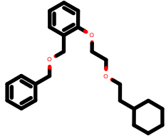
PhEthOH_4420.pdb
