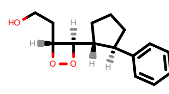
PhEthOH_1191.pdb
