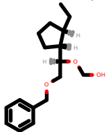
PhEthOH_1608.pdb
