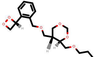
PhEthOH_2965.pdb
