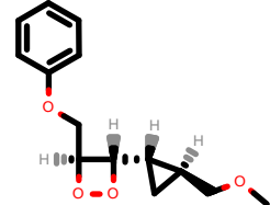
PhEthOH_1939.pdb
