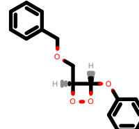
PhEthOH_895.pdb
