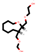
PhEthOH_573.pdb
