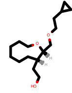
PhEthOH_3167.pdb
