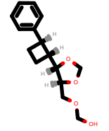
PhEthOH_1160.pdb
