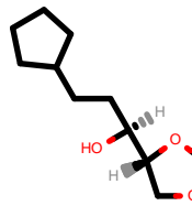
PhEthOH_3858.pdb
