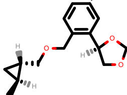
PhEthOH_245.pdb
