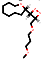
PhEthOH_1892.pdb
