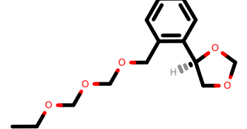
PhEthOH_2219.pdb
