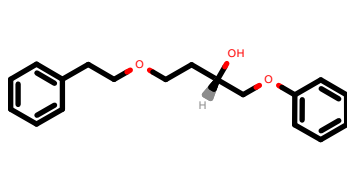
PhEthOH_1009.pdb
