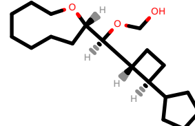
PhEthOH_4159.pdb
