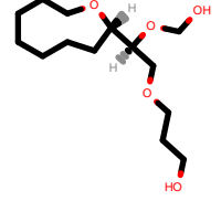
PhEthOH_631.pdb
