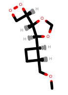
PhEthOH_2006.pdb
