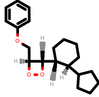
PhEthOH_4165.pdb
