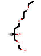
PhEthOH_2292.pdb
