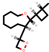
PhEthOH_281.pdb
