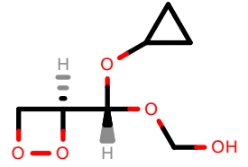
PhEthOH_3055.pdb
