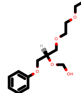
PhEthOH_2270.pdb
