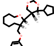
PhEthOH_4205.pdb
