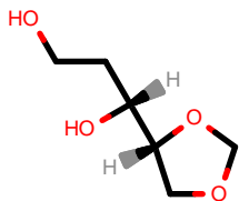
PhEthOH_452.pdb
