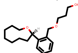
PhEthOH_499.pdb
