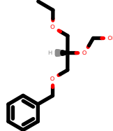
PhEthOH_92.pdb
