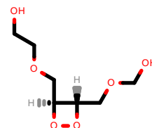
PhEthOH_567.pdb
