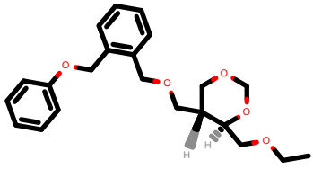
PhEthOH_2524.pdb
