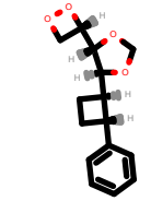
PhEthOH_1166.pdb
