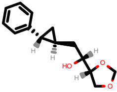
PhEthOH_1128.pdb
