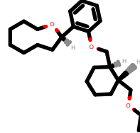
PhEthOH_2518.pdb
