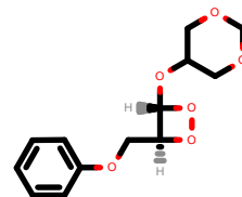
PhEthOH_4711.pdb
