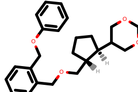
PhEthOH_4998.pdb
