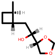
PhEthOH_284.pdb
