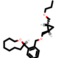
PhEthOH_2813.pdb
