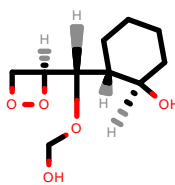
PhEthOH_783.pdb
