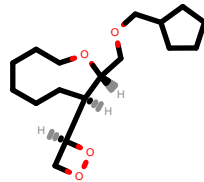
PhEthOH_3981.pdb
