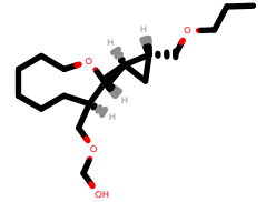
PhEthOH_2795.pdb
