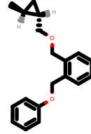
PhEthOH_214.pdb
