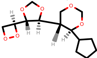
PhEthOH_4232.pdb
