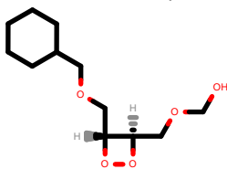
PhEthOH_4389.pdb
