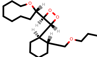
PhEthOH_2942.pdb
