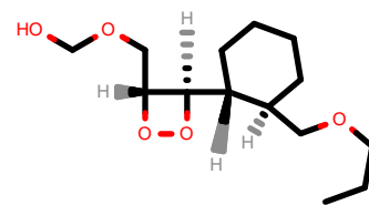
PhEthOH_2923.pdb
