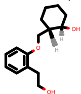
PhEthOH_768.pdb
