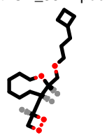
PhEthOH_3645.pdb
