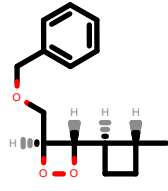
PhEthOH_265.pdb
