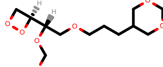
PhEthOH_4903.pdb
