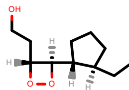
PhEthOH_1611.pdb
