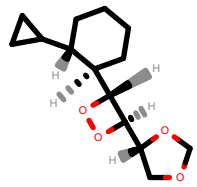
PhEthOH_3356.pdb
