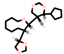
PhEthOH_4235.pdb
