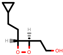
PhEthOH_3085.pdb
