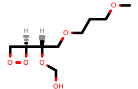
PhEthOH_1875.pdb
