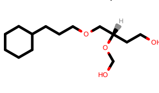
PhEthOH_4470.pdb
