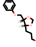
PhEthOH_1814.pdb
