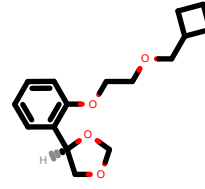
PhEthOH_3562.pdb
