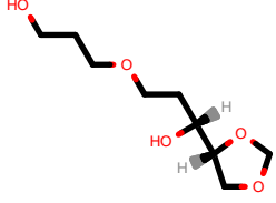
PhEthOH_624.pdb
