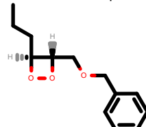
PhEthOH_51.pdb
