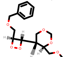
PhEthOH_2109.pdb
