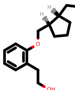
PhEthOH_1608.pdb
