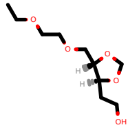
PhEthOH_2288.pdb
