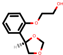
PhEthOH_450.pdb
