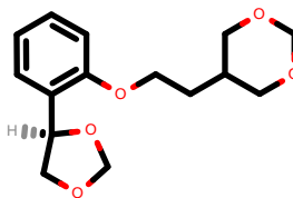
PhEthOH_4692.pdb
