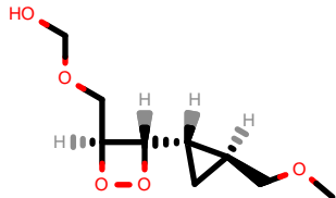
PhEthOH_1957.pdb
