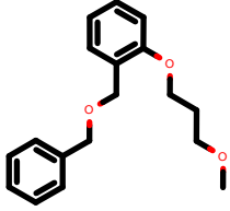
PhEthOH_1732.pdb
