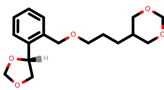
PhEthOH_4777.pdb
