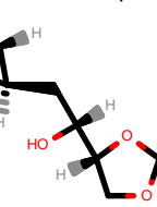
PhEthOH_246.pdb
