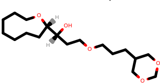
PhEthOH_4910.pdb
