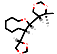
PhEthOH_413.pdb
