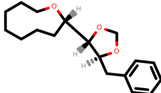
PhEthOH_885.pdb
