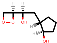
PhEthOH_740.pdb
