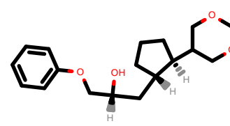
PhEthOH_4999.pdb
