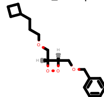
PhEthOH_3625.pdb
