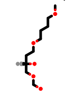
PhEthOH_1914.pdb
