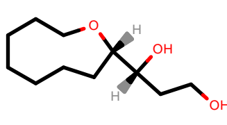
PhEthOH_462.pdb
