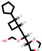
PhEthOH_4149.pdb
