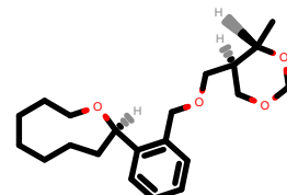
PhEthOH_415.pdb
