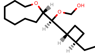
PhEthOH_1597.pdb
