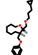
PhEthOH_3197.pdb
