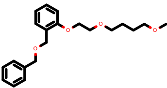
PhEthOH_1896.pdb
