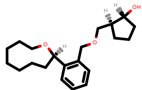
PhEthOH_755.pdb
