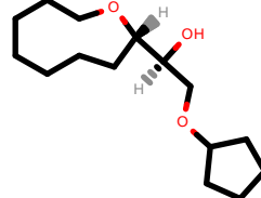
PhEthOH_3902.pdb
