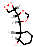
PhEthOH_784.pdb
