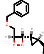
PhEthOH_1525.pdb
