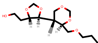
PhEthOH_2956.pdb
