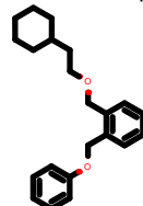
PhEthOH_4246.pdb
