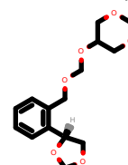
PhEthOH_4735.pdb
