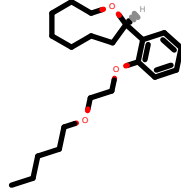
PhEthOH_1510.pdb
