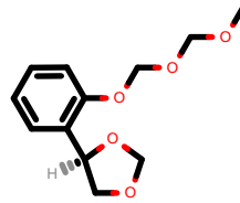
PhEthOH_1794.pdb
