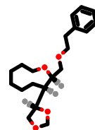
PhEthOH_1047.pdb
