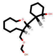
PhEthOH_779.pdb
