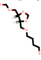
PhEthOH_1916.pdb
