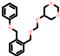
PhEthOH_4708.pdb
