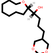
PhEthOH_4784.pdb
