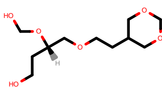
PhEthOH_4844.pdb
