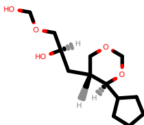
PhEthOH_4220.pdb
