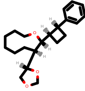
PhEthOH_1173.pdb
