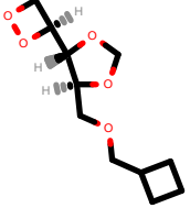
PhEthOH_3560.pdb
