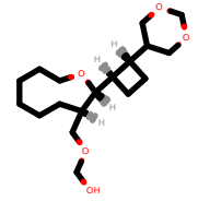
PhEthOH_4983.pdb
