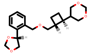
PhEthOH_4991.pdb
