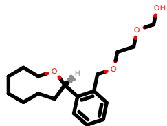
PhEthOH_541.pdb
