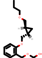
PhEthOH_2794.pdb
