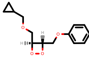
PhEthOH_3115.pdb
