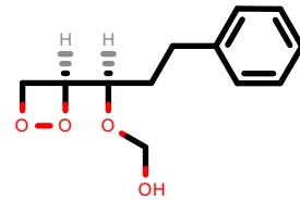
PhEthOH_955.pdb
