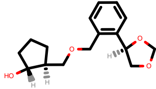
PhEthOH_745.pdb
