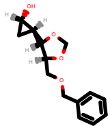
PhEthOH_644.pdb
