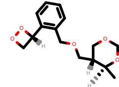
PhEthOH_407.pdb
