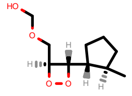
PhEthOH_319.pdb
