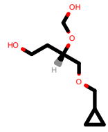
PhEthOH_3126.pdb
