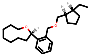
PhEthOH_1633.pdb
