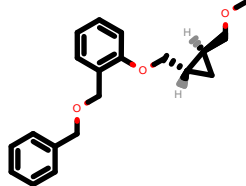
PhEthOH_1942.pdb
