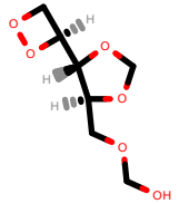
PhEthOH_532.pdb
