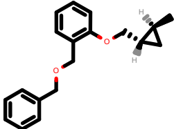
PhEthOH_220.pdb
