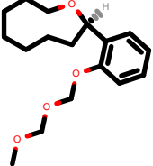
PhEthOH_1804.pdb
