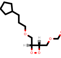
PhEthOH_4057.pdb
