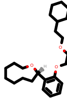
PhEthOH_4446.pdb
