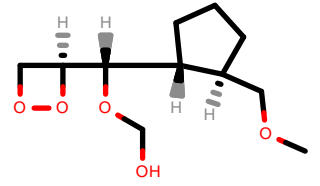
PhEthOH_2047.pdb
