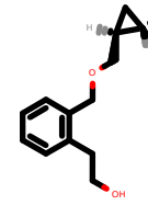
PhEthOH_223.pdb
