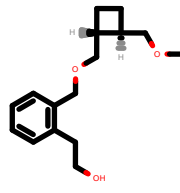
PhEthOH_1991.pdb
