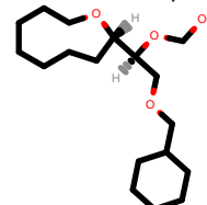
PhEthOH_4407.pdb
