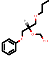
PhEthOH_132.pdb
