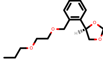
PhEthOH_157.pdb
