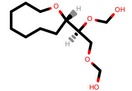
PhEthOH_543.pdb
