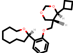
PhEthOH_3820.pdb
