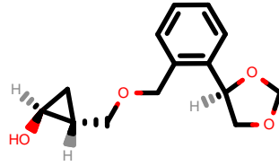
PhEthOH_665.pdb
