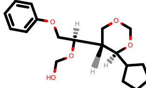
PhEthOH_4206.pdb
