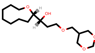
PhEthOH_4830.pdb
