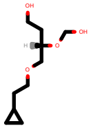
PhEthOH_3164.pdb
