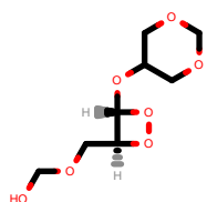
PhEthOH_4725.pdb
