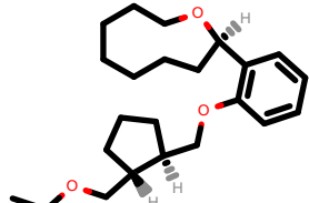
PhEthOH_2472.pdb
