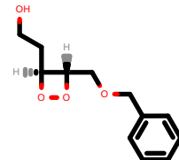
PhEthOH_475.pdb
