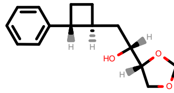
PhEthOH_1170.pdb
