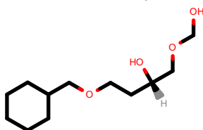
PhEthOH_4388.pdb
