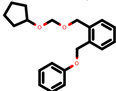
PhEthOH_3868.pdb
