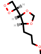
PhEthOH_1834.pdb
