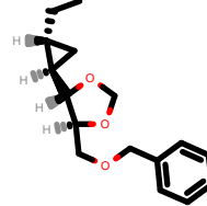
PhEthOH_1526.pdb
