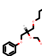
PhEthOH_1434.pdb
