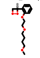
PhEthOH_1918.pdb
