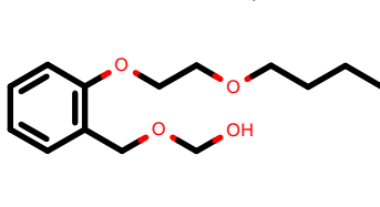
PhEthOH_186.pdb
