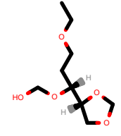
PhEthOH_2175.pdb
