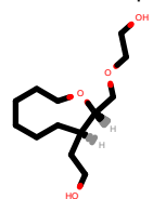
PhEthOH_563.pdb
