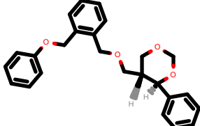
PhEthOH_1264.pdb
