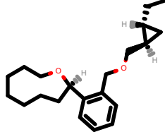
PhEthOH_1553.pdb
