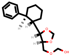
PhEthOH_1240.pdb
