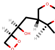
PhEthOH_404.pdb
