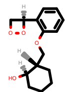
PhEthOH_780.pdb
