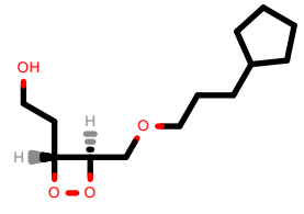
PhEthOH_4051.pdb
