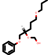
PhEthOH_2652.pdb
