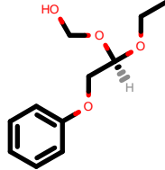
PhEthOH_1350.pdb
