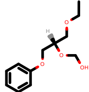
PhEthOH_86.pdb
