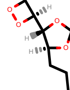
PhEthOH_1334.pdb
