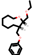
PhEthOH_89.pdb
