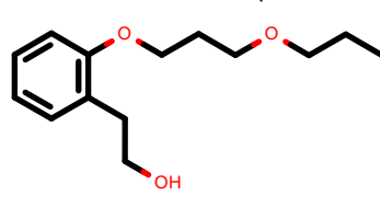
PhEthOH_2578.pdb
