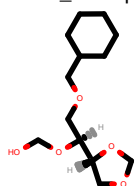
PhEthOH_4401.pdb
