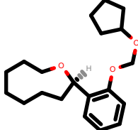
PhEthOH_3900.pdb
