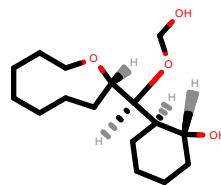
PhEthOH_795.pdb
