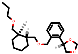
PhEthOH_2933.pdb
