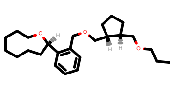
PhEthOH_2897.pdb
