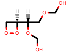
PhEthOH_531.pdb
