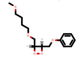
PhEthOH_1897.pdb
