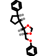
PhEthOH_1180.pdb
