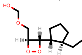
PhEthOH_1617.pdb
