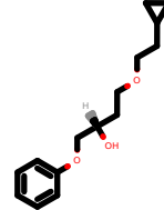
PhEthOH_3155.pdb
