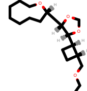
PhEthOH_2435.pdb
