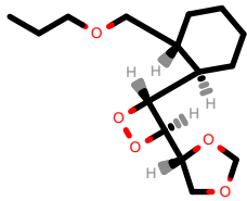
PhEthOH_2936.pdb
