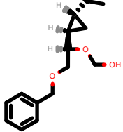
PhEthOH_1524.pdb
