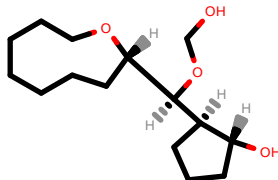
PhEthOH_757.pdb
