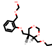
PhEthOH_2538.pdb
