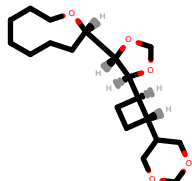
PhEthOH_4997.pdb
