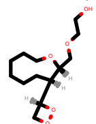
PhEthOH_575.pdb
