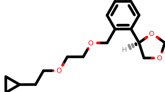
PhEthOH_3185.pdb
