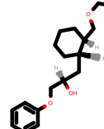
PhEthOH_2479.pdb
