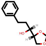
PhEthOH_876.pdb
