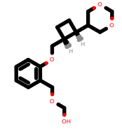
PhEthOH_4978.pdb
