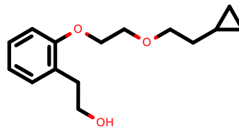
PhEthOH_3166.pdb
