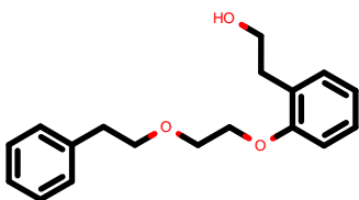
PhEthOH_1020.pdb
