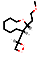
PhEthOH_1755.pdb
