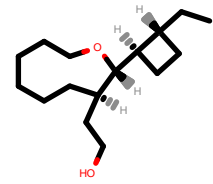
PhEthOH_1575.pdb
