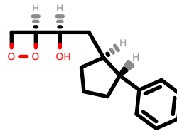
PhEthOH_1206.pdb
