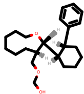
PhEthOH_1241.pdb
