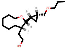
PhEthOH_2793.pdb
