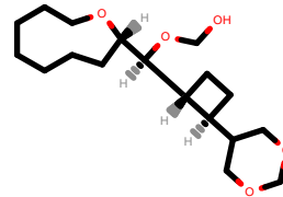
PhEthOH_4995.pdb
