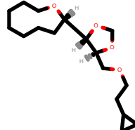
PhEthOH_3195.pdb
