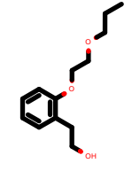
PhEthOH_142.pdb
