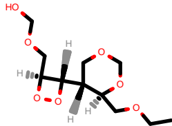
PhEthOH_2541.pdb
