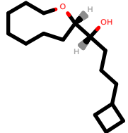
PhEthOH_3528.pdb
