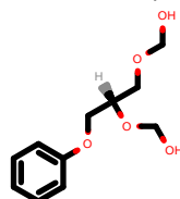
PhEthOH_506.pdb
