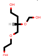
PhEthOH_560.pdb
