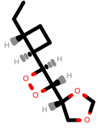
PhEthOH_1592.pdb
