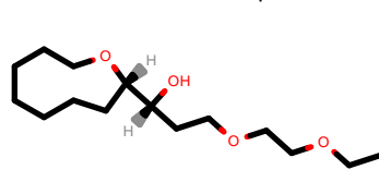
PhEthOH_2306.pdb
