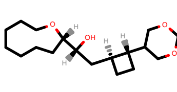
PhEthOH_4994.pdb
