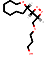
PhEthOH_632.pdb
