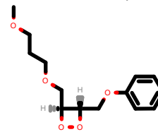
PhEthOH_1855.pdb
