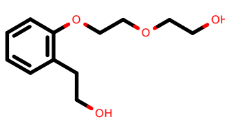
PhEthOH_562.pdb
