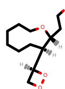
PhEthOH_491.pdb
