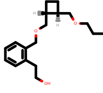
PhEthOH_2831.pdb
