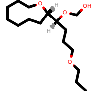
PhEthOH_2685.pdb
