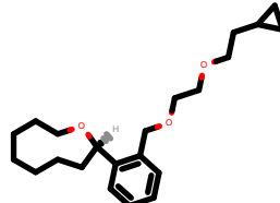
PhEthOH_3191.pdb
