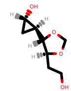
PhEthOH_650.pdb
