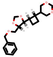
PhEthOH_4970.pdb
