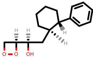
PhEthOH_1244.pdb
