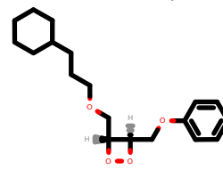
PhEthOH_4459.pdb
