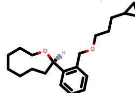
PhEthOH_3103.pdb
