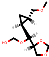
PhEthOH_1969.pdb
