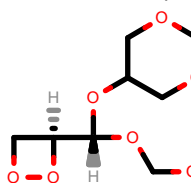
PhEthOH_4735.pdb
