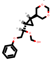
PhEthOH_4920.pdb
