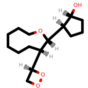
PhEthOH_743.pdb
