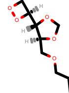
PhEthOH_1418.pdb
