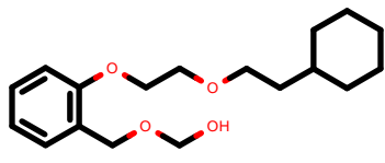
PhEthOH_4432.pdb
