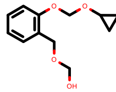
PhEthOH_3046.pdb
