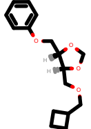
PhEthOH_3536.pdb
