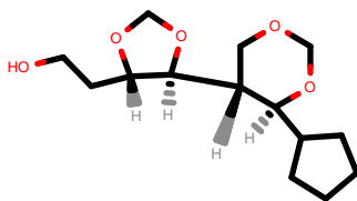
PhEthOH_4220.pdb
