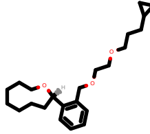
PhEthOH_3229.pdb
