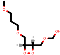
PhEthOH_1869.pdb
