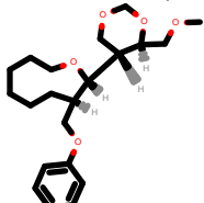
PhEthOH_2109.pdb
