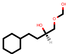
PhEthOH_4266.pdb
