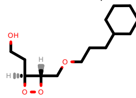
PhEthOH_4471.pdb
