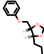
PhEthOH_46.pdb
