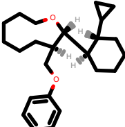
PhEthOH_3327.pdb
