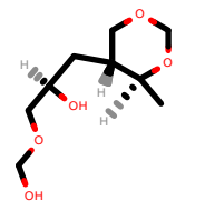
PhEthOH_402.pdb
