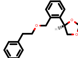
PhEthOH_875.pdb
