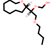
PhEthOH_211.pdb
