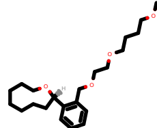
PhEthOH_1931.pdb
