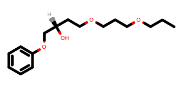
PhEthOH_2735.pdb
