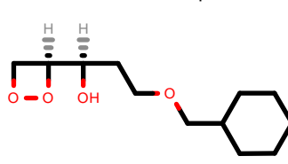
PhEthOH_4394.pdb
