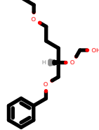
PhEthOH_2238.pdb
