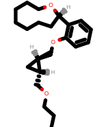
PhEthOH_2812.pdb
