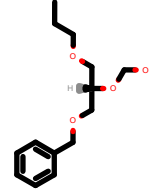
PhEthOH_138.pdb
