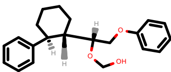
PhEthOH_1220.pdb
