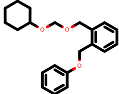
PhEthOH_4284.pdb
