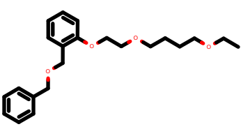
PhEthOH_2320.pdb
