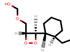
PhEthOH_1659.pdb
