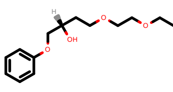
PhEthOH_2269.pdb
