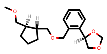
PhEthOH_2047.pdb
