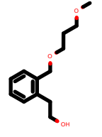
PhEthOH_1739.pdb
