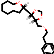
PhEthOH_1053.pdb
