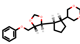
PhEthOH_5006.pdb
