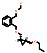
PhEthOH_2795.pdb
