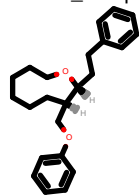
PhEthOH_933.pdb
