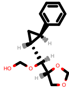
PhEthOH_1129.pdb
