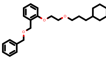
PhEthOH_4462.pdb
