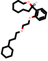
PhEthOH_4492.pdb
