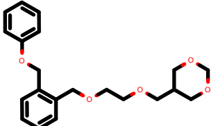
PhEthOH_4788.pdb
