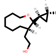
PhEthOH_231.pdb
