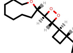
PhEthOH_1598.pdb
