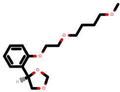
PhEthOH_1920.pdb
