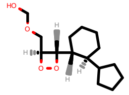
PhEthOH_4183.pdb
