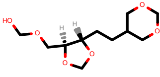
PhEthOH_4772.pdb
