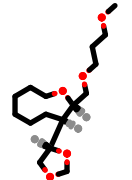
PhEthOH_1883.pdb
