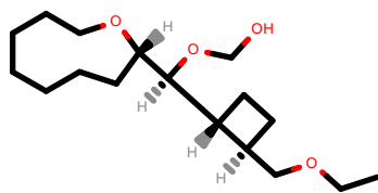
PhEthOH_2433.pdb
