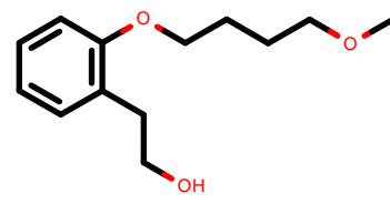
PhEthOH_1822.pdb
