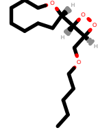
PhEthOH_1514.pdb
