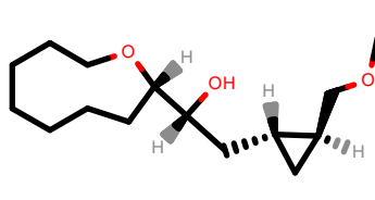
PhEthOH_1974.pdb
