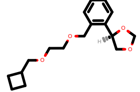
PhEthOH_3563.pdb
