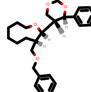
PhEthOH_1271.pdb
