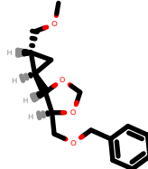
PhEthOH_1946.pdb
