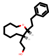
PhEthOH_945.pdb
