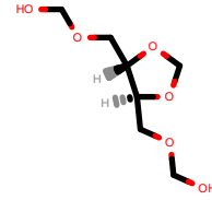
PhEthOH_530.pdb
