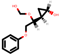
PhEthOH_636.pdb
