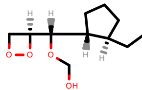
PhEthOH_1623.pdb
