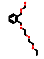
PhEthOH_2291.pdb
