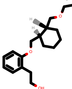
PhEthOH_2490.pdb
