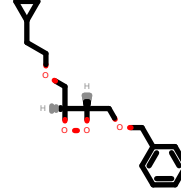
PhEthOH_3163.pdb
