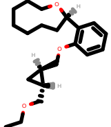
PhEthOH_2392.pdb
