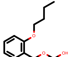
PhEthOH_60.pdb
