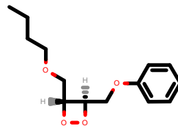
PhEthOH_171.pdb
