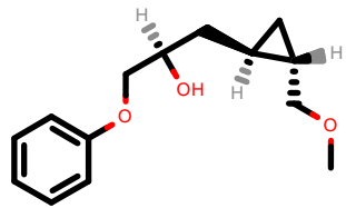
PhEthOH_1937.pdb
