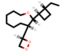
PhEthOH_1587.pdb
