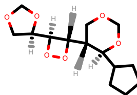
PhEthOH_4234.pdb
