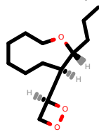
PhEthOH_71.pdb
