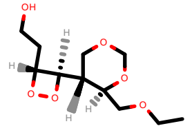
PhEthOH_2535.pdb
