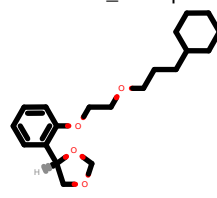
PhEthOH_4486.pdb
