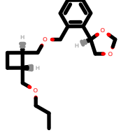
PhEthOH_2845.pdb
