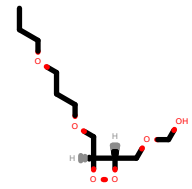
PhEthOH_2751.pdb
