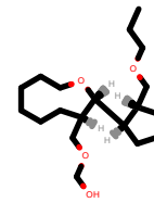
PhEthOH_2879.pdb
