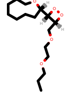
PhEthOH_2732.pdb
