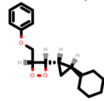
PhEthOH_4501.pdb
