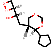
PhEthOH_4230.pdb
