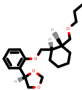
PhEthOH_2932.pdb
