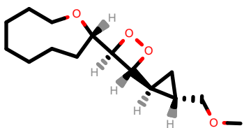
PhEthOH_1976.pdb
