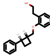
PhEthOH_1150.pdb
