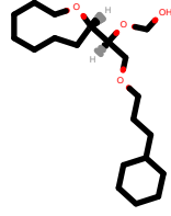
PhEthOH_4495.pdb
