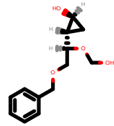
PhEthOH_638.pdb
