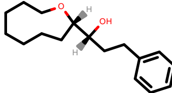
PhEthOH_882.pdb
