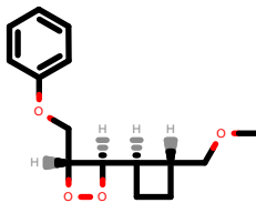
PhEthOH_1981.pdb
