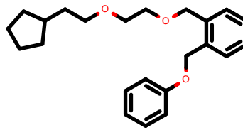
PhEthOH_3990.pdb
