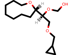
PhEthOH_3151.pdb
