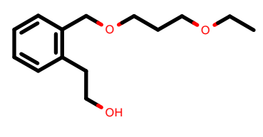
PhEthOH_2159.pdb
