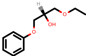
PhEthOH_1349.pdb
