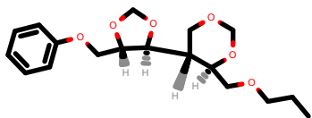
PhEthOH_2944.pdb
