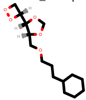
PhEthOH_4484.pdb
