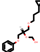
PhEthOH_3198.pdb
