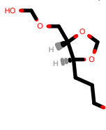
PhEthOH_1832.pdb
