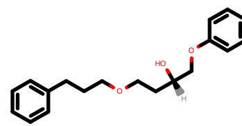
PhEthOH_1055.pdb
