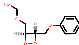
PhEthOH_507.pdb
