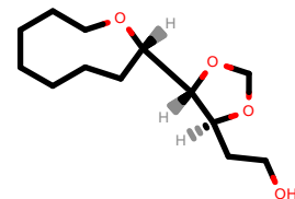
PhEthOH_503.pdb
