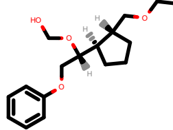
PhEthOH_2442.pdb
