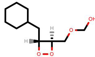
PhEthOH_4267.pdb
