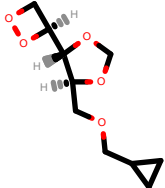
PhEthOH_3140.pdb
