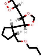
PhEthOH_2888.pdb
