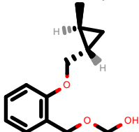
PhEthOH_232.pdb
