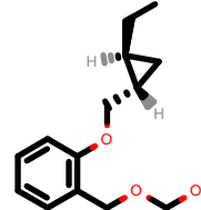
PhEthOH_1534.pdb
