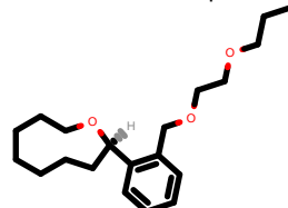
PhEthOH_163.pdb
