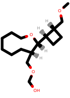
PhEthOH_2001.pdb
