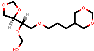
PhEthOH_4909.pdb
