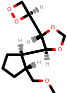
PhEthOH_2044.pdb
