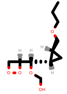
PhEthOH_2803.pdb
