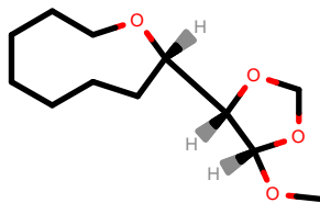
PhEthOH_41.pdb
