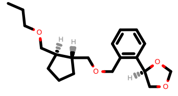
PhEthOH_2891.pdb
