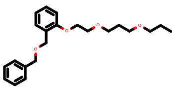
PhEthOH_2740.pdb
