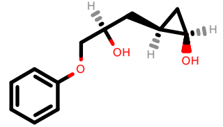
PhEthOH_635.pdb
