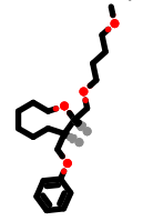
PhEthOH_1899.pdb
