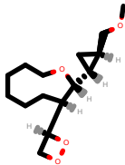
PhEthOH_1965.pdb
