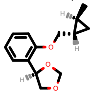
PhEthOH_244.pdb
