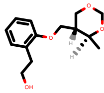
PhEthOH_394.pdb
