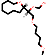
PhEthOH_1933.pdb
