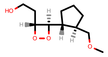
PhEthOH_2035.pdb
