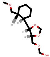
PhEthOH_2080.pdb
