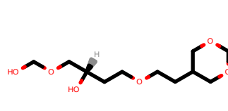
PhEthOH_4850.pdb
