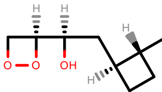
PhEthOH_278.pdb
