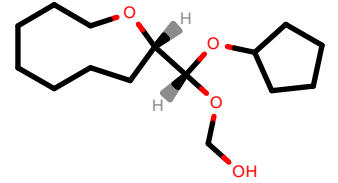
PhEthOH_3903.pdb
