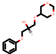
PhEthOH_4709.pdb
