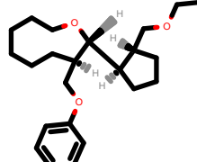
PhEthOH_2445.pdb
