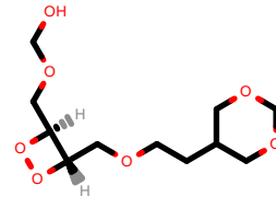
PhEthOH_4855.pdb
