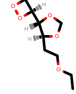
PhEthOH_2174.pdb
