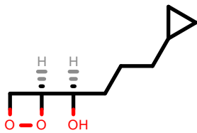
PhEthOH_3096.pdb
