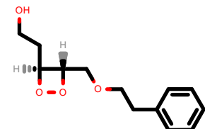
PhEthOH_1023.pdb
