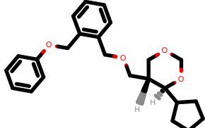
PhEthOH_4204.pdb
