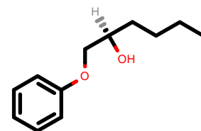
PhEthOH_43.pdb
