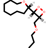
PhEthOH_1430.pdb
