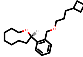
PhEthOH_3527.pdb
