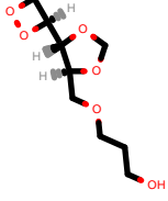
PhEthOH_620.pdb
