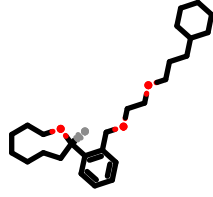
PhEthOH_4493.pdb
