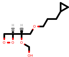
PhEthOH_3219.pdb
