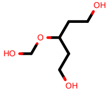
PhEthOH_476.pdb
