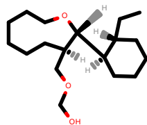
PhEthOH_1661.pdb
