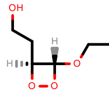
PhEthOH_1363.pdb
