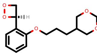
PhEthOH_4770.pdb
