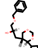
PhEthOH_4207.pdb
