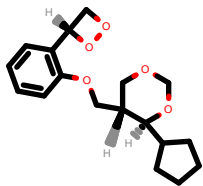
PhEthOH_4228.pdb
