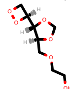
PhEthOH_574.pdb
