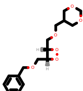
PhEthOH_4797.pdb
