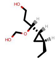
PhEthOH_1530.pdb
