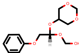
PhEthOH_4710.pdb
