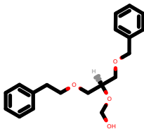
PhEthOH_1020.pdb
