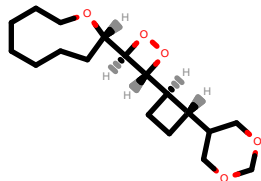
PhEthOH_4996.pdb
