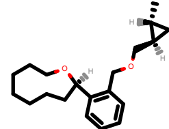
PhEthOH_251.pdb
