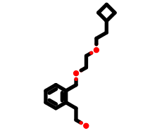
PhEthOH_3583.pdb
