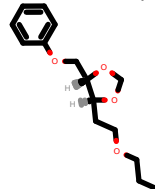
PhEthOH_2570.pdb
