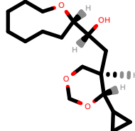
PhEthOH_3402.pdb
