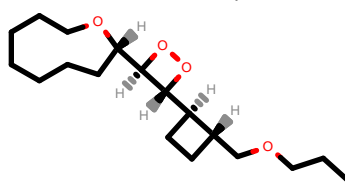
PhEthOH_2858.pdb
