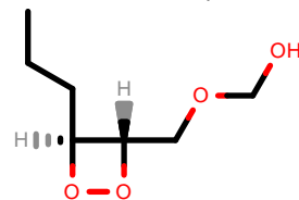
PhEthOH_63.pdb
