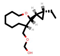
PhEthOH_1535.pdb
