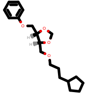
PhEthOH_4040.pdb
