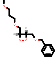
PhEthOH_1861.pdb
