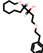
PhEthOH_1050.pdb
