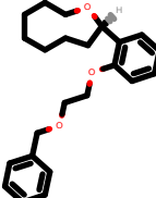
PhEthOH_1006.pdb
