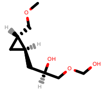
PhEthOH_1956.pdb
