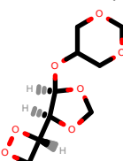
PhEthOH_4732.pdb
