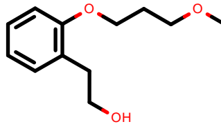
PhEthOH_1738.pdb
