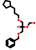
PhEthOH_4044.pdb
