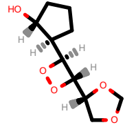
PhEthOH_752.pdb
