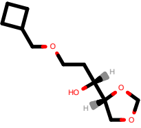
PhEthOH_3564.pdb
