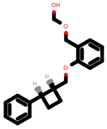
PhEthOH_1156.pdb
