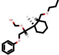
PhEthOH_2904.pdb
