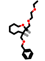
PhEthOH_2283.pdb
