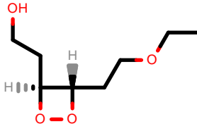
PhEthOH_2161.pdb
