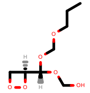
PhEthOH_2635.pdb
