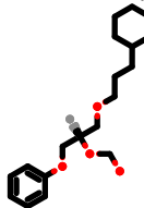
PhEthOH_4458.pdb
