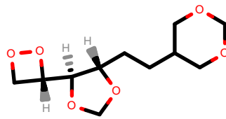
PhEthOH_4778.pdb
