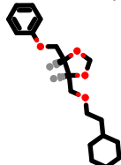
PhEthOH_4414.pdb
