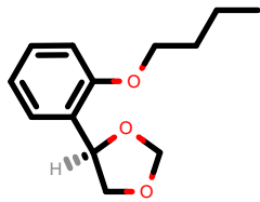
PhEthOH_72.pdb
