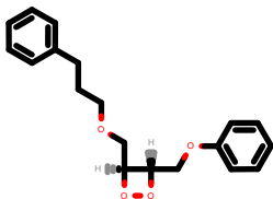
PhEthOH_1053.pdb
