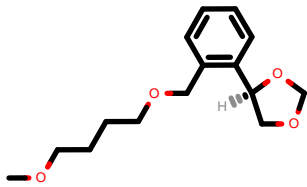
PhEthOH_1841.pdb
