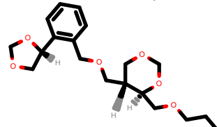
PhEthOH_2971.pdb
