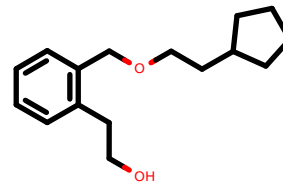
PhEthOH_3839.pdb
