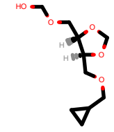
PhEthOH_3134.pdb
