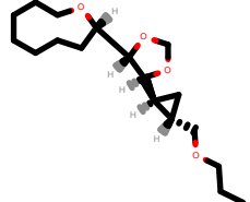
PhEthOH_2813.pdb
