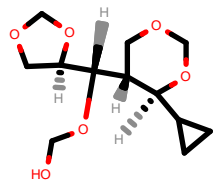
PhEthOH_3397.pdb
