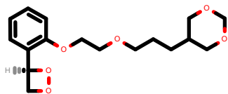
PhEthOH_4900.pdb
