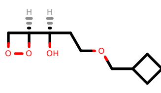
PhEthOH_3558.pdb
