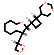
PhEthOH_4989.pdb
