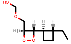
PhEthOH_1579.pdb
