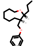
PhEthOH_47.pdb
