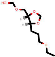
PhEthOH_2252.pdb
