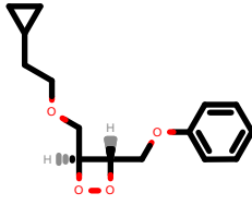
PhEthOH_3157.pdb
