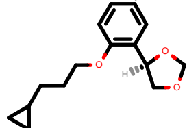
PhEthOH_3100.pdb
