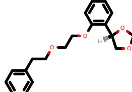
PhEthOH_1042.pdb
