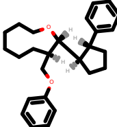
PhEthOH_1181.pdb
