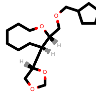
PhEthOH_3987.pdb
