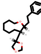
PhEthOH_959.pdb
