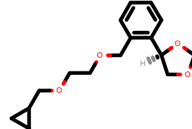
PhEthOH_3143.pdb
