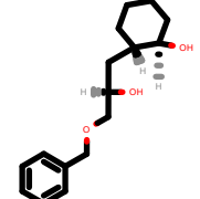
PhEthOH_767.pdb
