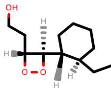
PhEthOH_1653.pdb
