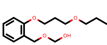
PhEthOH_2580.pdb
