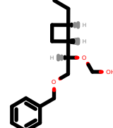
PhEthOH_1566.pdb
