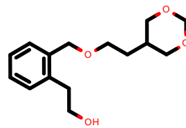
PhEthOH_4679.pdb
