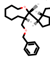
PhEthOH_1611.pdb
