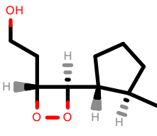
PhEthOH_313.pdb
