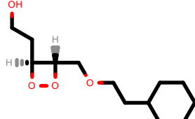
PhEthOH_4429.pdb
