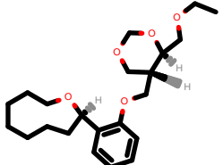
PhEthOH_2556.pdb
