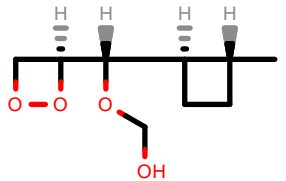
PhEthOH_279.pdb
