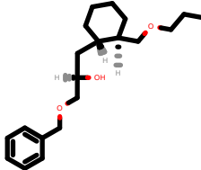
PhEthOH_2909.pdb
