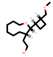
PhEthOH_1995.pdb
