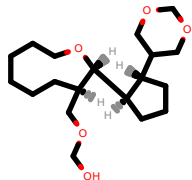
PhEthOH_5021.pdb
