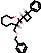
PhEthOH_1149.pdb
