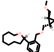
PhEthOH_1973.pdb
