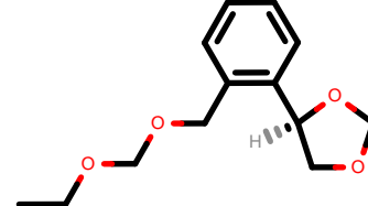
PhEthOH_1375.pdb
