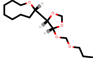
PhEthOH_2649.pdb
