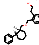
PhEthOH_1235.pdb
