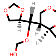
PhEthOH_415.pdb
