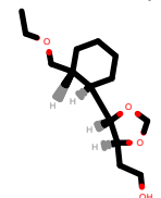
PhEthOH_2494.pdb
