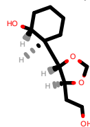
PhEthOH_772.pdb
