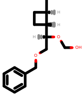
PhEthOH_264.pdb
