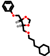
PhEthOH_4460.pdb
