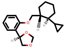
PhEthOH_3348.pdb
