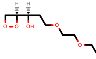
PhEthOH_2298.pdb
