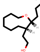
PhEthOH_59.pdb
