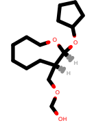
PhEthOH_3891.pdb
