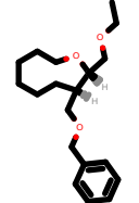
PhEthOH_95.pdb
