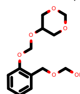
PhEthOH_4722.pdb
