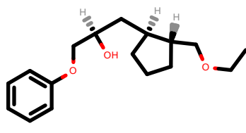
PhEthOH_2441.pdb
