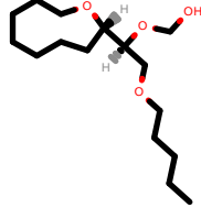
PhEthOH_1513.pdb
