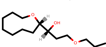
PhEthOH_164.pdb
