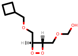
PhEthOH_3549.pdb
