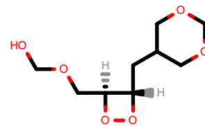
PhEthOH_4687.pdb
