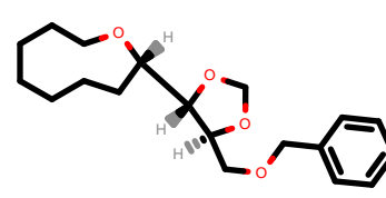
PhEthOH_1007.pdb
