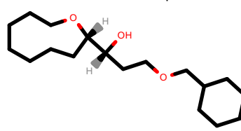
PhEthOH_4406.pdb
