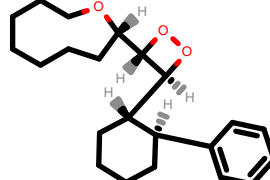
PhEthOH_1258.pdb
