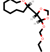
PhEthOH_2229.pdb
