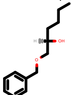
PhEthOH_49.pdb
