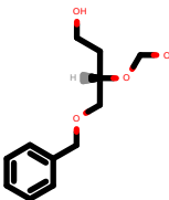
PhEthOH_474.pdb
