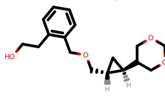
PhEthOH_4927.pdb
