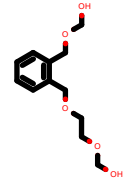
PhEthOH_523.pdb
