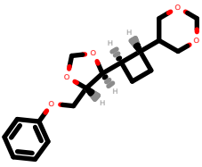
PhEthOH_4964.pdb
