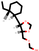
PhEthOH_1660.pdb
