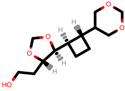
PhEthOH_4976.pdb
