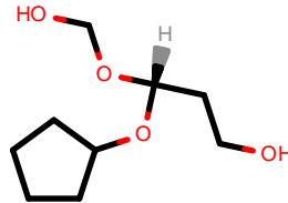
PhEthOH_3882.pdb
