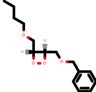
PhEthOH_1437.pdb
