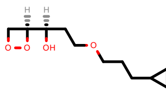
PhEthOH_3222.pdb
