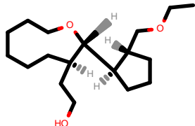
PhEthOH_2453.pdb
