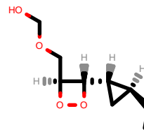
PhEthOH_1533.pdb
