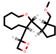
PhEthOH_2045.pdb
