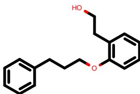
PhEthOH_936.pdb
