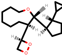
PhEthOH_3309.pdb
