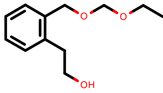
PhEthOH_1361.pdb
