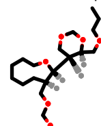
PhEthOH_2963.pdb
