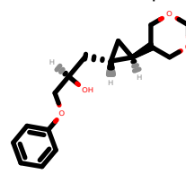
PhEthOH_4919.pdb
