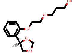
PhEthOH_622.pdb
