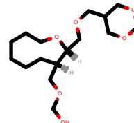
PhEthOH_4811.pdb
