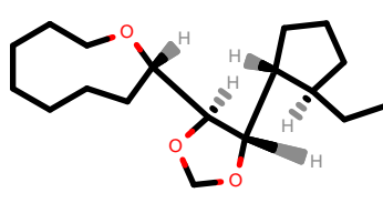
PhEthOH_1641.pdb
