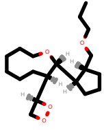
PhEthOH_2889.pdb
