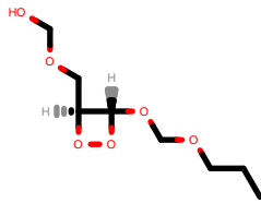
PhEthOH_2629.pdb
