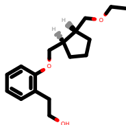
PhEthOH_2448.pdb
