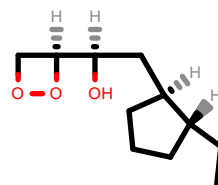
PhEthOH_1622.pdb
