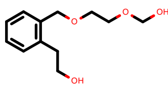
PhEthOH_517.pdb
