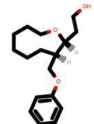
PhEthOH_471.pdb
