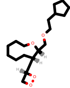
PhEthOH_4023.pdb
