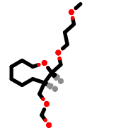
PhEthOH_1871.pdb
