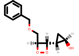
PhEthOH_639.pdb
