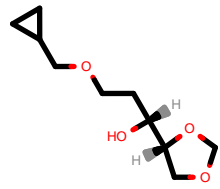
PhEthOH_3144.pdb
