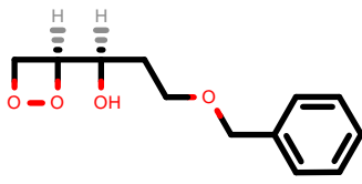
PhEthOH_996.pdb
