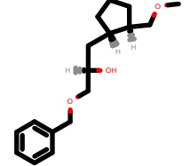
PhEthOH_2027.pdb
