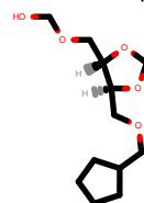
PhEthOH_3970.pdb
