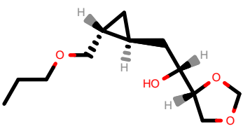
PhEthOH_2804.pdb
