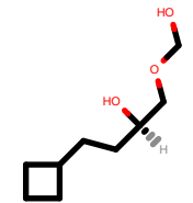
PhEthOH_3422.pdb
