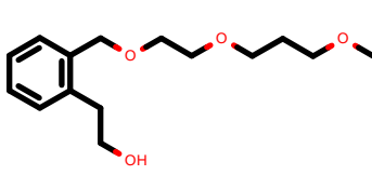
PhEthOH_1861.pdb
