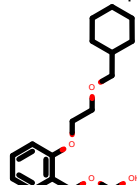
PhEthOH_4386.pdb
