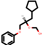
PhEthOH_3828.pdb
