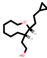
PhEthOH_3087.pdb
