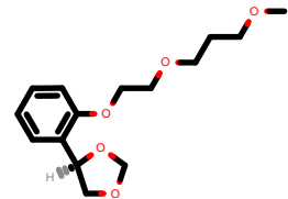
PhEthOH_1878.pdb
