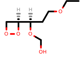
PhEthOH_2173.pdb
