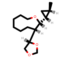
PhEthOH_249.pdb
