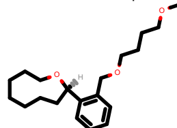
PhEthOH_1847.pdb
