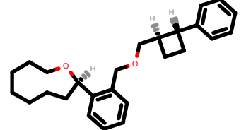
PhEthOH_1175.pdb
