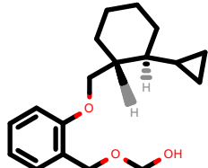
PhEthOH_3336.pdb
