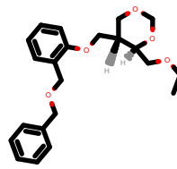
PhEthOH_2526.pdb
