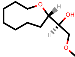
PhEthOH_42.pdb
