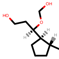
PhEthOH_312.pdb
