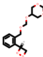
PhEthOH_4733.pdb
