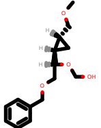
PhEthOH_1944.pdb
