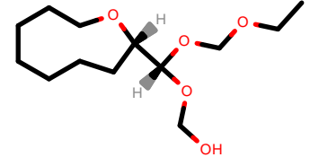
PhEthOH_2227.pdb
