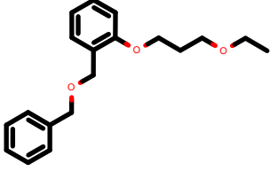
PhEthOH_2152.pdb
