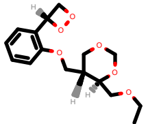
PhEthOH_2544.pdb
