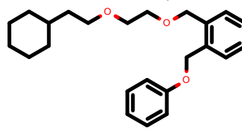
PhEthOH_4410.pdb
