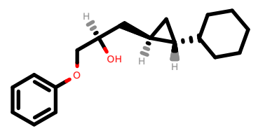
PhEthOH_4499.pdb
