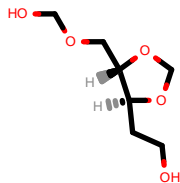
PhEthOH_484.pdb
