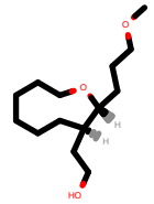
PhEthOH_1823.pdb
