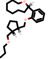
PhEthOH_2896.pdb
