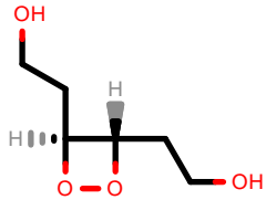
PhEthOH_477.pdb
