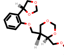
PhEthOH_2550.pdb
