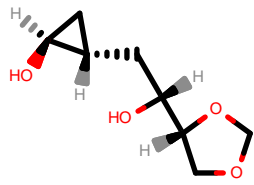
PhEthOH_666.pdb
