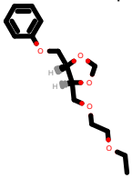
PhEthOH_2276.pdb
