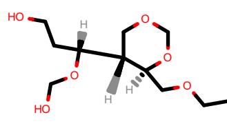
PhEthOH_2534.pdb
