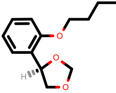
PhEthOH_1336.pdb
