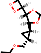
PhEthOH_2384.pdb
