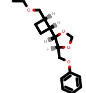
PhEthOH_2398.pdb
