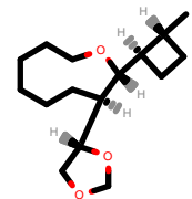
PhEthOH_287.pdb
