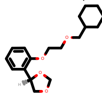
PhEthOH_4398.pdb
