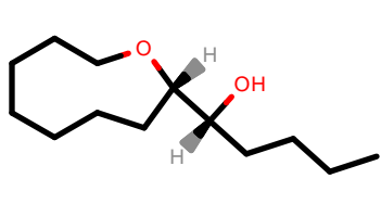
PhEthOH_80.pdb
