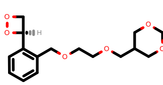
PhEthOH_4813.pdb
