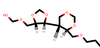
PhEthOH_2962.pdb
