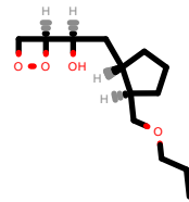
PhEthOH_2882.pdb
