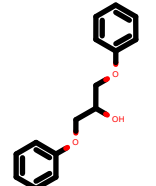
PhEthOH_887.pdb
