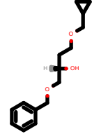
PhEthOH_3119.pdb
