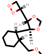
PhEthOH_2086.pdb
