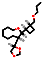
PhEthOH_2853.pdb
