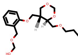
PhEthOH_2958.pdb
