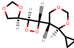
PhEthOH_3398.pdb
