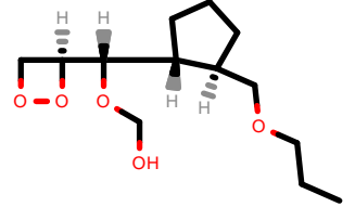
PhEthOH_2887.pdb
