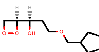
PhEthOH_3974.pdb
