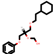
PhEthOH_4412.pdb
