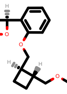
PhEthOH_2002.pdb
