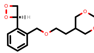
PhEthOH_4691.pdb
