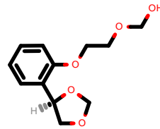
PhEthOH_534.pdb
