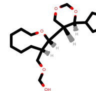
PhEthOH_4223.pdb
