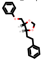
PhEthOH_932.pdb
