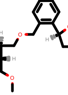
PhEthOH_2009.pdb
