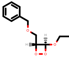
PhEthOH_1357.pdb
