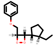
PhEthOH_1599.pdb
