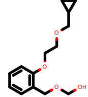
PhEthOH_3130.pdb
