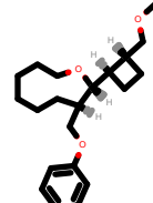
PhEthOH_1983.pdb
