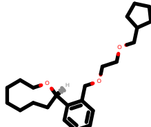
PhEthOH_3985.pdb
