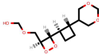
PhEthOH_4981.pdb
