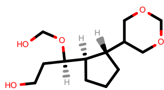
PhEthOH_5012.pdb
