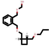
PhEthOH_2837.pdb
