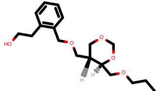
PhEthOH_2957.pdb
