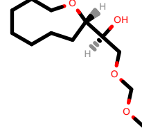
PhEthOH_1806.pdb
