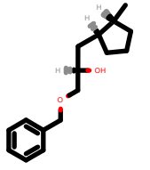
PhEthOH_305.pdb
