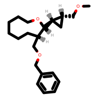
PhEthOH_1947.pdb
