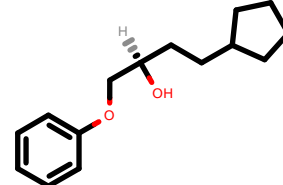
PhEthOH_3827.pdb
