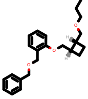
PhEthOH_2824.pdb
