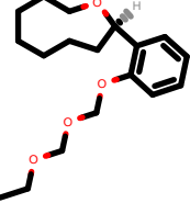
PhEthOH_2224.pdb
