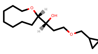
PhEthOH_3150.pdb
