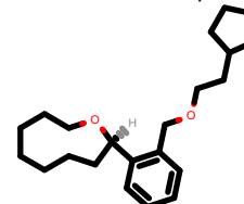
PhEthOH_3863.pdb
