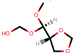
PhEthOH_33.pdb
