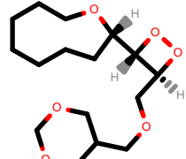
PhEthOH_4828.pdb
