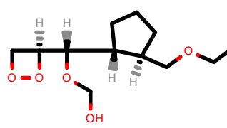
PhEthOH_2463.pdb
