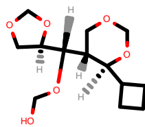
PhEthOH_3817.pdb
