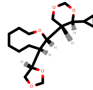
PhEthOH_3399.pdb
