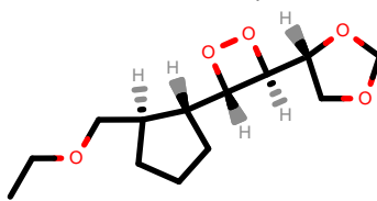
PhEthOH_2470.pdb
