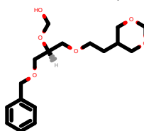
PhEthOH_4838.pdb
