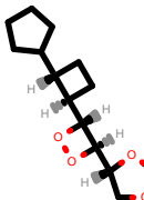
PhEthOH_4150.pdb
