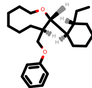
PhEthOH_1647.pdb
