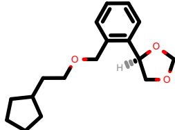
PhEthOH_3857.pdb
