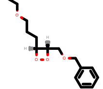
PhEthOH_2239.pdb
