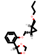
PhEthOH_2806.pdb
