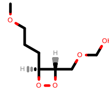
PhEthOH_1827.pdb
