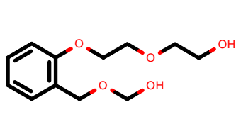
PhEthOH_564.pdb
