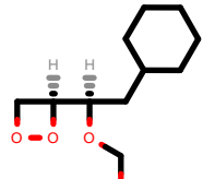
PhEthOH_4269.pdb
