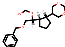
PhEthOH_5010.pdb
