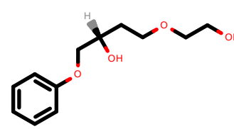
PhEthOH_551.pdb
