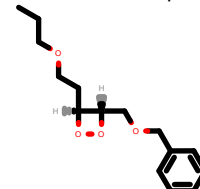
PhEthOH_2575.pdb
