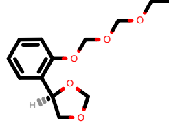
PhEthOH_2218.pdb
