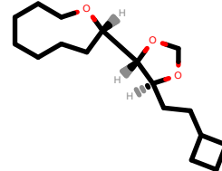
PhEthOH_3531.pdb
