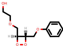
PhEthOH_553.pdb
