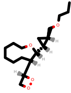
PhEthOH_2805.pdb
