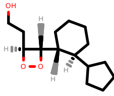
PhEthOH_4177.pdb
