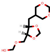
PhEthOH_4688.pdb
