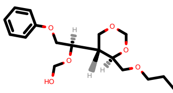
PhEthOH_2942.pdb
