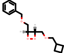
PhEthOH_3541.pdb
