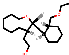
PhEthOH_2495.pdb
