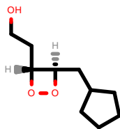
PhEthOH_3837.pdb
