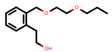
PhEthOH_139.pdb
