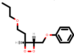
PhEthOH_2569.pdb
