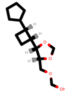
PhEthOH_4142.pdb
