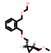
PhEthOH_1951.pdb
