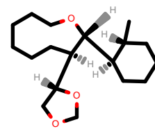
PhEthOH_375.pdb
