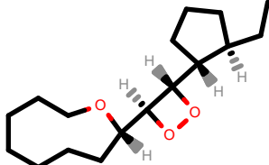
PhEthOH_1640.pdb
