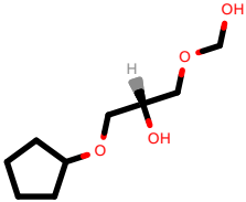
PhEthOH_3888.pdb
