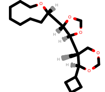
PhEthOH_3825.pdb
