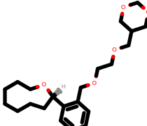
PhEthOH_4829.pdb
