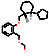
PhEthOH_4180.pdb
