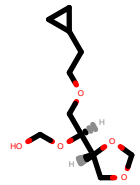
PhEthOH_3187.pdb
