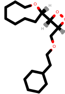
PhEthOH_4454.pdb
