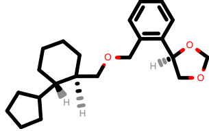
PhEthOH_4189.pdb
