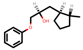
PhEthOH_299.pdb
