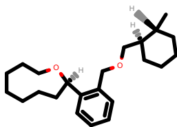
PhEthOH_377.pdb
