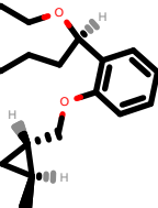
PhEthOH_250.pdb
