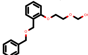
PhEthOH_510.pdb
