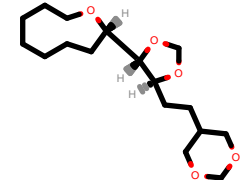
PhEthOH_4787.pdb
