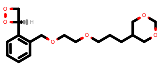
PhEthOH_4901.pdb
