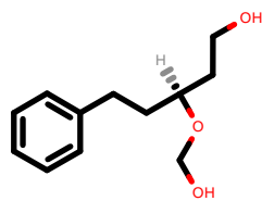
PhEthOH_938.pdb
