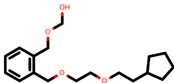
PhEthOH_4013.pdb
