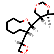
PhEthOH_407.pdb
