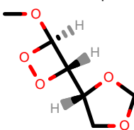
PhEthOH_34.pdb
