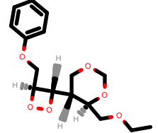
PhEthOH_2527.pdb
