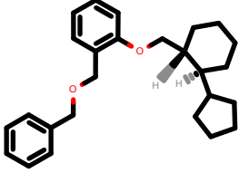
PhEthOH_4168.pdb
