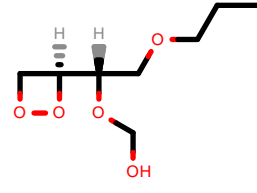
PhEthOH_157.pdb
