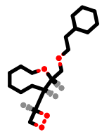
PhEthOH_4443.pdb
