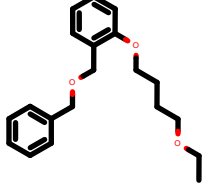
PhEthOH_2236.pdb
