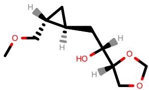
PhEthOH_1968.pdb
