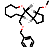
PhEthOH_2451.pdb
