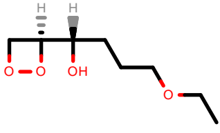
PhEthOH_2172.pdb
