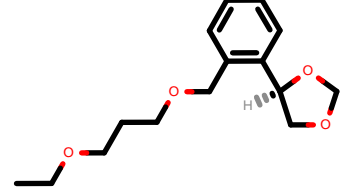
PhEthOH_2173.pdb
