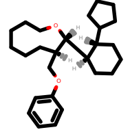
PhEthOH_4167.pdb
