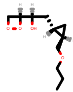
PhEthOH_2802.pdb
