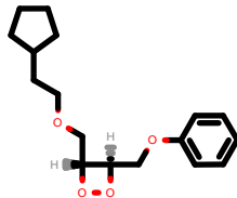
PhEthOH_3997.pdb
