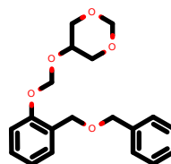
PhEthOH_4714.pdb
