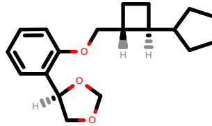
PhEthOH_4150.pdb
