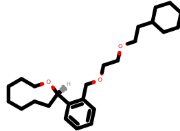
PhEthOH_4447.pdb
