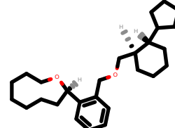
PhEthOH_4199.pdb
