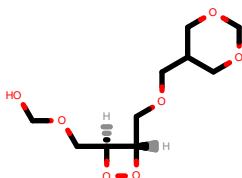
PhEthOH_4809.pdb
