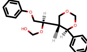
PhEthOH_1266.pdb
