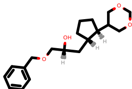
PhEthOH_5009.pdb
