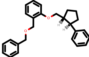
PhEthOH_1182.pdb
