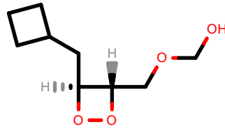
PhEthOH_3423.pdb
