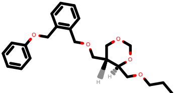
PhEthOH_2940.pdb
