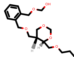
PhEthOH_2959.pdb
