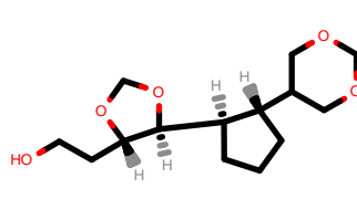
PhEthOH_5014.pdb
