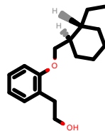
PhEthOH_1650.pdb
