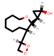
PhEthOH_663.pdb
