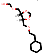
PhEthOH_4436.pdb
