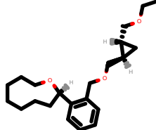
PhEthOH_2393.pdb
