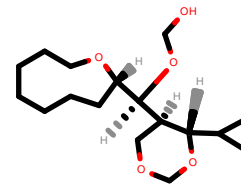
PhEthOH_3403.pdb
