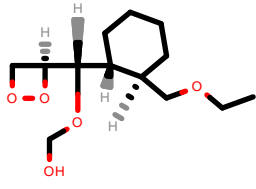
PhEthOH_2509.pdb
