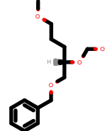
PhEthOH_1818.pdb
