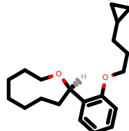
PhEthOH_3102.pdb
