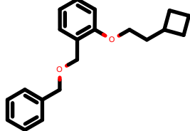
PhEthOH_3412.pdb
