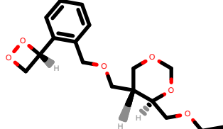
PhEthOH_2545.pdb
