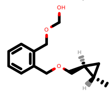
PhEthOH_233.pdb
