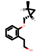
PhEthOH_222.pdb
