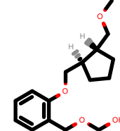
PhEthOH_2038.pdb
