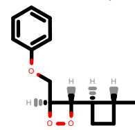
PhEthOH_255.pdb
