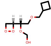
PhEthOH_3559.pdb
