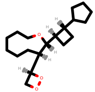
PhEthOH_4149.pdb
