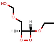
PhEthOH_1369.pdb
