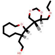
PhEthOH_2537.pdb
