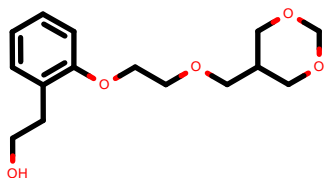
PhEthOH_4804.pdb
