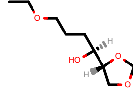
PhEthOH_2174.pdb
