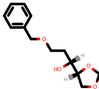
PhEthOH_1002.pdb
