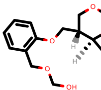
PhEthOH_400.pdb
