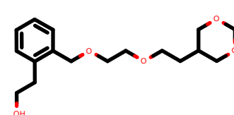
PhEthOH_4843.pdb
