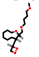
PhEthOH_1919.pdb
