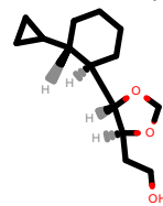
PhEthOH_3334.pdb
