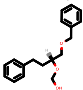
PhEthOH_932.pdb
