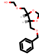
PhEthOH_518.pdb
