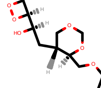
PhEthOH_2546.pdb
