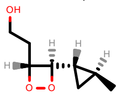
PhEthOH_229.pdb
