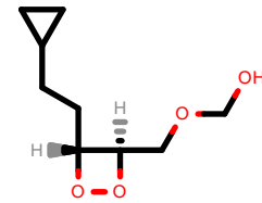
PhEthOH_3091.pdb
