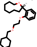
PhEthOH_4404.pdb
