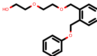
PhEthOH_550.pdb
