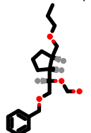
PhEthOH_2864.pdb
