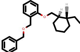
PhEthOH_1648.pdb
