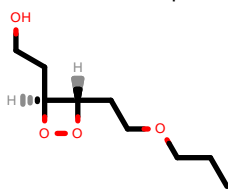
PhEthOH_2581.pdb
