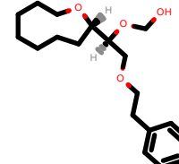
PhEthOH_1051.pdb
