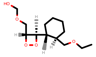
PhEthOH_2503.pdb
