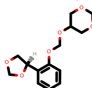
PhEthOH_4734.pdb
