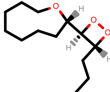
PhEthOH_82.pdb
