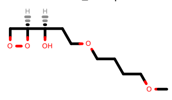
PhEthOH_1916.pdb
