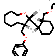
PhEthOH_2483.pdb
