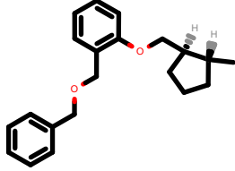
PhEthOH_304.pdb
