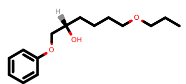
PhEthOH_2647.pdb
