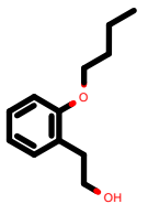
PhEthOH_54.pdb
