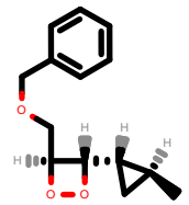
PhEthOH_223.pdb
