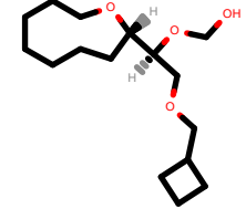
PhEthOH_3571.pdb
