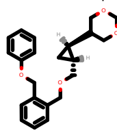
PhEthOH_4918.pdb
