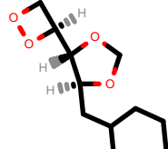
PhEthOH_4270.pdb
