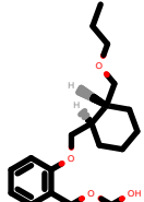
PhEthOH_2920.pdb
