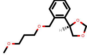
PhEthOH_1757.pdb
