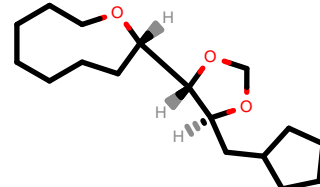
PhEthOH_3867.pdb
