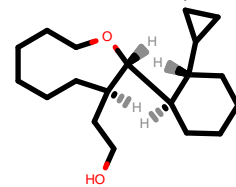
PhEthOH_3335.pdb
