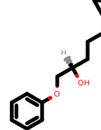
PhEthOH_3071.pdb
