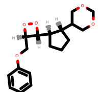
PhEthOH_5005.pdb
