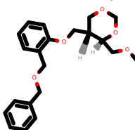
PhEthOH_2110.pdb
