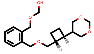
PhEthOH_4979.pdb
