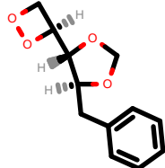
PhEthOH_872.pdb
