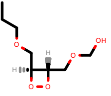
PhEthOH_151.pdb
