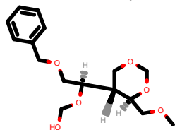
PhEthOH_2108.pdb
