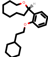
PhEthOH_4282.pdb
