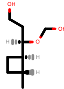
PhEthOH_266.pdb
