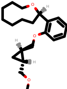
PhEthOH_1972.pdb
