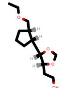
PhEthOH_2452.pdb
