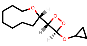
PhEthOH_3068.pdb
