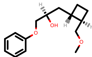
PhEthOH_1979.pdb
