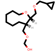
PhEthOH_3135.pdb
