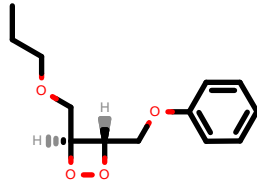
PhEthOH_133.pdb
