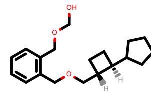
PhEthOH_4139.pdb
