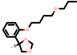
PhEthOH_2680.pdb
