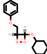
PhEthOH_4287.pdb
