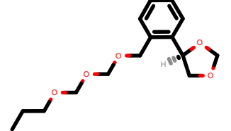
PhEthOH_2639.pdb
