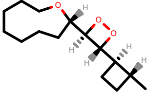
PhEthOH_296.pdb
