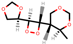
PhEthOH_412.pdb
