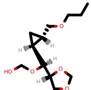
PhEthOH_2805.pdb
