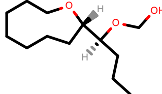
PhEthOH_1341.pdb
