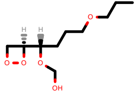
PhEthOH_2677.pdb
