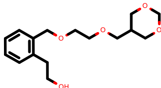
PhEthOH_4805.pdb
