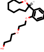
PhEthOH_628.pdb
