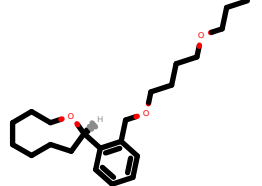
PhEthOH_2687.pdb
