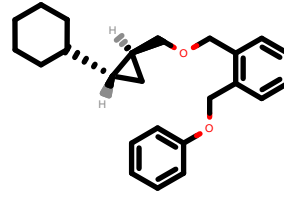
PhEthOH_4498.pdb
