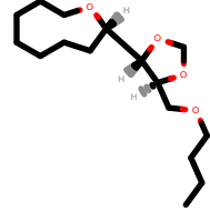
PhEthOH_213.pdb
