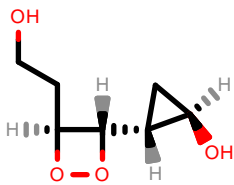
PhEthOH_649.pdb
