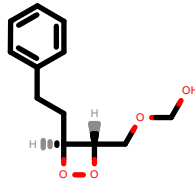
PhEthOH_949.pdb
