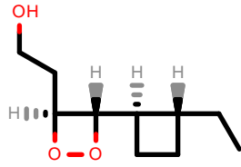
PhEthOH_1573.pdb
