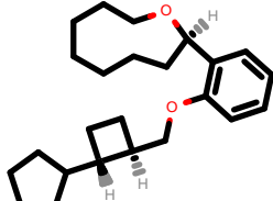
PhEthOH_4156.pdb
