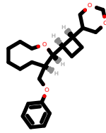
PhEthOH_4965.pdb
