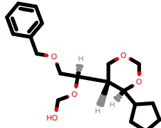
PhEthOH_4212.pdb
