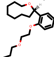
PhEthOH_162.pdb
