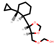
PhEthOH_3340.pdb
