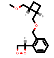
PhEthOH_2003.pdb
