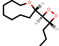
PhEthOH_1342.pdb
