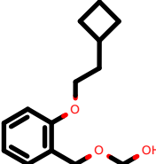
PhEthOH_3420.pdb
