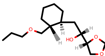
PhEthOH_2934.pdb
