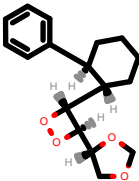
PhEthOH_1252.pdb
