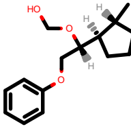
PhEthOH_300.pdb
