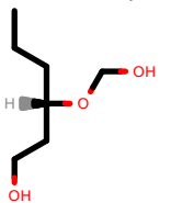
PhEthOH_56.pdb
