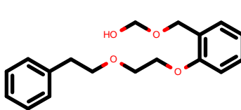
PhEthOH_1026.pdb
