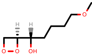
PhEthOH_1832.pdb
