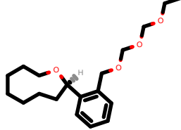
PhEthOH_2225.pdb
