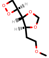
PhEthOH_1754.pdb
