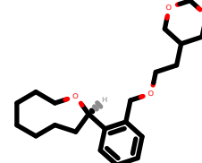
PhEthOH_4703.pdb
