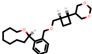
PhEthOH_4993.pdb
