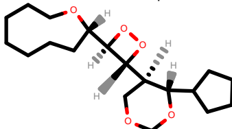
PhEthOH_4244.pdb
