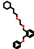
PhEthOH_4456.pdb
