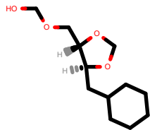
PhEthOH_4268.pdb
