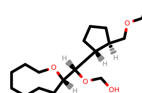
PhEthOH_2475.pdb
