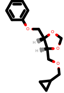
PhEthOH_3116.pdb
