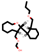
PhEthOH_2925.pdb
