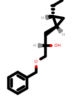
PhEthOH_1523.pdb
