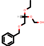
PhEthOH_1356.pdb
