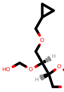
PhEthOH_3145.pdb
