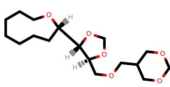
PhEthOH_4829.pdb
