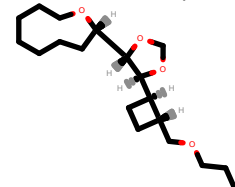
PhEthOH_2859.pdb
