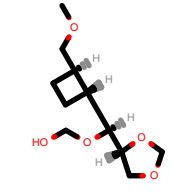
PhEthOH_2011.pdb
