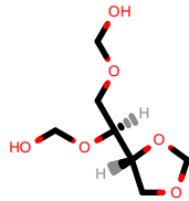
PhEthOH_541.pdb
