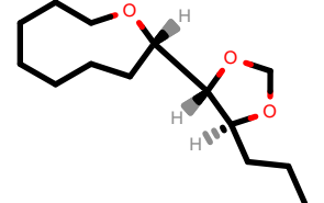
PhEthOH_1343.pdb
