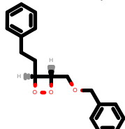
PhEthOH_933.pdb
