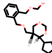
PhEthOH_4223.pdb
