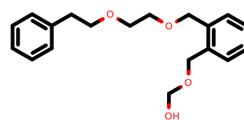
PhEthOH_1027.pdb
