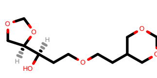
PhEthOH_4862.pdb
