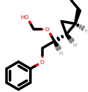
PhEthOH_1518.pdb
