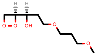
PhEthOH_1874.pdb
