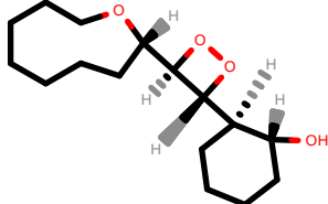
PhEthOH_796.pdb
