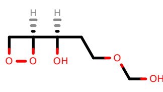
PhEthOH_530.pdb
