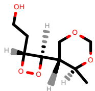
PhEthOH_393.pdb
