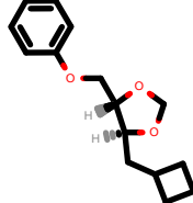
PhEthOH_3410.pdb
