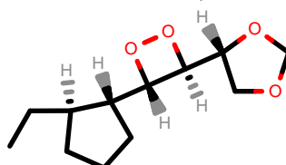
PhEthOH_1630.pdb
