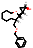
PhEthOH_645.pdb
