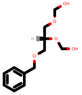
PhEthOH_516.pdb
