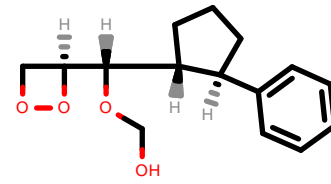
PhEthOH_1207.pdb
