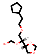
PhEthOH_4027.pdb
