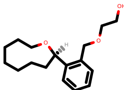
PhEthOH_461.pdb
