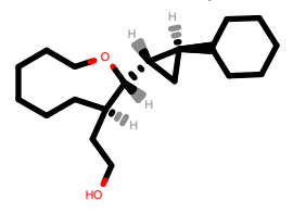
PhEthOH_4511.pdb
