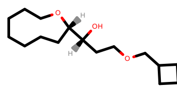
PhEthOH_3570.pdb
