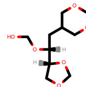
PhEthOH_4695.pdb
