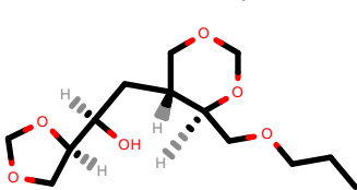
PhEthOH_2972.pdb
