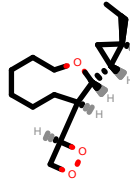
PhEthOH_1545.pdb
