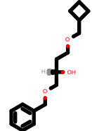
PhEthOH_3539.pdb
