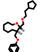
PhEthOH_3999.pdb
