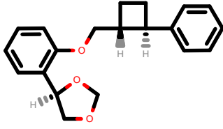
PhEthOH_1168.pdb
