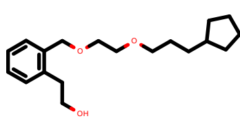
PhEthOH_4049.pdb
