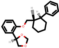
PhEthOH_1252.pdb
