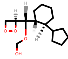
PhEthOH_4189.pdb
