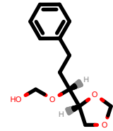
PhEthOH_957.pdb
