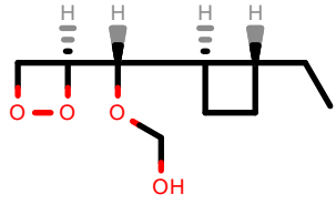
PhEthOH_1585.pdb
