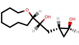
PhEthOH_668.pdb
