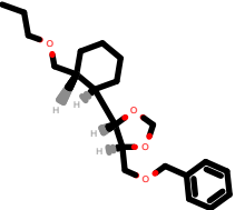
PhEthOH_2908.pdb
