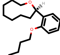
PhEthOH_1342.pdb
