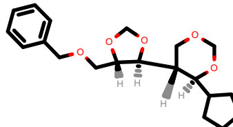
PhEthOH_4214.pdb
