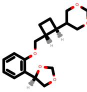
PhEthOH_4990.pdb
