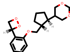
PhEthOH_5022.pdb
