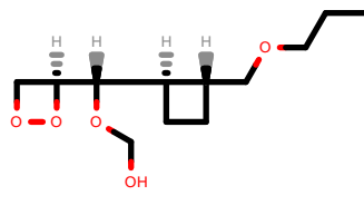
PhEthOH_2845.pdb
