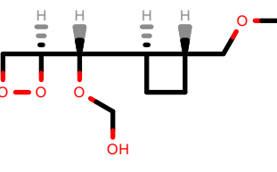
PhEthOH_2005.pdb
