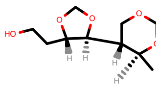
PhEthOH_394.pdb
