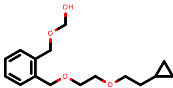
PhEthOH_3169.pdb
