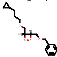
PhEthOH_3205.pdb
