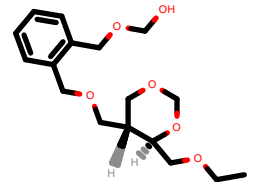
PhEthOH_2539.pdb
