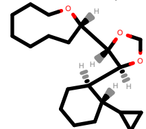
PhEthOH_3359.pdb
