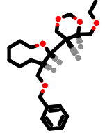
PhEthOH_2535.pdb
