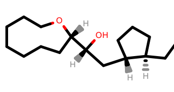
PhEthOH_1634.pdb
