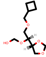
PhEthOH_3565.pdb
