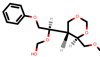
PhEthOH_2102.pdb
