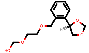
PhEthOH_535.pdb
