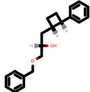
PhEthOH_1145.pdb
