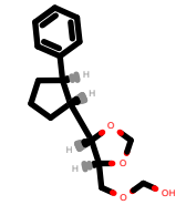
PhEthOH_1202.pdb
