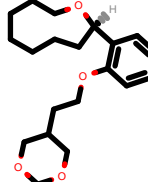
PhEthOH_4702.pdb
