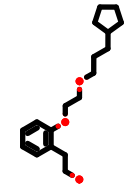
PhEthOH_4048.pdb
