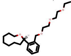
PhEthOH_2309.pdb
