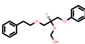
PhEthOH_1010.pdb
