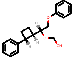
PhEthOH_1140.pdb
