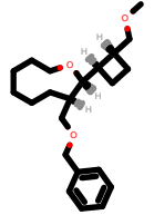
PhEthOH_1989.pdb
