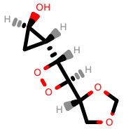
PhEthOH_668.pdb
