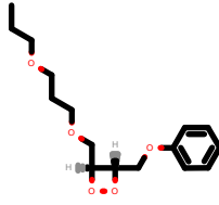
PhEthOH_2737.pdb
