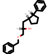
PhEthOH_1183.pdb
