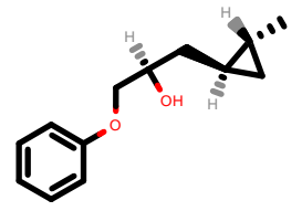
PhEthOH_215.pdb
