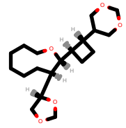
PhEthOH_4991.pdb
