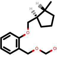
PhEthOH_316.pdb
