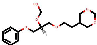
PhEthOH_4832.pdb
