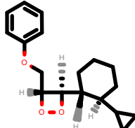
PhEthOH_3325.pdb
