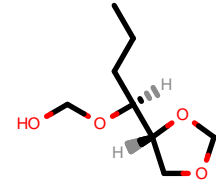
PhEthOH_1339.pdb
