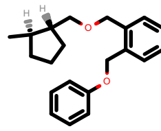
PhEthOH_298.pdb
