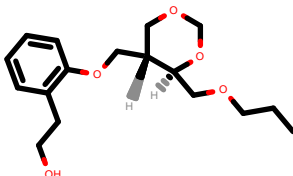
PhEthOH_2956.pdb
