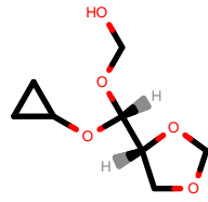
PhEthOH_3061.pdb
