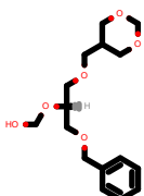
PhEthOH_4796.pdb
