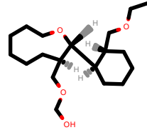
PhEthOH_2505.pdb
