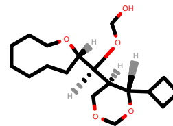
PhEthOH_3823.pdb
