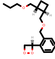
PhEthOH_2843.pdb
