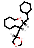
PhEthOH_4281.pdb
