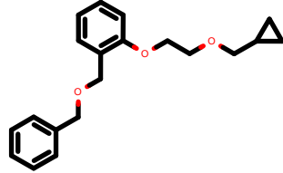
PhEthOH_3118.pdb
