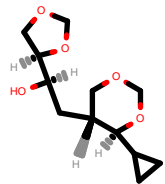
PhEthOH_3396.pdb
