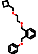
PhEthOH_3532.pdb
