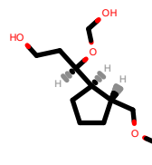
PhEthOH_2450.pdb
