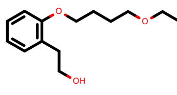
PhEthOH_2238.pdb
