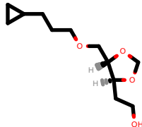
PhEthOH_3208.pdb
