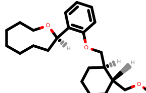
PhEthOH_2098.pdb
