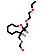
PhEthOH_2295.pdb
