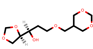
PhEthOH_4820.pdb
