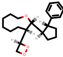
PhEthOH_1205.pdb
