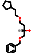
PhEthOH_3997.pdb
