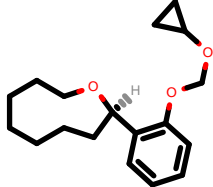
PhEthOH_3064.pdb
