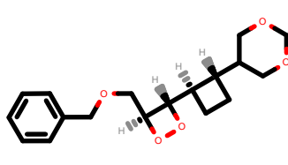
PhEthOH_4969.pdb
