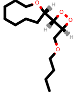
PhEthOH_212.pdb
