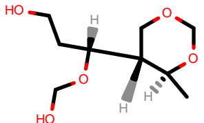
PhEthOH_392.pdb
