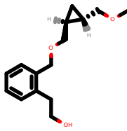
PhEthOH_1949.pdb
