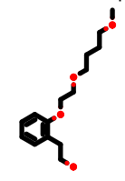
PhEthOH_1906.pdb
