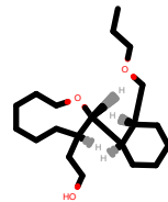
PhEthOH_2919.pdb
