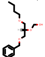
PhEthOH_176.pdb
