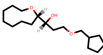
PhEthOH_3986.pdb
