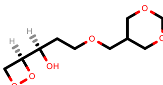
PhEthOH_4814.pdb
