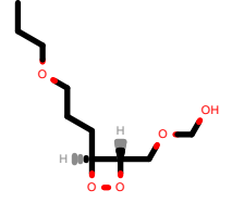
PhEthOH_2671.pdb
