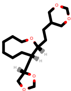
PhEthOH_4781.pdb
