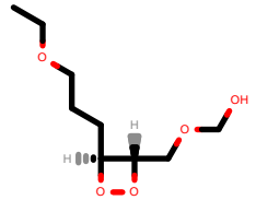
PhEthOH_2247.pdb
