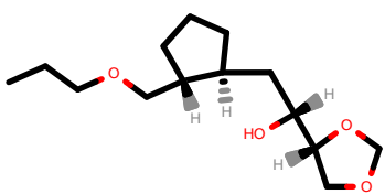
PhEthOH_2888.pdb
