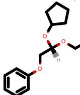
PhEthOH_3870.pdb
