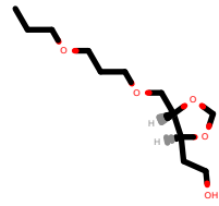
PhEthOH_2750.pdb
