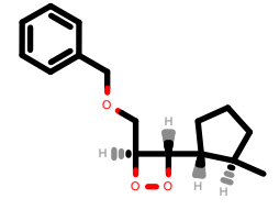
PhEthOH_307.pdb
