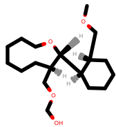
PhEthOH_2081.pdb
