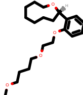
PhEthOH_1930.pdb
