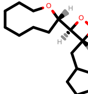
PhEthOH_3866.pdb
