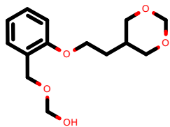
PhEthOH_4684.pdb
