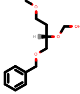
PhEthOH_1734.pdb
