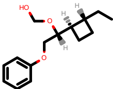
PhEthOH_1556.pdb
