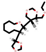
PhEthOH_2555.pdb
