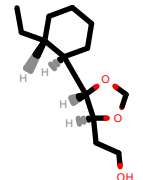
PhEthOH_1654.pdb
