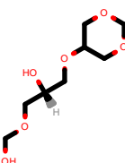
PhEthOH_4724.pdb
