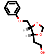
PhEthOH_470.pdb
