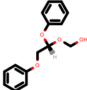
PhEthOH_888.pdb
