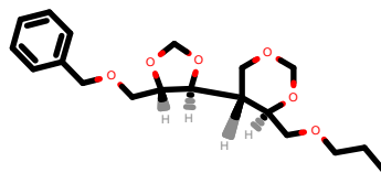
PhEthOH_2950.pdb
