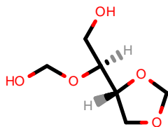
PhEthOH_453.pdb
