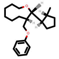
PhEthOH_303.pdb
