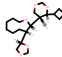
PhEthOH_3819.pdb
