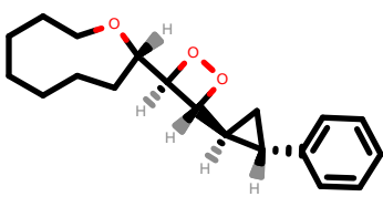
PhEthOH_1136.pdb
