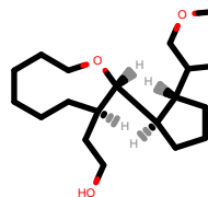
PhEthOH_5015.pdb
