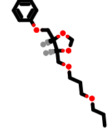
PhEthOH_2738.pdb
