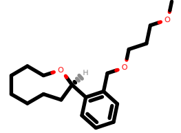
PhEthOH_1759.pdb
