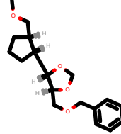
PhEthOH_2030.pdb
