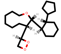
PhEthOH_4191.pdb
