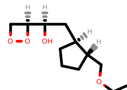
PhEthOH_2462.pdb
