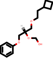
PhEthOH_3576.pdb
