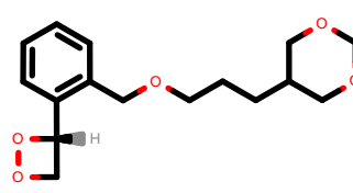
PhEthOH_4771.pdb
