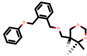
PhEthOH_382.pdb
