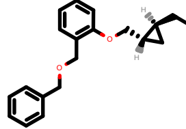
PhEthOH_1522.pdb
