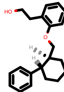
PhEthOH_1234.pdb
