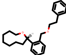
PhEthOH_881.pdb
