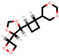
PhEthOH_4988.pdb
