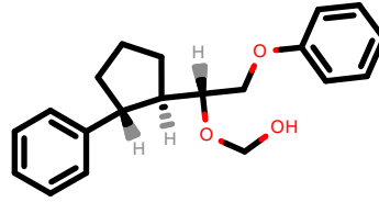
PhEthOH_1182.pdb
