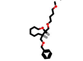
PhEthOH_1905.pdb
