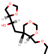
PhEthOH_2552.pdb
