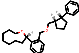
PhEthOH_1213.pdb
