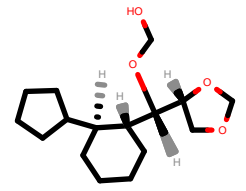
PhEthOH_4191.pdb
