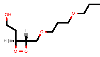
PhEthOH_2749.pdb
