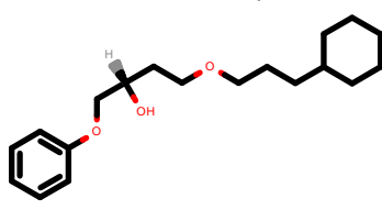
PhEthOH_4457.pdb
