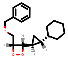
PhEthOH_4507.pdb
