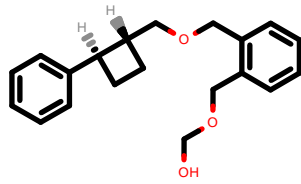
PhEthOH_1157.pdb
