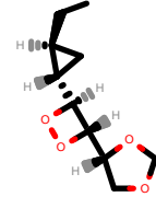
PhEthOH_1546.pdb
