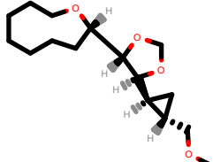
PhEthOH_1977.pdb
