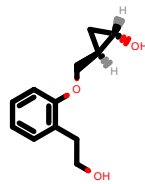
PhEthOH_646.pdb
