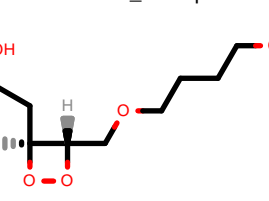
PhEthOH_1909.pdb
