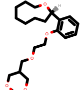
PhEthOH_4828.pdb
