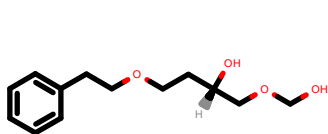
PhEthOH_1028.pdb
