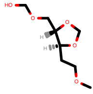
PhEthOH_1748.pdb
