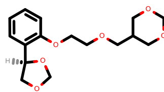
PhEthOH_4818.pdb
