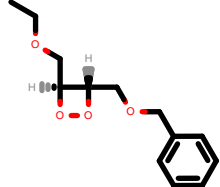
PhEthOH_93.pdb
