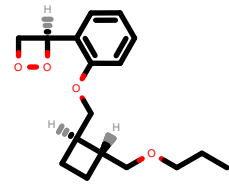
PhEthOH_2842.pdb
