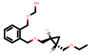
PhEthOH_2375.pdb
