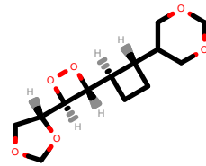
PhEthOH_4990.pdb
