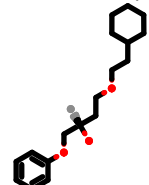
PhEthOH_4411.pdb
