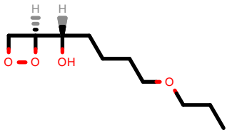
PhEthOH_2676.pdb
