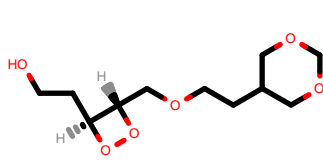
PhEthOH_4845.pdb
