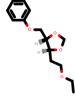
PhEthOH_2150.pdb
