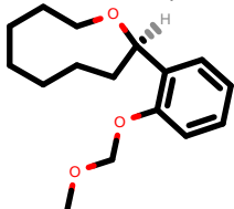
PhEthOH_40.pdb
