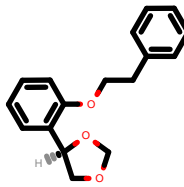
PhEthOH_874.pdb
