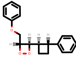
PhEthOH_1141.pdb
