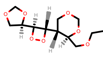
PhEthOH_2554.pdb
