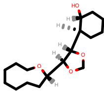
PhEthOH_797.pdb
