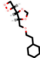
PhEthOH_4442.pdb
