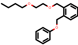
PhEthOH_1432.pdb
