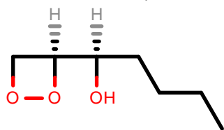
PhEthOH_68.pdb
