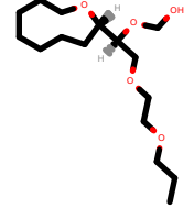
PhEthOH_2731.pdb
