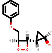
PhEthOH_637.pdb
