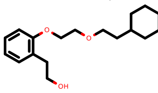
PhEthOH_4426.pdb
