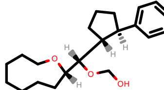
PhEthOH_1215.pdb
