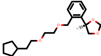
PhEthOH_4025.pdb
