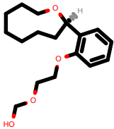
PhEthOH_540.pdb
