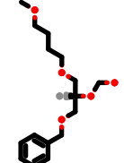
PhEthOH_1898.pdb
