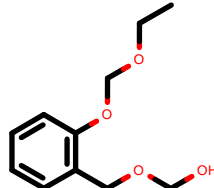
PhEthOH_1366.pdb
