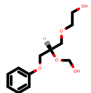
PhEthOH_552.pdb
