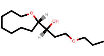
PhEthOH_1428.pdb
