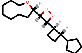
PhEthOH_4156.pdb
