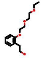
PhEthOH_2284.pdb
