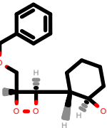
PhEthOH_765.pdb
