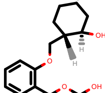
PhEthOH_774.pdb
