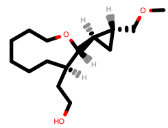
PhEthOH_1949.pdb
