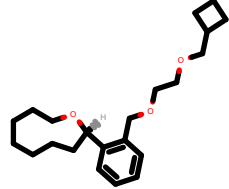
PhEthOH_3569.pdb
