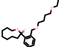
PhEthOH_2267.pdb
