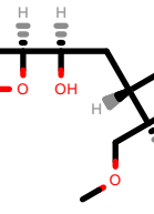
PhEthOH_2004.pdb
