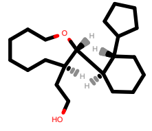
PhEthOH_4179.pdb
