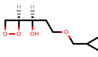
PhEthOH_3134.pdb
