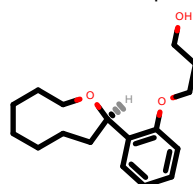
PhEthOH_498.pdb
