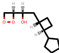
PhEthOH_4146.pdb
