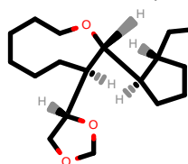
PhEthOH_1631.pdb
