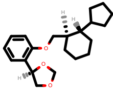
PhEthOH_4188.pdb
