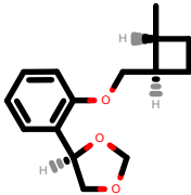
PhEthOH_282.pdb
