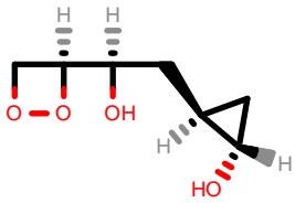
PhEthOH_660.pdb
