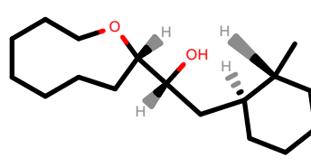
PhEthOH_378.pdb
