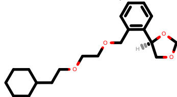
PhEthOH_4445.pdb
