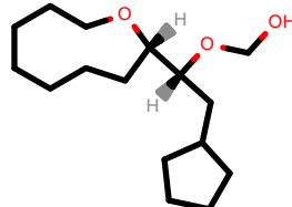
PhEthOH_3865.pdb
