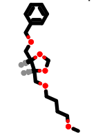
PhEthOH_1904.pdb
