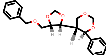
PhEthOH_1270.pdb
