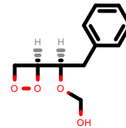
PhEthOH_867.pdb
