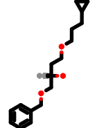
PhEthOH_3199.pdb
