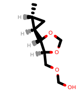
PhEthOH_236.pdb
