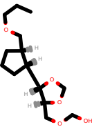
PhEthOH_2878.pdb
