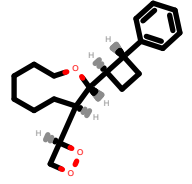
PhEthOH_1167.pdb
