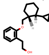
PhEthOH_3334.pdb
