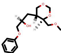
PhEthOH_2101.pdb
