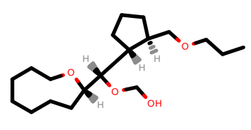
PhEthOH_2899.pdb
