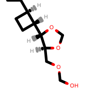
PhEthOH_1580.pdb
