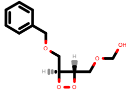
PhEthOH_517.pdb
