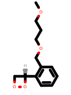
PhEthOH_1751.pdb
