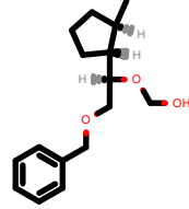
PhEthOH_306.pdb
