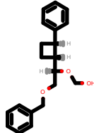
PhEthOH_1146.pdb
