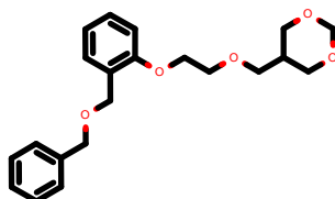
PhEthOH_4794.pdb
