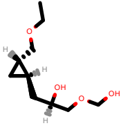
PhEthOH_2376.pdb
