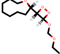
PhEthOH_2228.pdb
