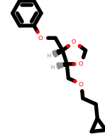
PhEthOH_3158.pdb
