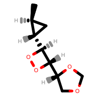
PhEthOH_248.pdb
