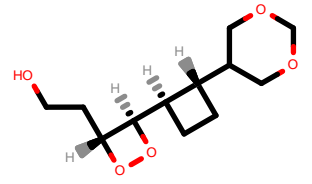
PhEthOH_4975.pdb
