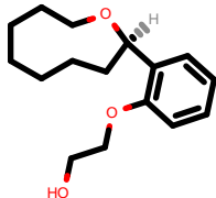
PhEthOH_460.pdb
