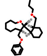
PhEthOH_2907.pdb
