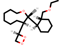
PhEthOH_2511.pdb
