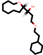
PhEthOH_4452.pdb
