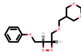
PhEthOH_4791.pdb
