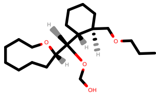
PhEthOH_2941.pdb
