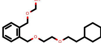
PhEthOH_4433.pdb
