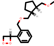
PhEthOH_2045.pdb
