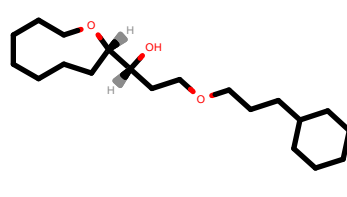
PhEthOH_4494.pdb
