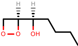
PhEthOH_1332.pdb
