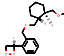
PhEthOH_2083.pdb
