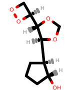
PhEthOH_742.pdb
