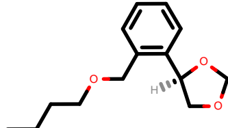
PhEthOH_73.pdb
