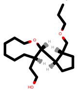
PhEthOH_2877.pdb
