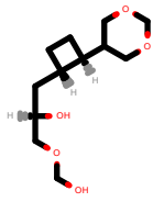
PhEthOH_4980.pdb
