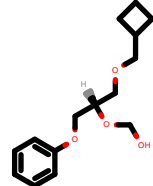
PhEthOH_3534.pdb
