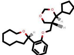
PhEthOH_4240.pdb
