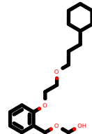
PhEthOH_4474.pdb
