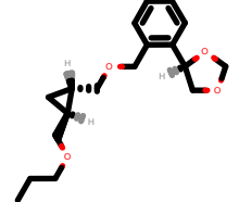
PhEthOH_2807.pdb
