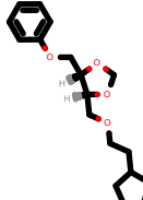
PhEthOH_3998.pdb
