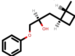
PhEthOH_253.pdb
