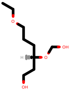
PhEthOH_2244.pdb
