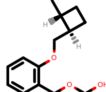
PhEthOH_270.pdb
