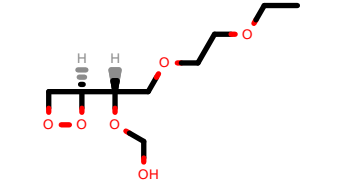
PhEthOH_2299.pdb
