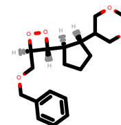
PhEthOH_5011.pdb
