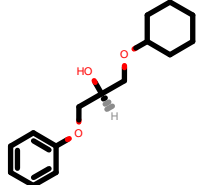
PhEthOH_4285.pdb
