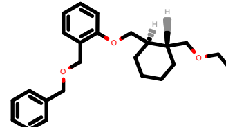
PhEthOH_2484.pdb
