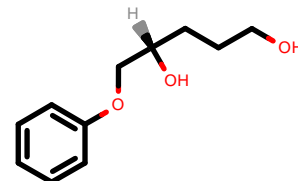
PhEthOH_467.pdb
