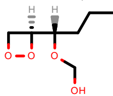
PhEthOH_69.pdb
