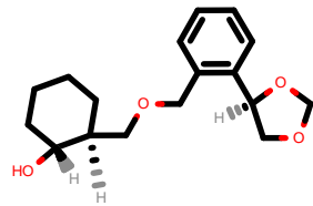
PhEthOH_787.pdb
