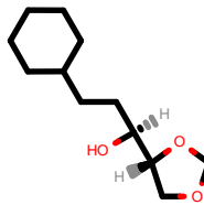
PhEthOH_4278.pdb
