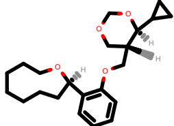
PhEthOH_3400.pdb
