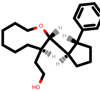
PhEthOH_1193.pdb
