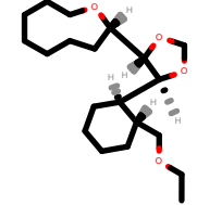
PhEthOH_2523.pdb
