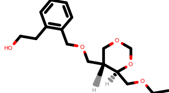
PhEthOH_2533.pdb
