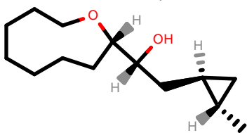
PhEthOH_252.pdb
