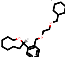
PhEthOH_4405.pdb
