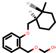
PhEthOH_358.pdb
