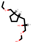
PhEthOH_2460.pdb
