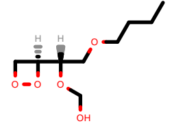
PhEthOH_199.pdb
