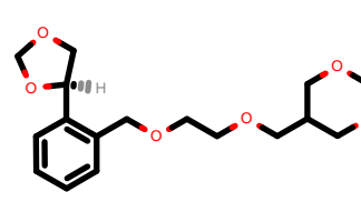
PhEthOH_4819.pdb
