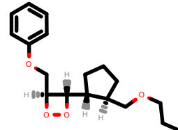
PhEthOH_2863.pdb
