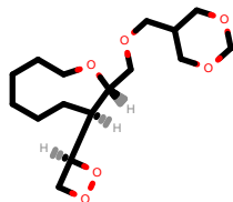
PhEthOH_4817.pdb
