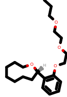
PhEthOH_2728.pdb
