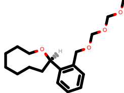
PhEthOH_1805.pdb
