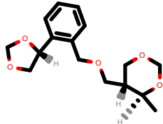
PhEthOH_413.pdb
