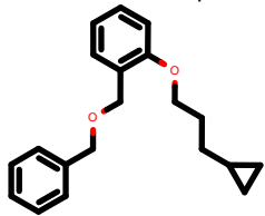
PhEthOH_3076.pdb
