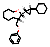
PhEthOH_4503.pdb
