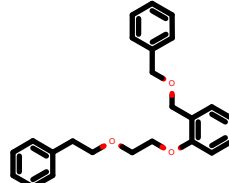
PhEthOH_1018.pdb
