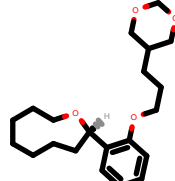
PhEthOH_4782.pdb
