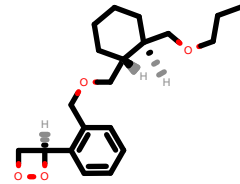
PhEthOH_2927.pdb
