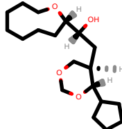
PhEthOH_4242.pdb
