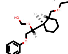
PhEthOH_2480.pdb
