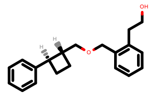
PhEthOH_1151.pdb
