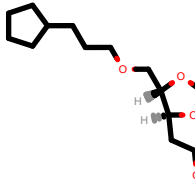
PhEthOH_4052.pdb
