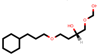
PhEthOH_4476.pdb
