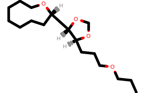
PhEthOH_2687.pdb
