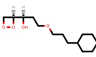
PhEthOH_4478.pdb
