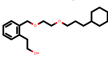
PhEthOH_4469.pdb
