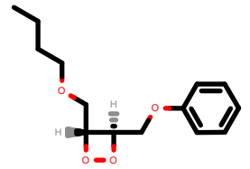
PhEthOH_1435.pdb
