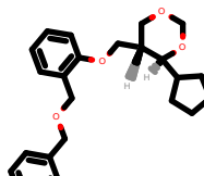
PhEthOH_4206.pdb
