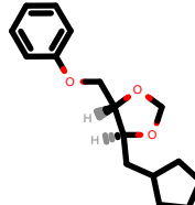
PhEthOH_3830.pdb
