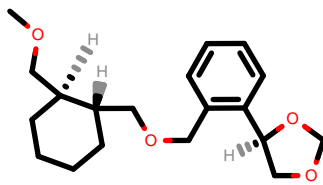
PhEthOH_2089.pdb
