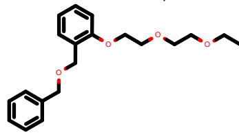
PhEthOH_2278.pdb
