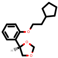
PhEthOH_3856.pdb
