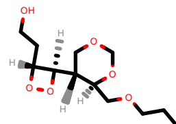
PhEthOH_2955.pdb
