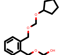
PhEthOH_3887.pdb
