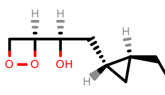
PhEthOH_1542.pdb
