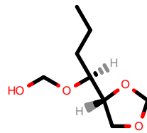
PhEthOH_75.pdb
