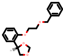
PhEthOH_1000.pdb
