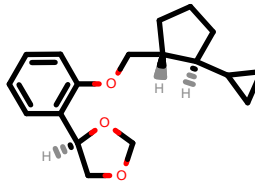
PhEthOH_3310.pdb
