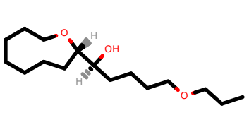
PhEthOH_2684.pdb
