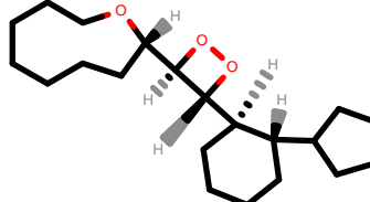
PhEthOH_4202.pdb
