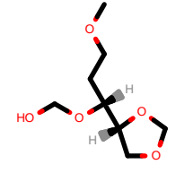
PhEthOH_1759.pdb
