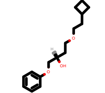
PhEthOH_3575.pdb
