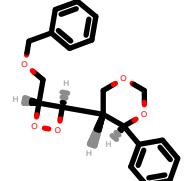
PhEthOH_1269.pdb
