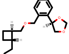
PhEthOH_1589.pdb
