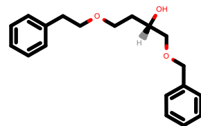
PhEthOH_1019.pdb
