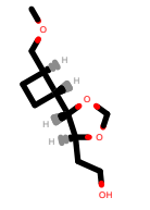
PhEthOH_1994.pdb
