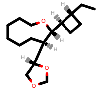
PhEthOH_1593.pdb
