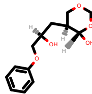
PhEthOH_799.pdb
