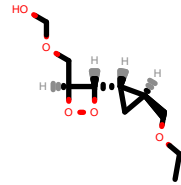
PhEthOH_2377.pdb
