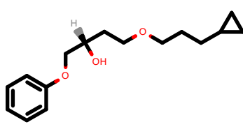
PhEthOH_3197.pdb
