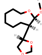
PhEthOH_35.pdb
