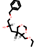
PhEthOH_2527.pdb
