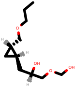
PhEthOH_2792.pdb
