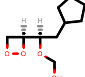
PhEthOH_3853.pdb
