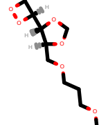
PhEthOH_1876.pdb
