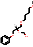
PhEthOH_1896.pdb
