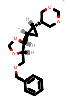
PhEthOH_4924.pdb
