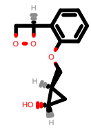
PhEthOH_658.pdb
