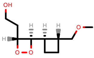
PhEthOH_1993.pdb
