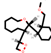
PhEthOH_2087.pdb
