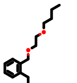
PhEthOH_181.pdb
