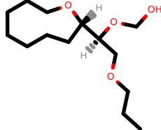
PhEthOH_1429.pdb
