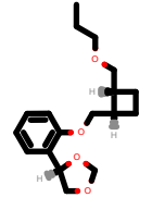
PhEthOH_2844.pdb
