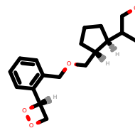
PhEthOH_5023.pdb
