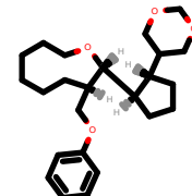
PhEthOH_5007.pdb
