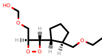
PhEthOH_2461.pdb
