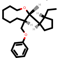
PhEthOH_1605.pdb
