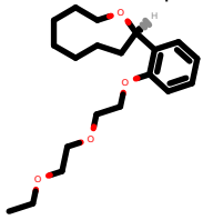
PhEthOH_2308.pdb
