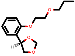
PhEthOH_1420.pdb
