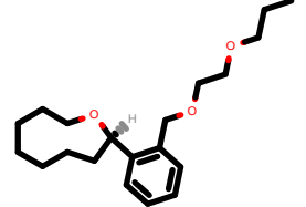
PhEthOH_1427.pdb
