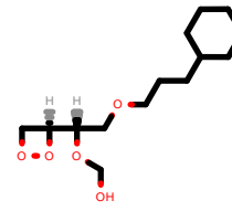
PhEthOH_4479.pdb
