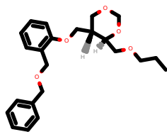
PhEthOH_2950.pdb
