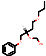
PhEthOH_2568.pdb
