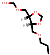
PhEthOH_1412.pdb
