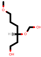
PhEthOH_1820.pdb
