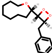
PhEthOH_884.pdb
