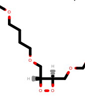
PhEthOH_1915.pdb
