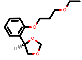
PhEthOH_2172.pdb
