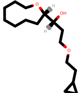
PhEthOH_3192.pdb
