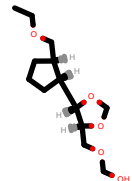
PhEthOH_2462.pdb
