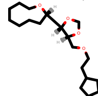
PhEthOH_4031.pdb
