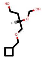
PhEthOH_3546.pdb
