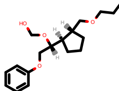
PhEthOH_2862.pdb
