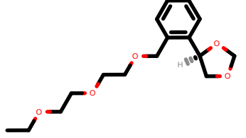
PhEthOH_2303.pdb
