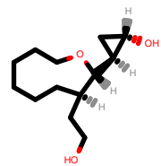
PhEthOH_651.pdb
