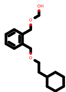
PhEthOH_4265.pdb
