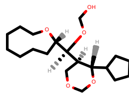
PhEthOH_4243.pdb
