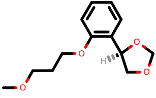
PhEthOH_1756.pdb
