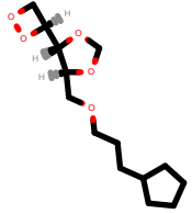
PhEthOH_4060.pdb
