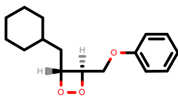
PhEthOH_4249.pdb
