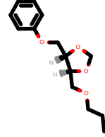
PhEthOH_134.pdb
