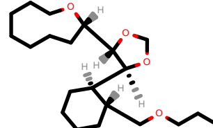
PhEthOH_2943.pdb
