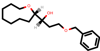
PhEthOH_1004.pdb
