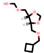
PhEthOH_3550.pdb
