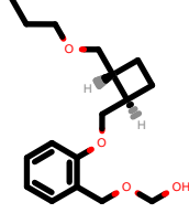
PhEthOH_2836.pdb
