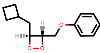
PhEthOH_3409.pdb
