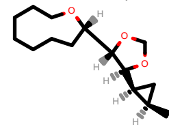
PhEthOH_255.pdb
