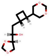
PhEthOH_4988.pdb
