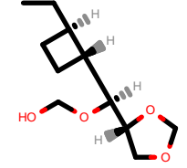
PhEthOH_1591.pdb
