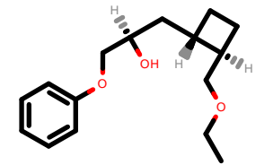
PhEthOH_2399.pdb
