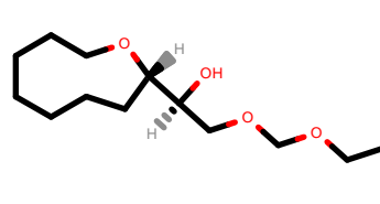
PhEthOH_2226.pdb
