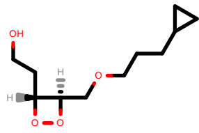
PhEthOH_3211.pdb
