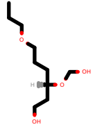
PhEthOH_2660.pdb
