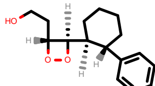
PhEthOH_1233.pdb
