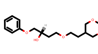
PhEthOH_4831.pdb
