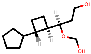
PhEthOH_4134.pdb
