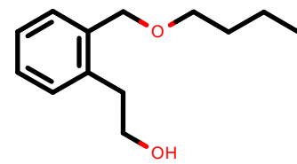
PhEthOH_55.pdb
