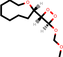
PhEthOH_1808.pdb
