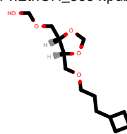
PhEthOH_3638.pdb
