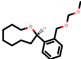
PhEthOH_41.pdb
