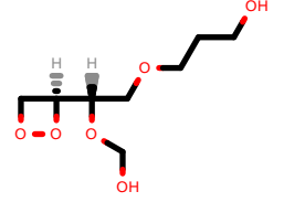
PhEthOH_619.pdb
