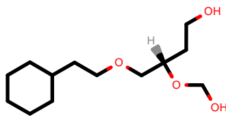
PhEthOH_4428.pdb
