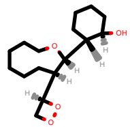
PhEthOH_785.pdb
