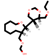
PhEthOH_2543.pdb
