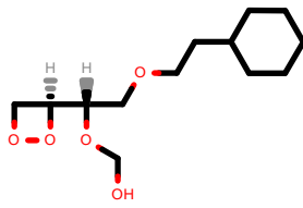
PhEthOH_4441.pdb
