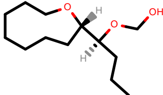
PhEthOH_81.pdb
