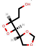
PhEthOH_496.pdb
