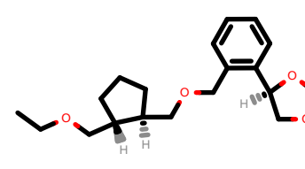
PhEthOH_2471.pdb
