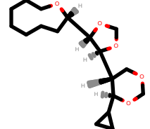
PhEthOH_3405.pdb
