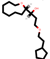
PhEthOH_4028.pdb
