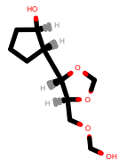
PhEthOH_736.pdb
