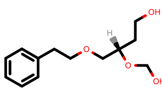
PhEthOH_1022.pdb
