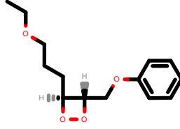
PhEthOH_2233.pdb
