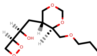
PhEthOH_2966.pdb
