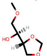
PhEthOH_32.pdb
