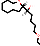
PhEthOH_2268.pdb
