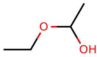
AlkEthOH_c1241
