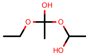
AlkEthOH_c1221
