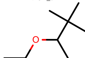
AlkEthOH_c1226
