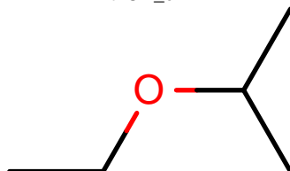
AlkEthOH_c1225
