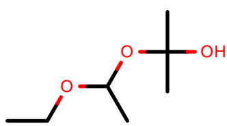
AlkEthOH_c1240
