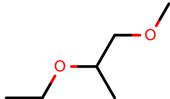
AlkEthOH_c1240
