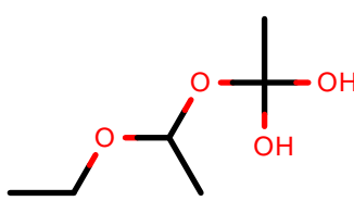
AlkEthOH_c1241
