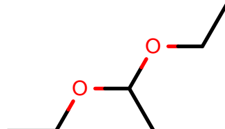
AlkEthOH_c1245
