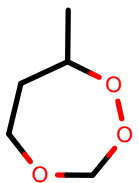
AlkEthOH_r1048
