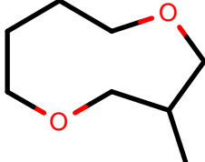
AlkEthOH_r1085
