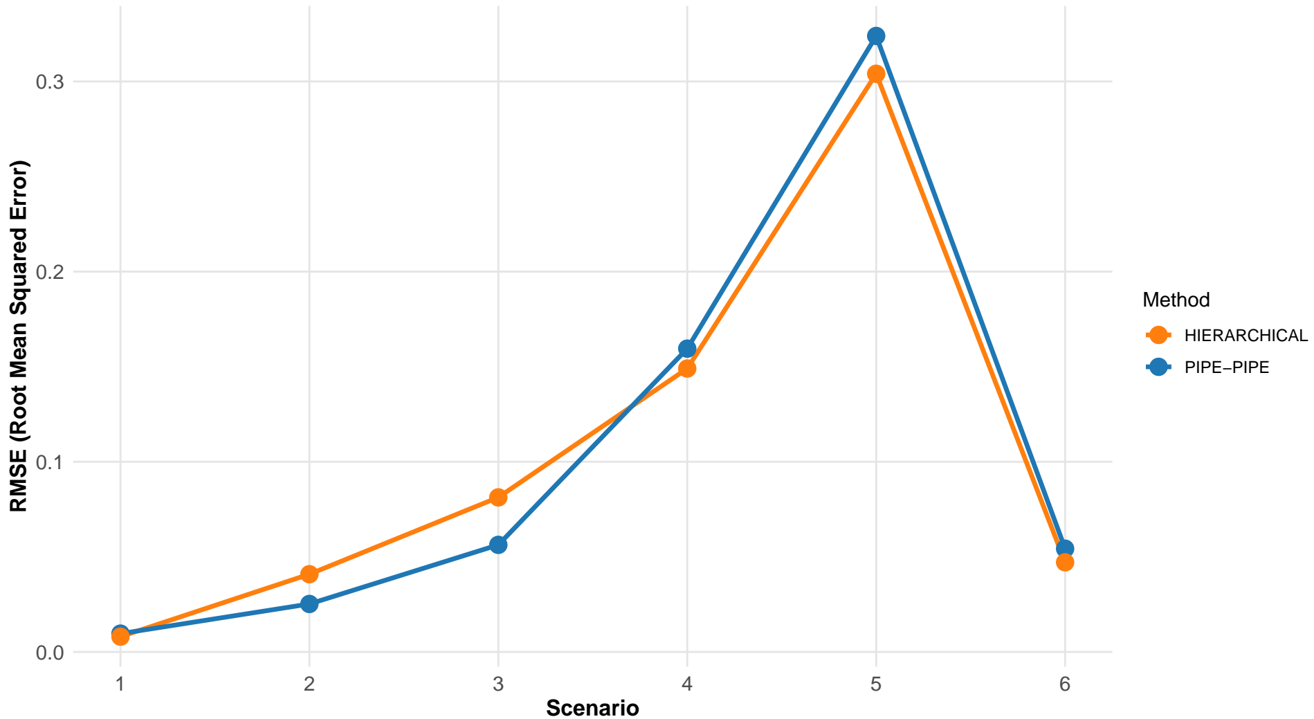
RMSE Comparison Across 6 Scenarios: PIPE-PIPE (Fixed Prior) vs HIERARCHICAL
