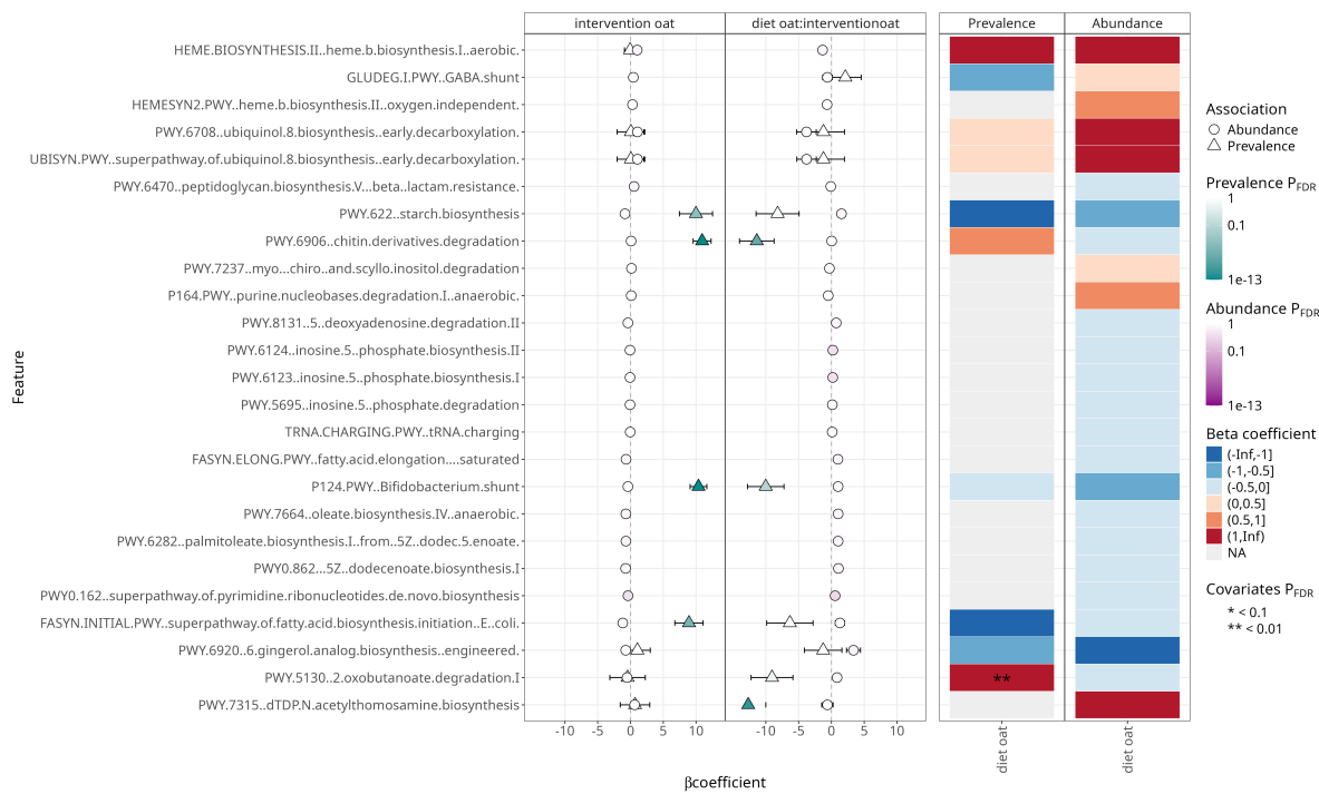
Figure 1: summary_plot.png
