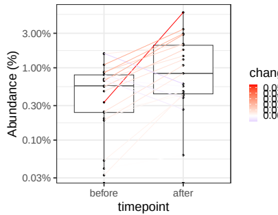
rice / Streptococcus_salivarius
