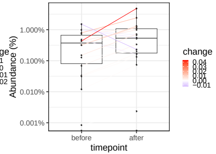
rice / Blautia_SGB4815
