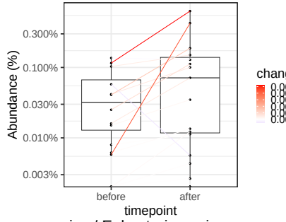
rice / Eubacterium_siraeum
