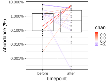
rice / Bifidobacterium_longum
