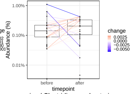
rice / Clostridiaceae_bacterium
