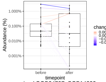
rice / GGB34797_SGB14322
