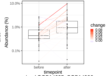
rice / GGB14025_SGB14906
