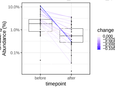
rice / Firmicutes_bacterium_AF16_1
