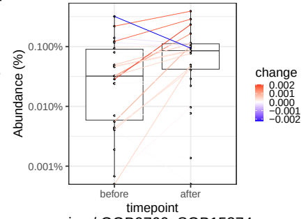
rice / GGB9760_SGB15374
