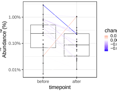
rice / Bilophila_wadsworthia
