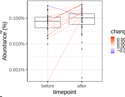
rice / Candidatus_Cibionibacter_quic
