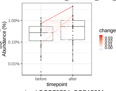
rice / GGB79734_SGB15291
