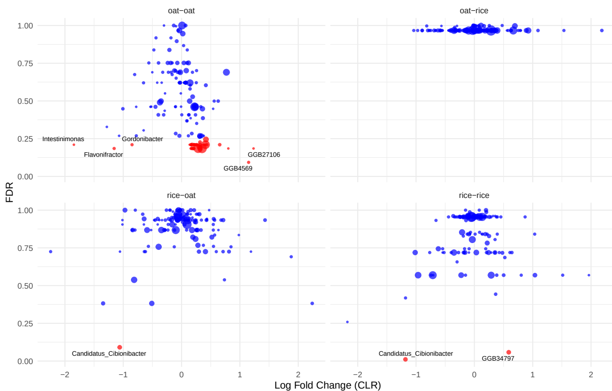
Volcano Plot: Effect Size vs Significance
