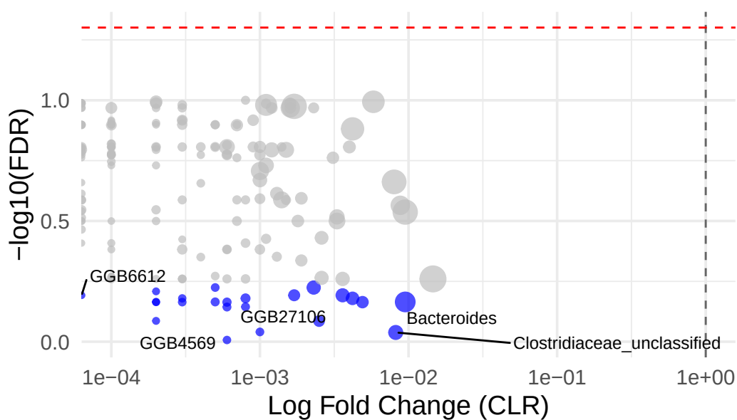
Volcano Plot: Effect Size vs Significance
