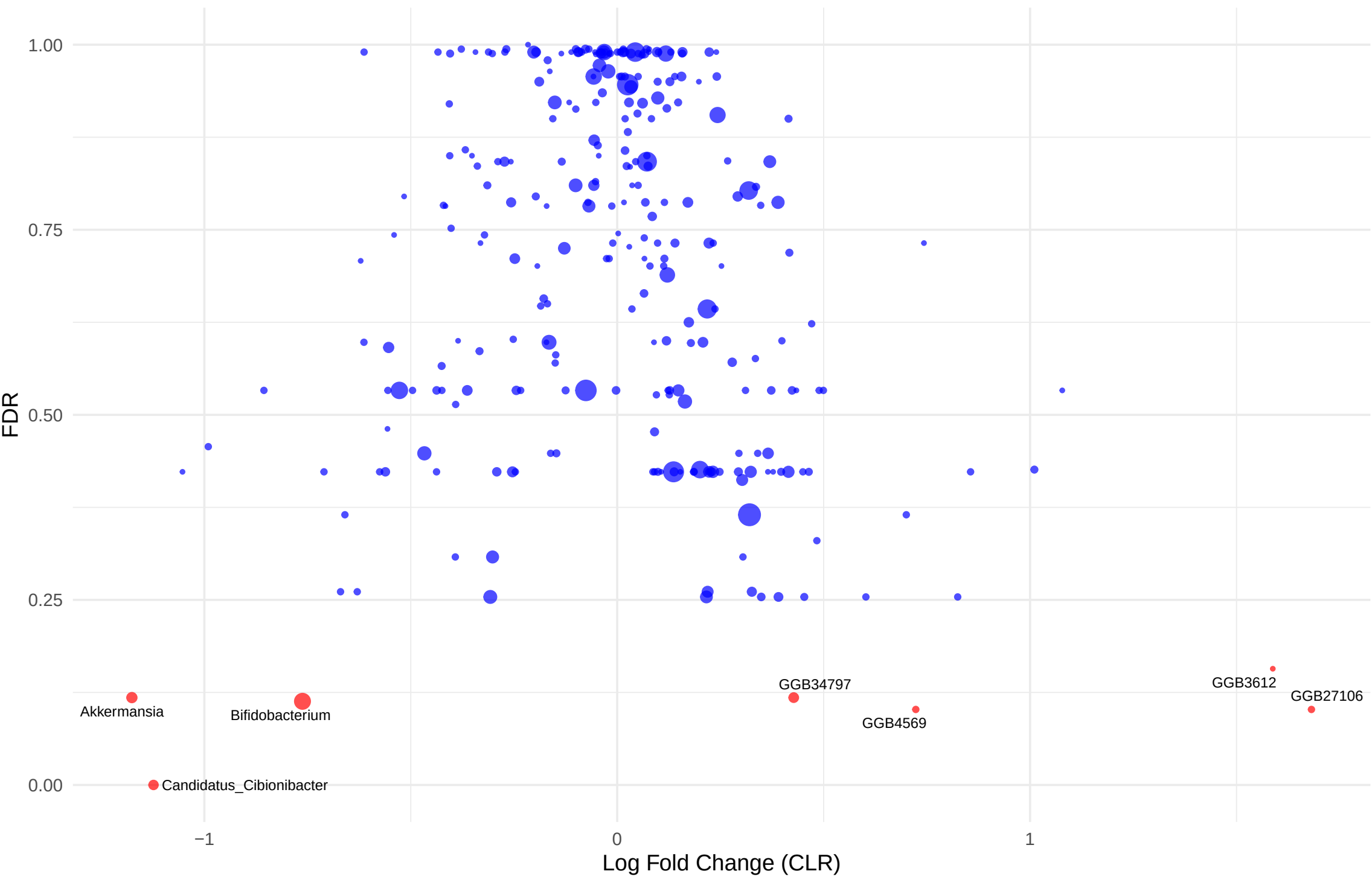
Volcano Plot: Effect Size vs Significance
