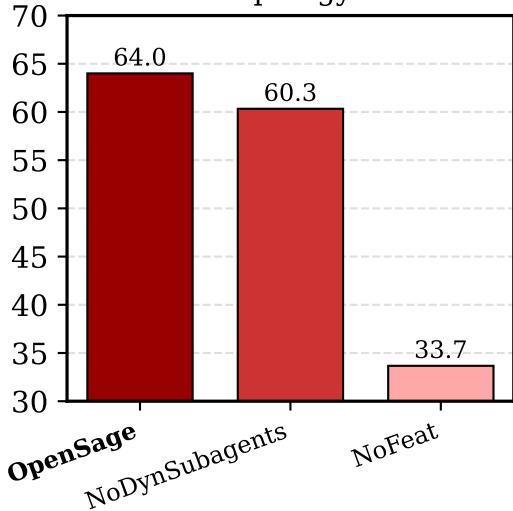
Vertical Topology Ablation
