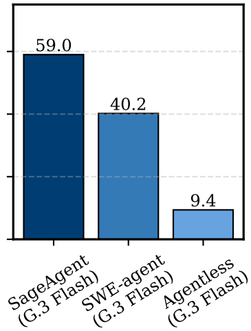
SWE-Bench Pro (Python)
