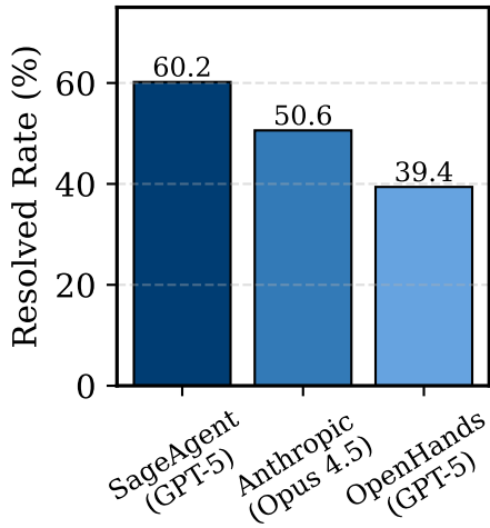
CyberGym
