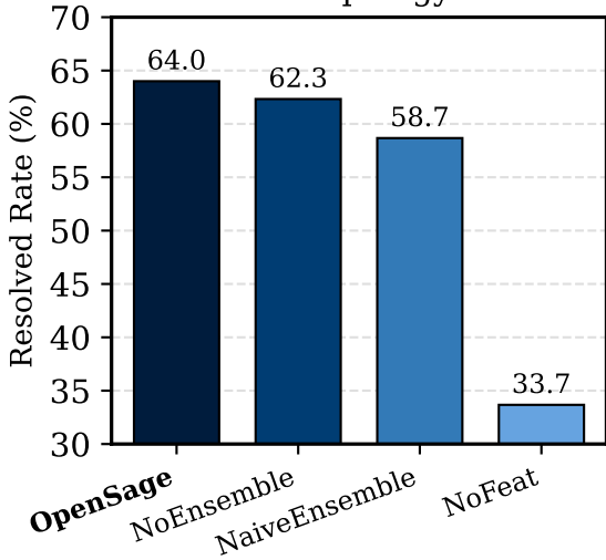
Horizontal Topology Ablation
