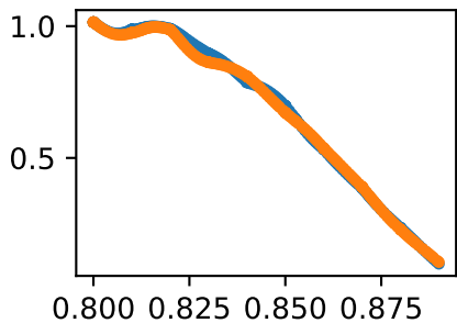
jointsetknee_rknee_angle_rvalue
