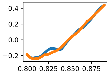
jointsetankle_rankle_angle_rvalue
