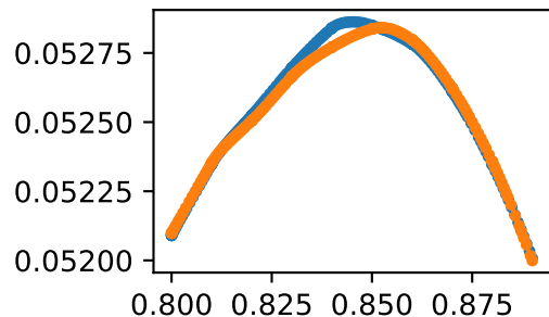
forcesetglut_med3_ractivation
