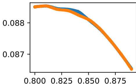
forcesetbifemlh_ractivation
