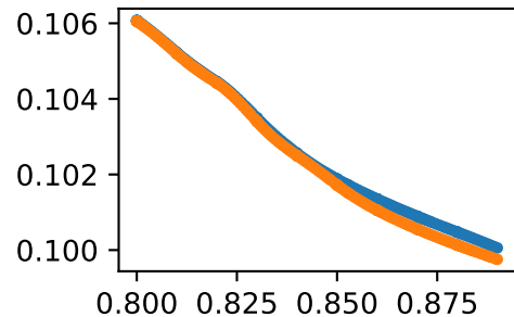
forcesetsar_ractivation
