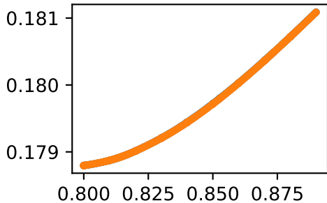
forcesetadd_mag2_ractivation
