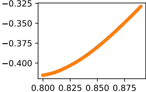
jointsetankle_rankle_angle_rspeed
