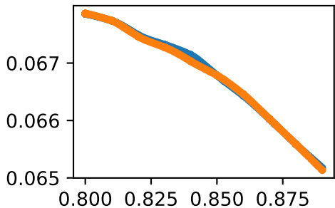
forcesetbifemsh_ractivation
