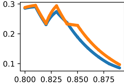
forcesetbifemsh_rfiber_length
