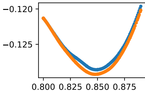
jointsetknee_rknee_angle_rspeed
