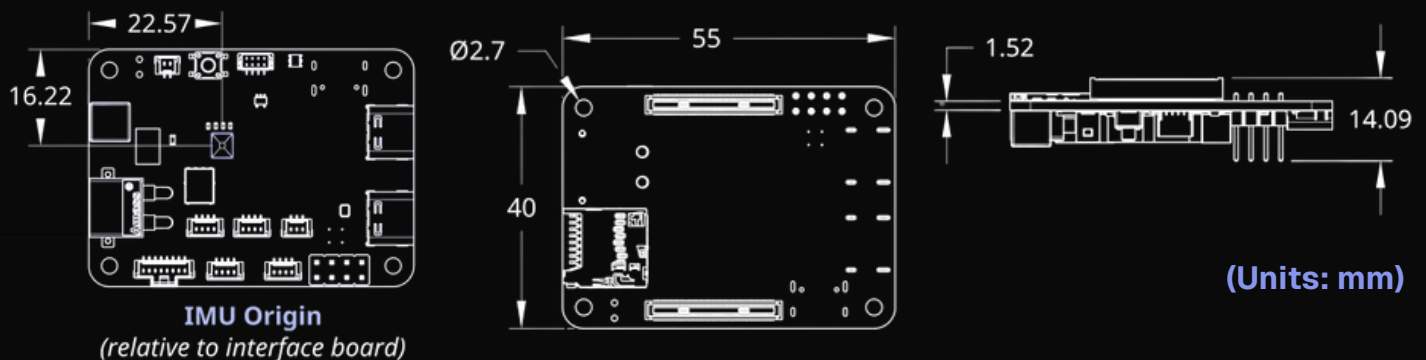
Figure 1: Mechanical Drawing & Sensor Origin
