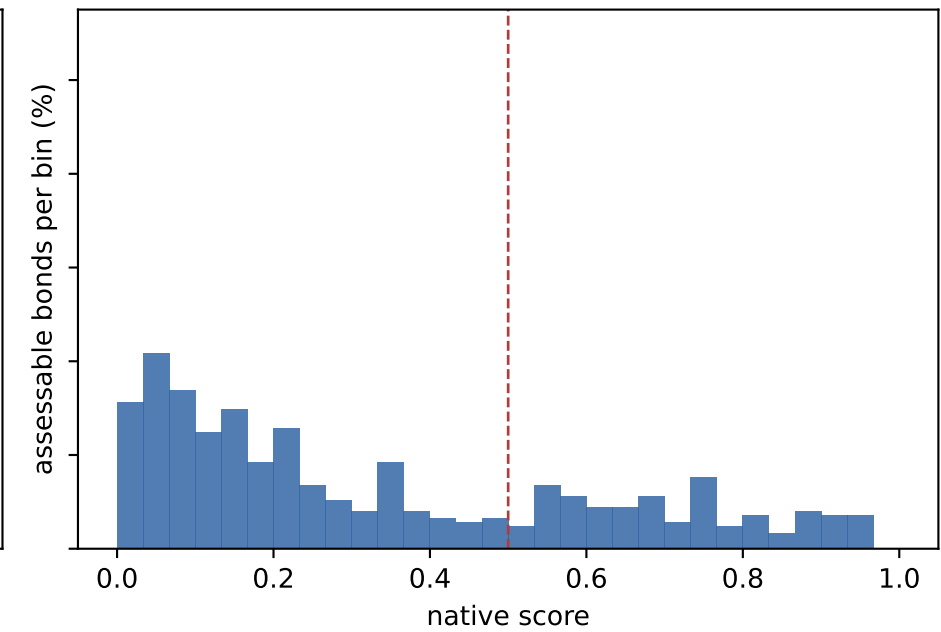
netcleave-ii-hla n=300 assessable bonds
