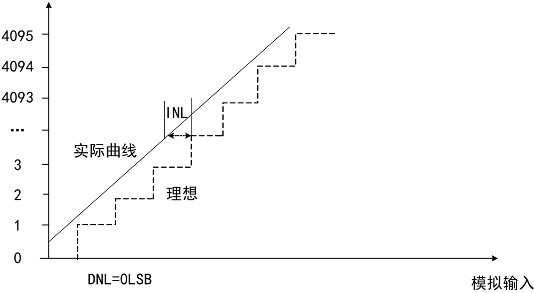
图 1-5 ADC 积分误差
