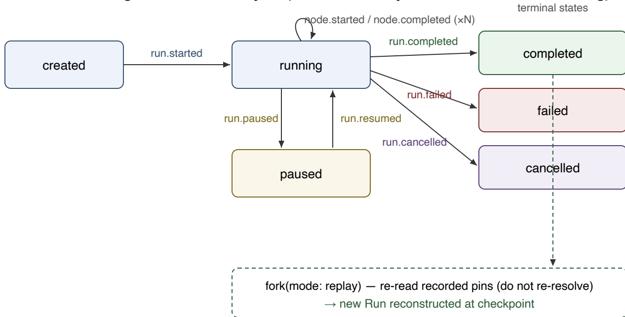
Figure 2 — Run lifecycle (states driven by RunEvents on the EventLog)
