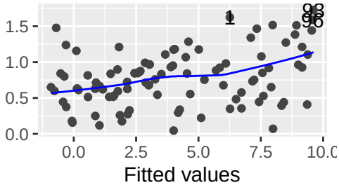
Scale-Location
