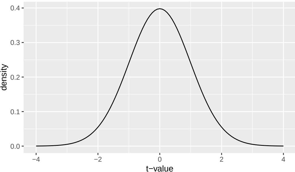
t-distribution with 98 degrees of freedom
