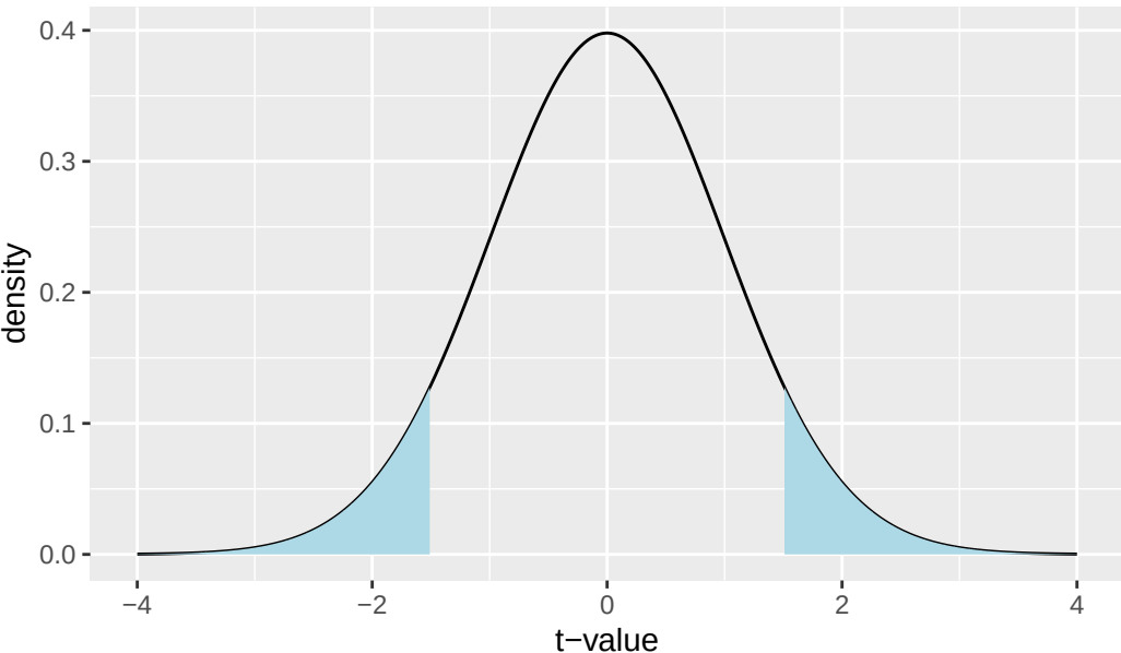
t-distribution with 100 degrees of freedom
