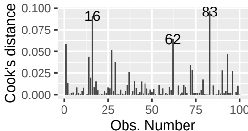
Cook's distance
