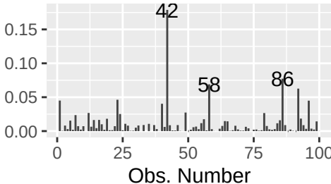
Cook's distance
