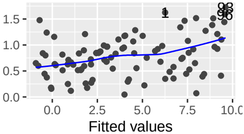
Scale-Location
