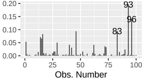
Cook's distance
