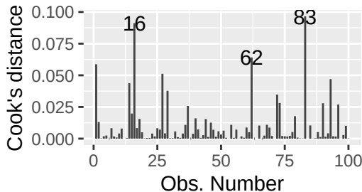
Cook's distance
