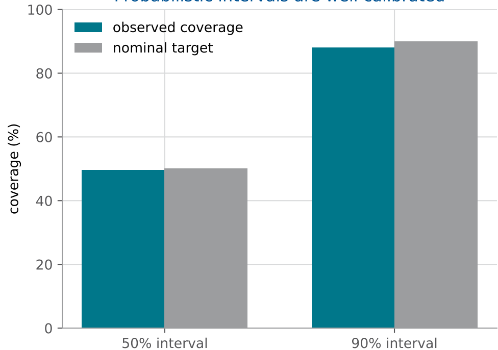
Probabilistic intervals are well calibrated
