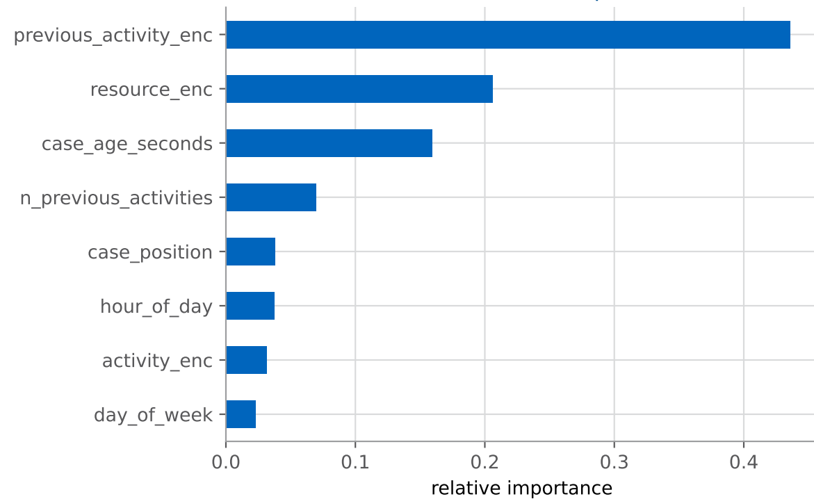
Point-model feature importances
