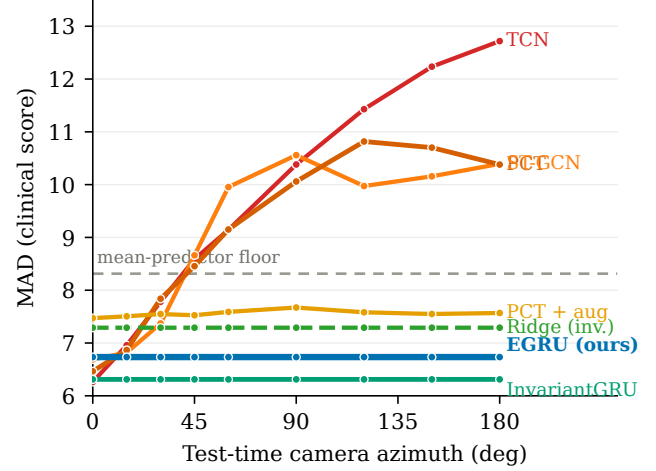
Figure 2. MAD vs. camera azimuth. Certified-invariant models (EGRU, InvariantGRU, hand-crafted Ridge) are flat by theorem; all non-equivariant baselines (PCT, TCN, ST-GCN) degrade 9–13 MAD at extreme angles, indicating viewpoint fragility is a generic property of non-equivariant architectures. Augmentation flattens PCT’s aggregate but not its per-sequence swing (mean 3.01 MAD, worst sequence 20.12). Azimuth here is a rigid rotation of the ground-truth Kinect skeletons; it isolates the geometric effect of viewpoint and does not model per-view tracker degradation.
