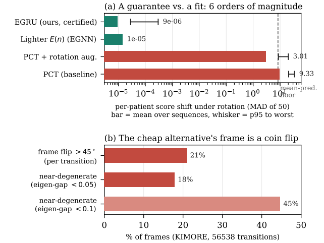
Figure 2. The axis that separates the survivors. (a) Per-patient score shift under camera rotation (log scale); bar is the mean over held-out sequences at the worst azimuth, whisker runs 95th percentile to worst sequence — the tail the mean conceals, and the reason we report both. EGNN has no measured tail and so carries no whisker. The certified models (EGRU, EGNN) hold a patient’s score to \sim 10^{-5} MAD, five to six orders of magnitude below the augmented and unaugmented transformers, whose worst sequences move 20.12 and 33.96 points of fifty. InvariantGRU is exactly 0 and Canon-PCA empirically \approx 0 , but unbounded off distribution. (b) Why the cheap canonicalization alternative is not a guarantee: its PCA frame flips by > 45^\circ on 21% of frame transitions and sits within an eigen-gap of 0.05 of degeneracy on 18% of frames.
