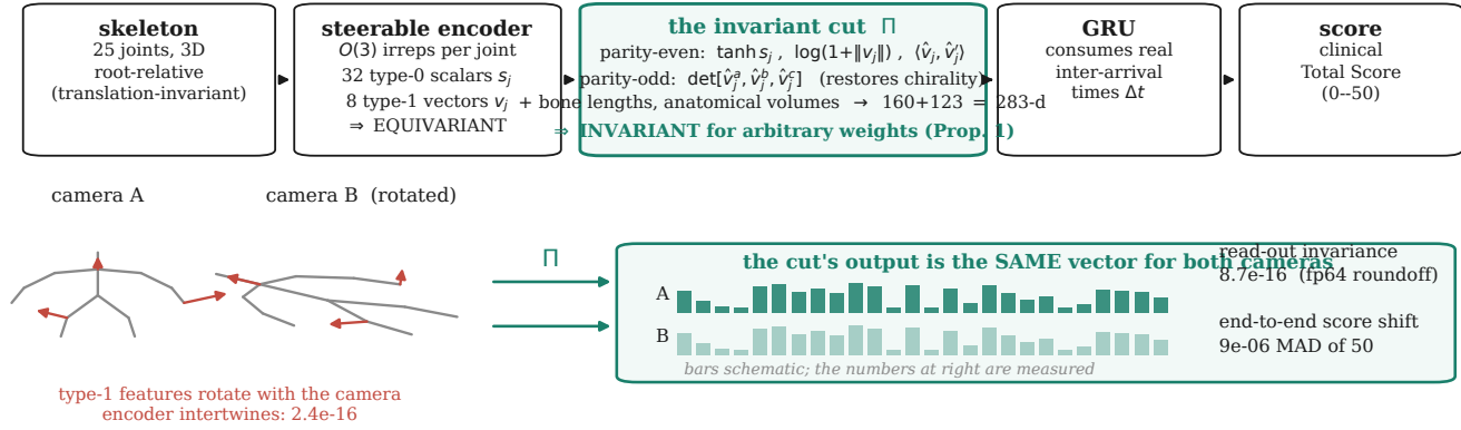
Figure 1. The invariant cut is the method. Top: the pipeline. Bottom: the same pose at two camera poses — the encoder’s type-1 features rotate (equivariance), the cut’s output does not (invariance, Prop. 1). Bar heights are schematic; the annotated quantities are measured (certify_egru.json, final_tables.json).
