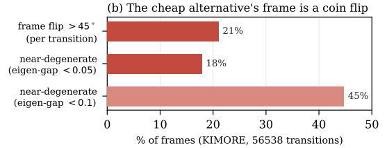
Figure 2. The axis that separates the survivors. (a) Worst-case per-patient score shift under camera rotation (log scale): the certified models (EGRU, EGNN) hold a patient’s score to \sim 10^{-5} MAD, six orders of magnitude below the augmented and unaugmented transformers. InvariantGRU is exactly 0 and Canon-PCA empirically \approx 0 , but unbounded off distribution. (b) Why the cheap canonicalization alternative is not a guarantee: its PCA frame flips by > 45^\circ on 21% of frame transitions and sits within an eigen-gap of 0.05 of degeneracy on 18% of frames.
