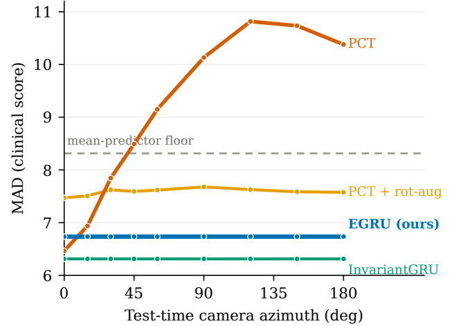
Figure 1. MAD vs. camera azimuth. Certified-invariant models are flat by theorem; the transformer degrades through the mean-predictor floor. Augmentation flattens the mean but not the per-sequence swing (3.03 MAD).
