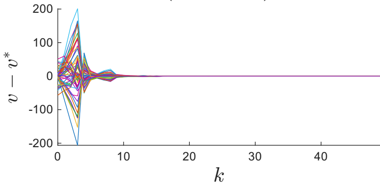
State (Network) Error
