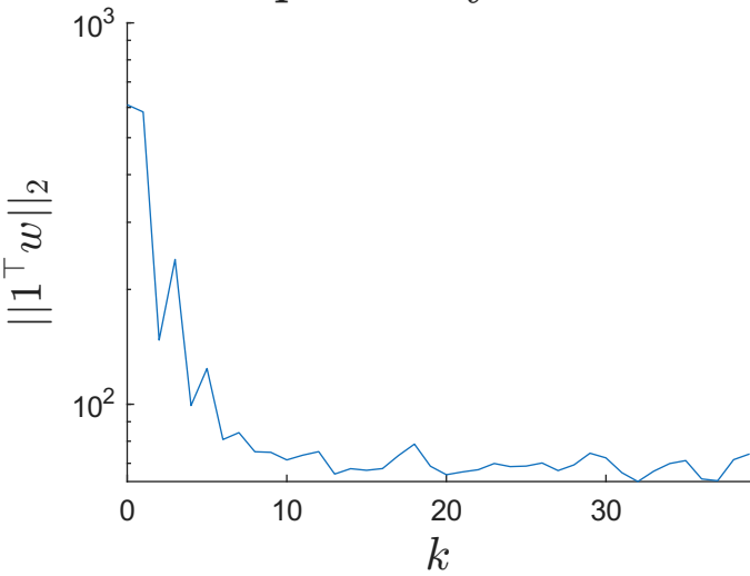
Optimality Error
