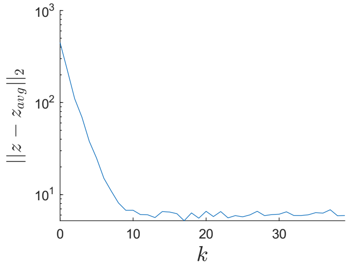
Consensus Error
