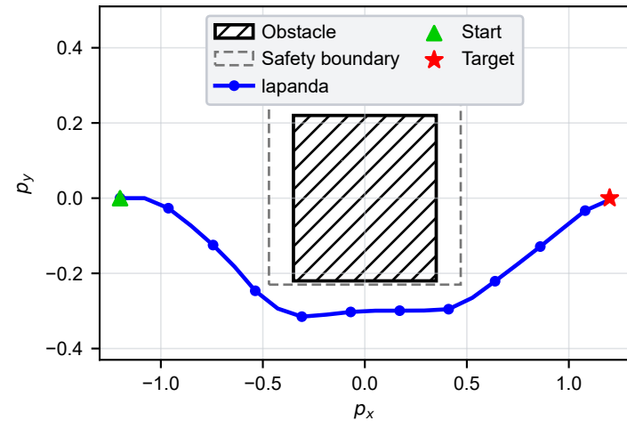
(a) Closed-loop trajectory
