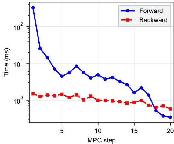
(b) Per-step computation time
