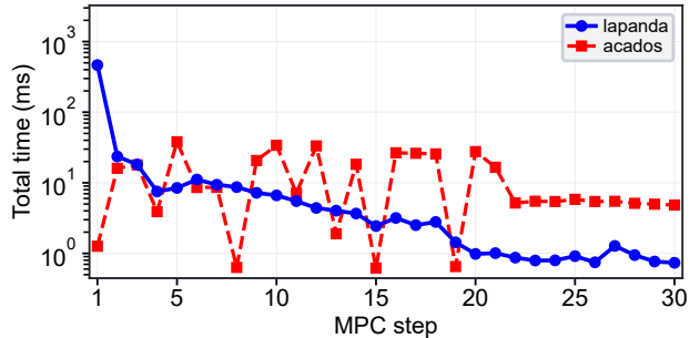
(b) Per-step computation time
