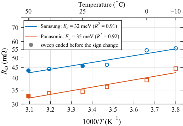
(a) Ohmic intercept R_{\Omega}
