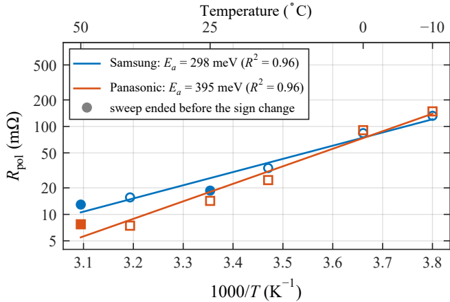
(b) Polarisation resistance R_{pol}
