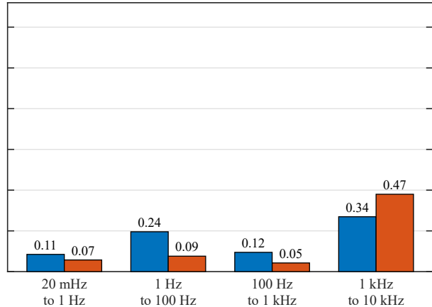
(b) LG INR21700-M50
