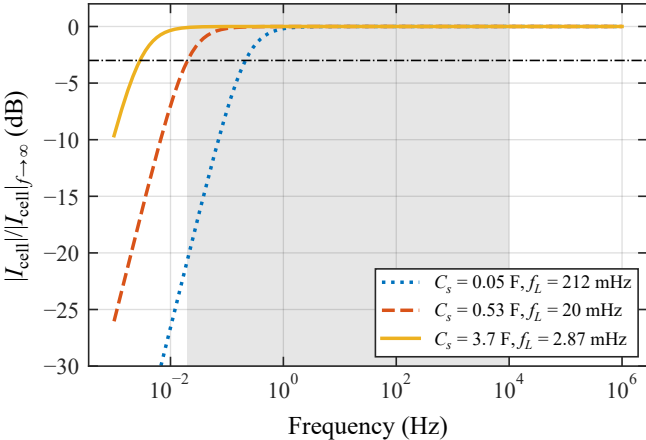
(a) Blocking network, R_{\text{loop}} = 15 \Omega
