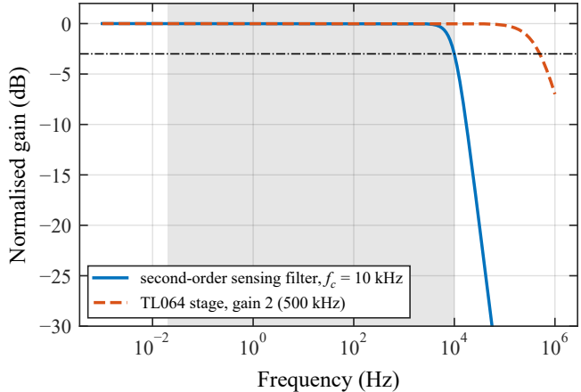
(b) Sensing filter and drive stage
