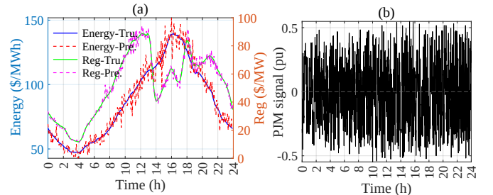
Fig. 1. Actual and forecast values of energy and reserve prices and PJM regulation signal: (a) actual and forecast values of energy and reserve prices. (b) PJM regulation signal.
