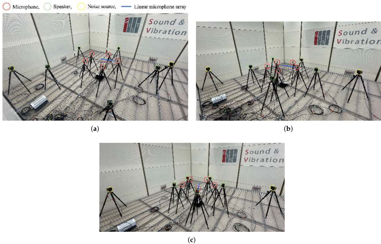
Figure 11. Experimental setup, (a–c) cases 1–3.
