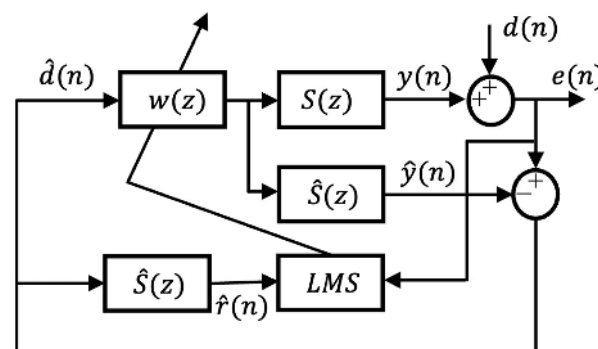
Figure 6. Block diagram of adaptive feedback FxLMS.
