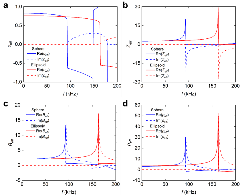
Figure 2.3 a-d, Real (solid line) and imaginary part (dashed line) of the effective speed of sound c_{\text{eff}} , acoustic impedance Z_{\text{eff}} , bulk modulus B_{\text{eff}} , and mass density \rho_{\text{eff}} of the spherical (blue) and ellipsoidal meta-atoms (red) are plotted in the frequency range of 1–200 kHz. All values are calculated using the S-parameter retrieval method (Supplementary Fig. 2a,b).
