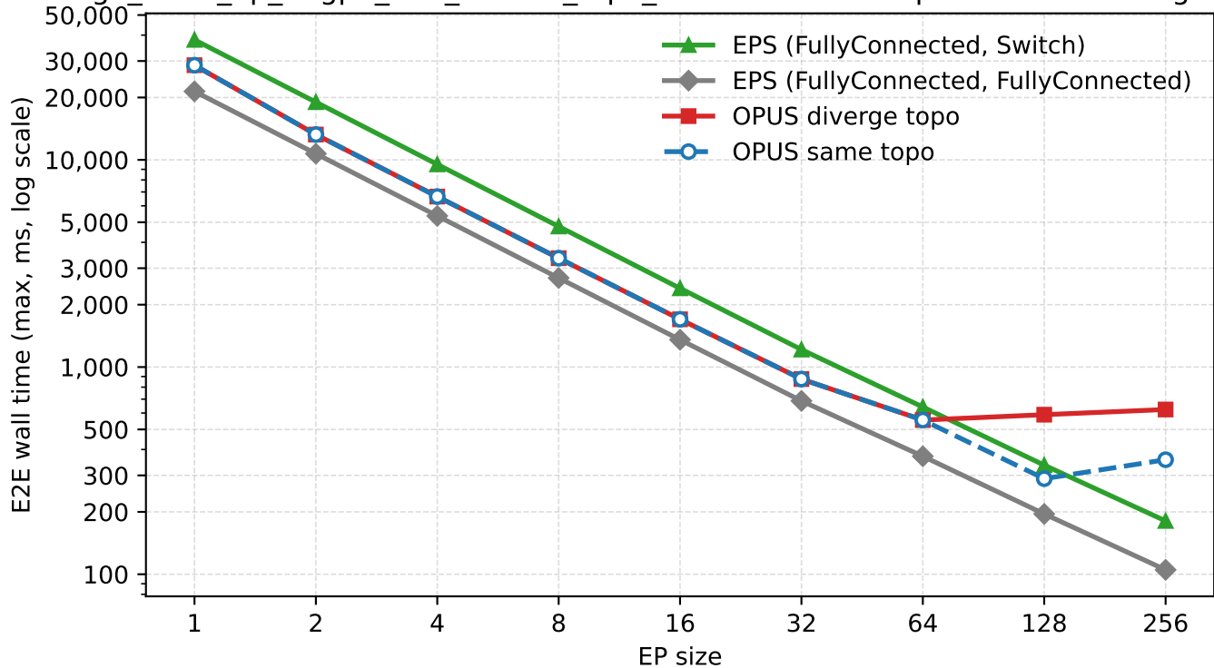
large_scale_ep_32gpu_512_all2allv_topk_context - EP sweep at 1ms switching lat
