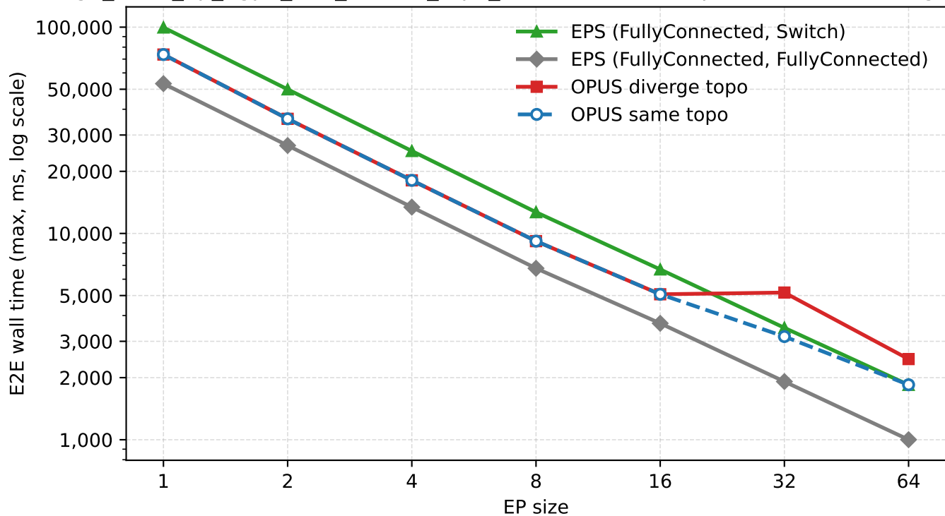
large_scale_ep_8gpu_256_all2allv_topk_context - EP sweep at 500us switching lat
