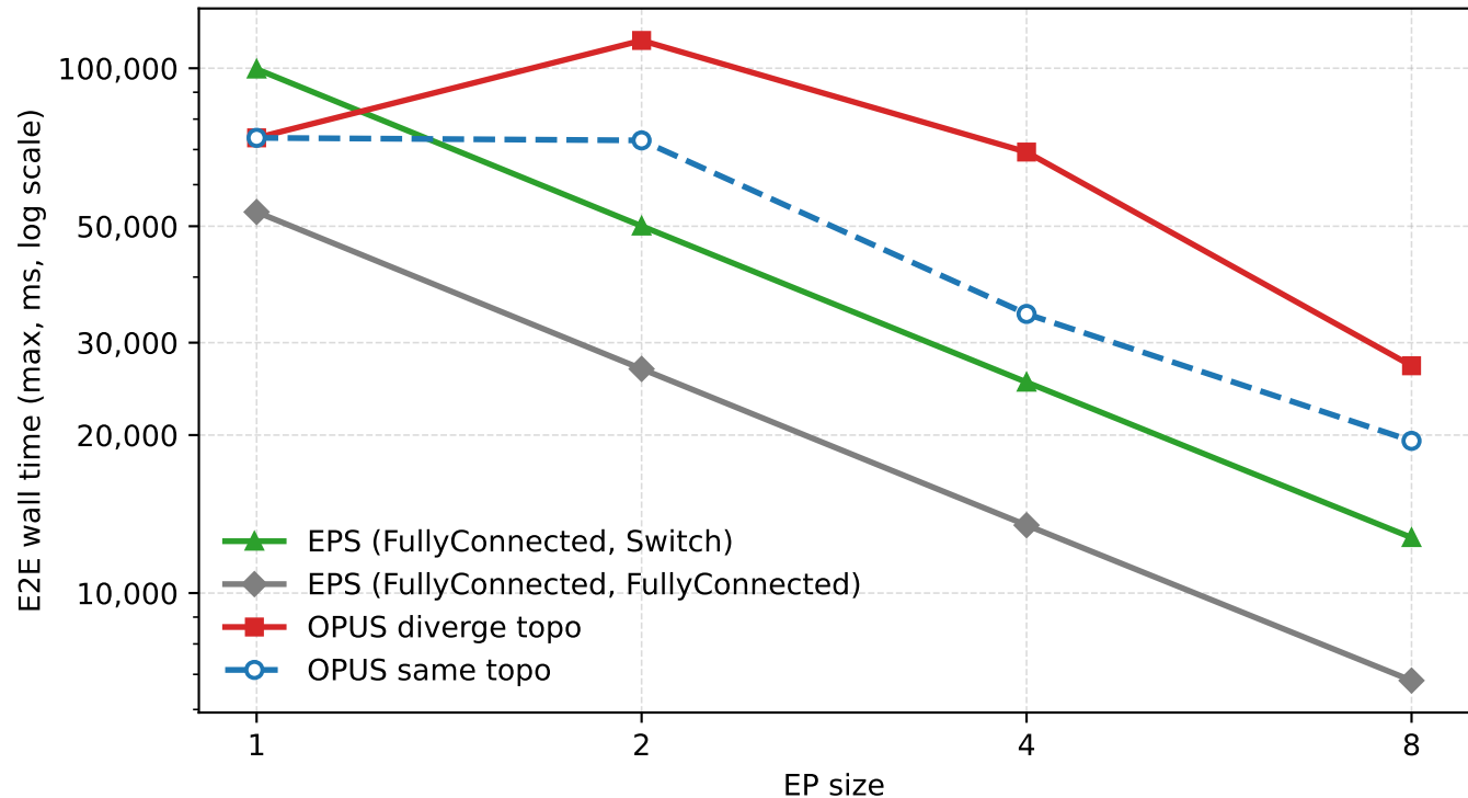
large_scale_ep_scaleout_8gpu_256_all2allv_topk_context - EP sweep at 1ms switchin
