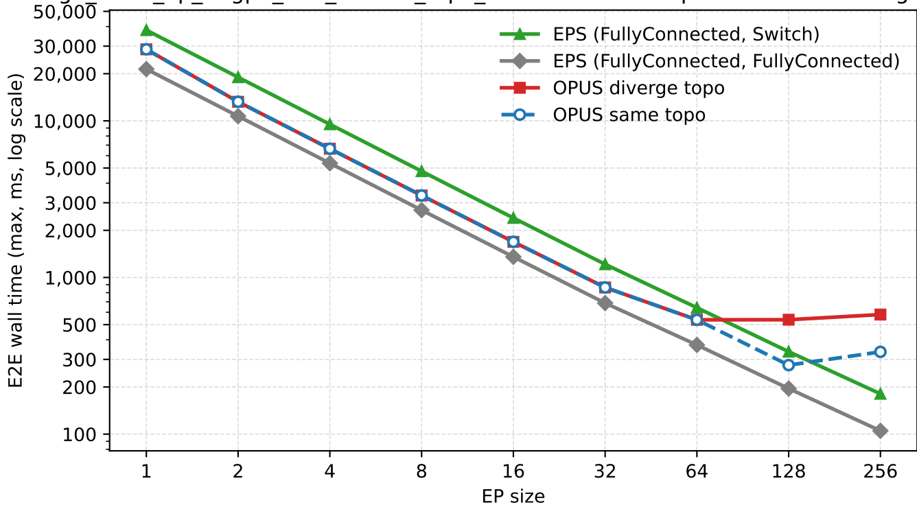
large_scale_ep_32gpu_512_all2allv_topk_context - EP sweep at 500us switching la
