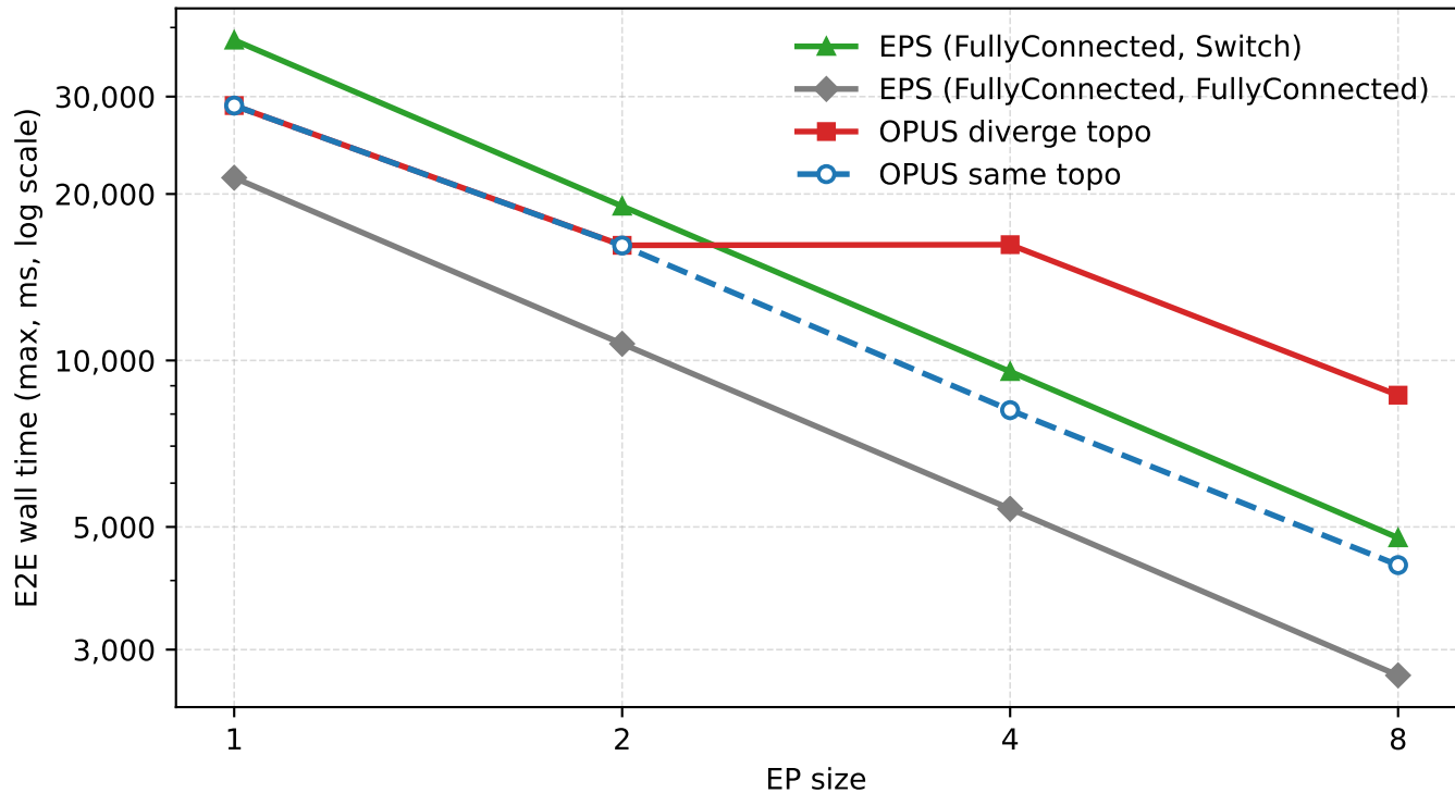
large_scale_ep_scaleout_32gpu_512_all2allv_topk_context - EP sweep at 10ms switching
