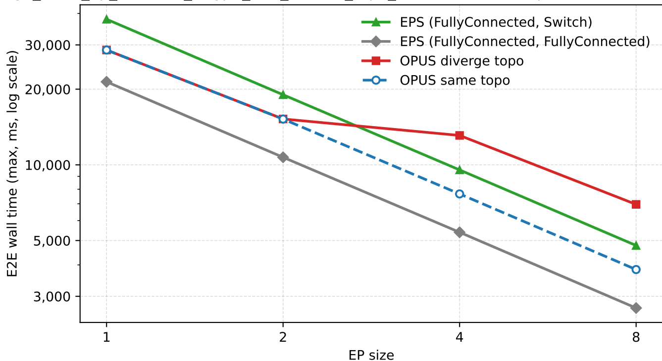
large_scale_ep_scaleout_32gpu_512_all2allv_topk_context - EP sweep at 1ms switching
