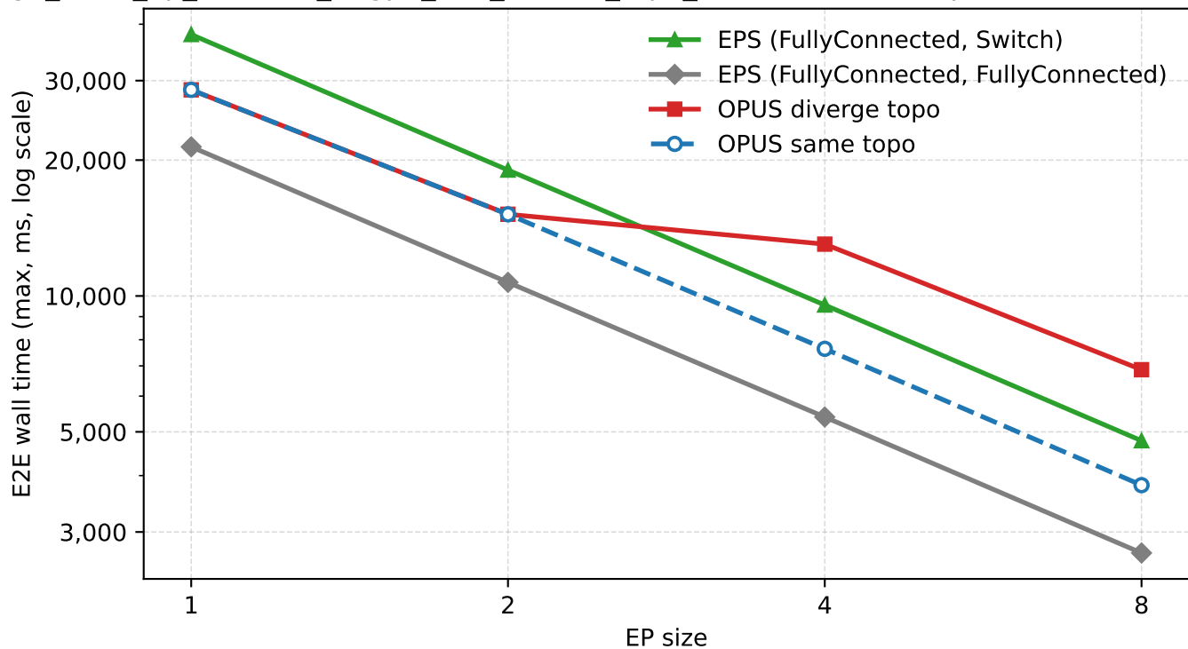
large_scale_ep_scaleout_32gpu_512_all2allv_topk_context - EP sweep at 500us switching
