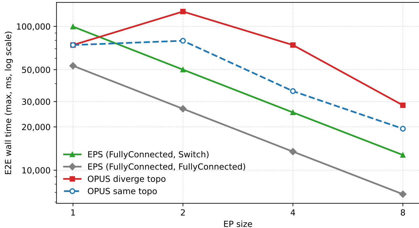
large_scale_ep_scaleout_8gpu_256_all2allv_topk_context - EP sweep at 10ms switchir
