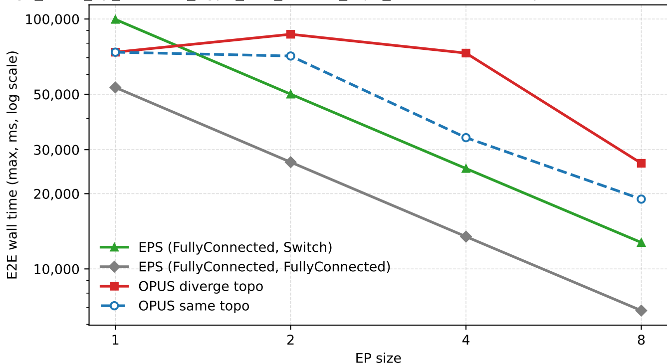
large_scale_ep_scaleout_8gpu_256_all2allv_topk_context - EP sweep at 500us switching
